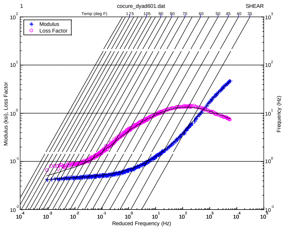
Figure 16. Nomogram for Cocured Soundcoat Dyad601
