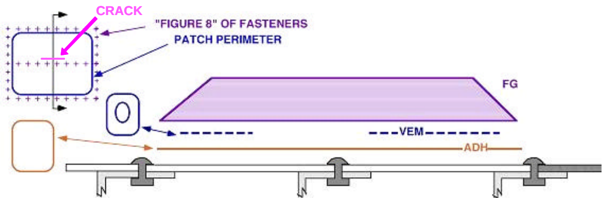
Figure 3. “Figure 8” Planform of Fasteners and Cross Section of Durability Patch
