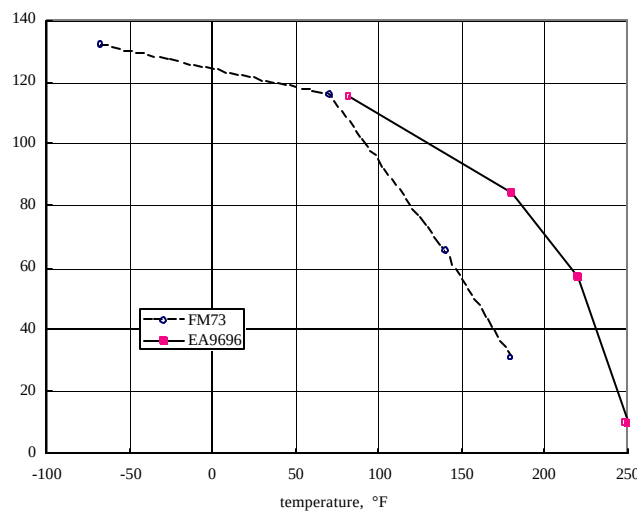
Figure 1. Shear Modulus Versus Temperature for Candidate Film Adhesives, 250°F Cure
