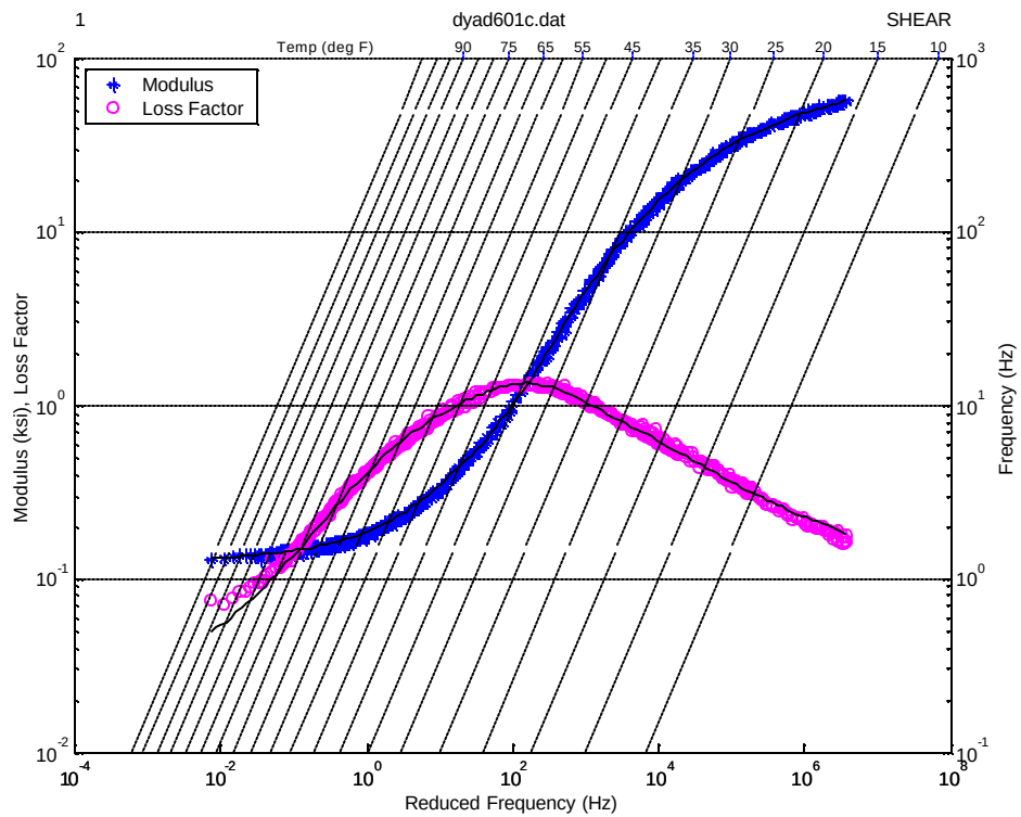
Figure 15. Nomogram for Soundcoat Dyad601
