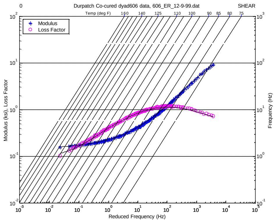
Figure 18. Nomogram for Cocured Soundcoat Dyad606
