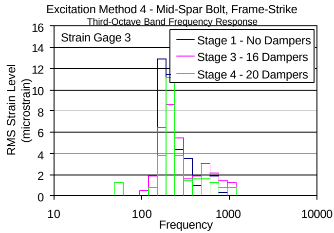
Figure 53. Comparison of Frequency Response Before and After Damper Application Using Excitation Method 4
