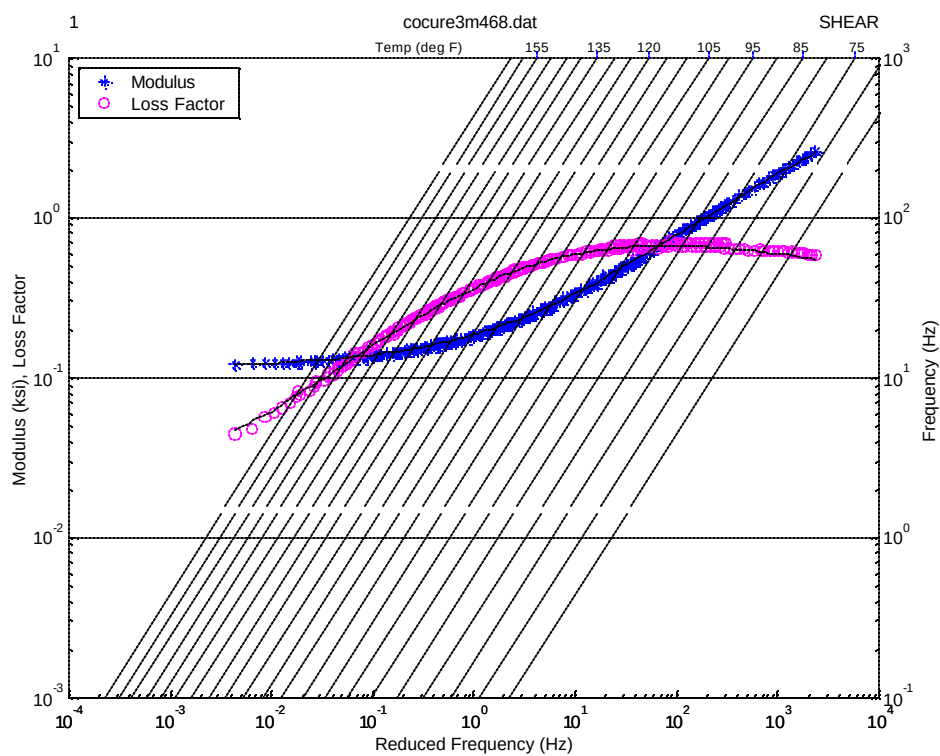
Figure 3. Nomogram for Cocured 3M 468
