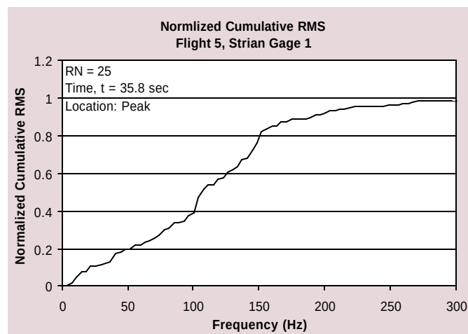
Figure 6. Sample Normalized Cumulative RMS Plot
