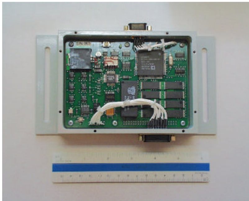
Figure 2. Damage Dosimeter
