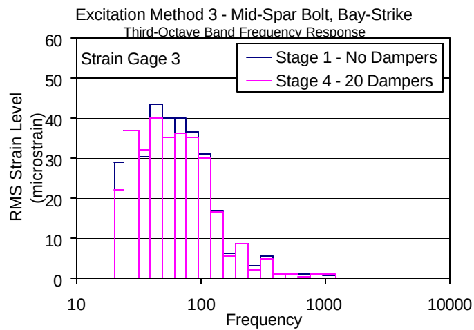
Figure 52. Comparison of Frequency Response Before and After Damper Application Using Excitation Method 3
