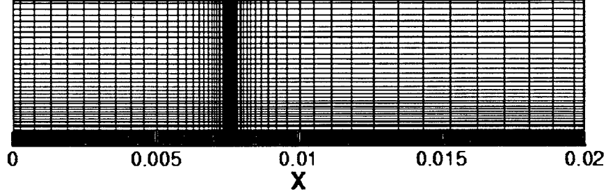
(a) 2-Dimensional, 113 × 81 grid.
