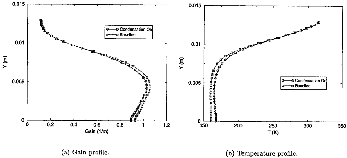
Figure 18: Gain (1/m) and temperature (K) profiles at the RADICL optical axis ( x = 0.11578m ).
