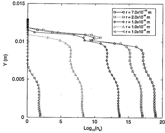
Figure 17: Water droplet number density profile, \text{Log}_{10}(n_k) , profiles at the RADICL optical axis ( x = 0.11578m ).
