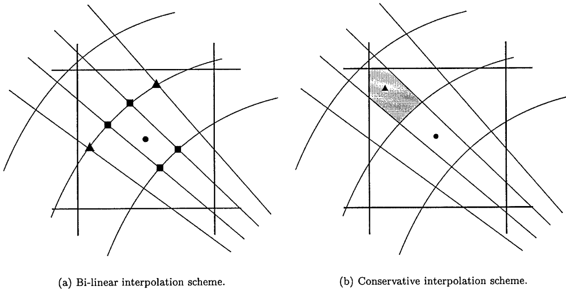
Figure 9: Schematic of mapping between flow-solver and polar optics mesh.
