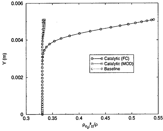
(a) O_2(^3\Sigma) mass fractions.
