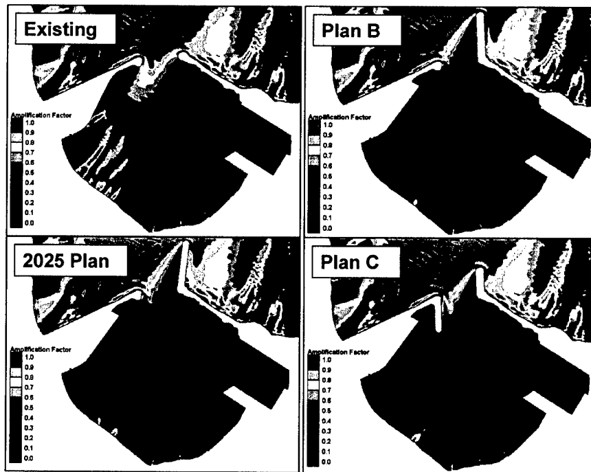
Figure 40. Wave height amplification factor, storm event of 13 Mar. 1994
