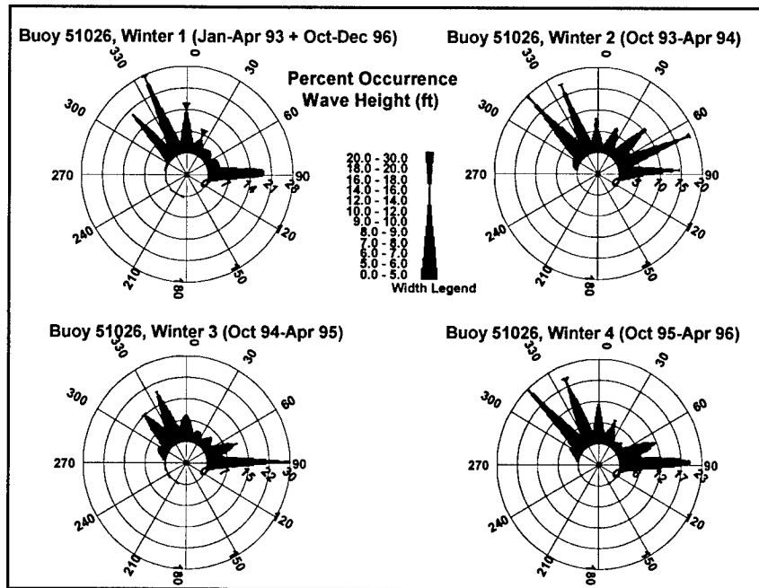
Figure 10. Wave height roses, winter, NDBC buoy 51026
