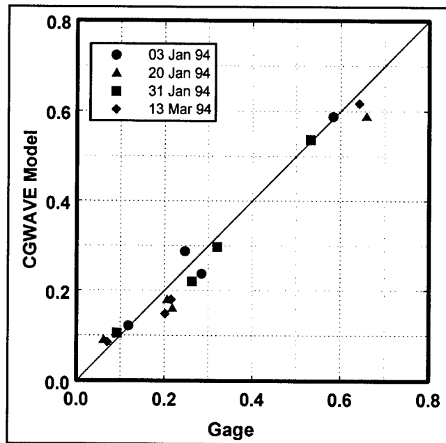
Figure 34. Model short wave calibration to four storm events, amplification factors
