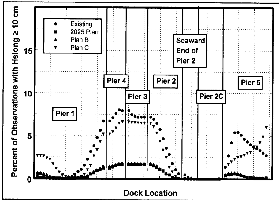
Figure 56. Percent occurrence of H_{s,long} \geq 10 cm at piers, T = 100\text{--}400 sec
