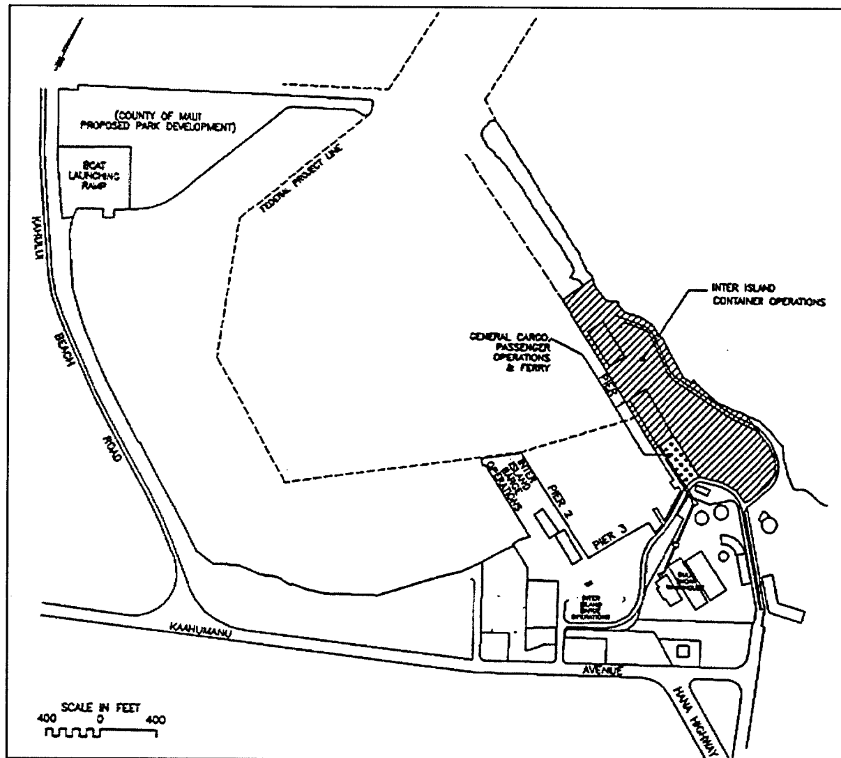
Figure 4. Kahului Harbor, existing plan
