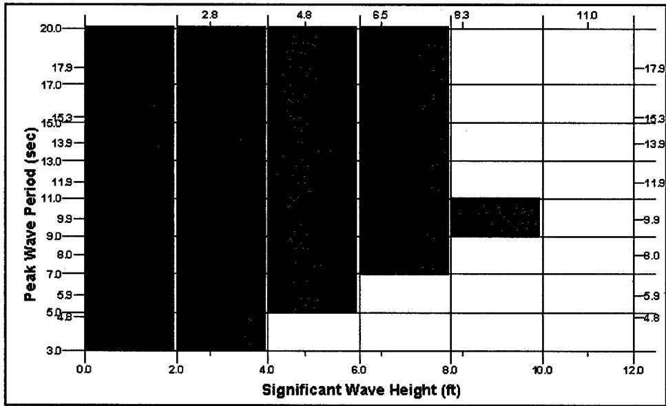
Figure 23. Percent occurrence, peak wave period vs. significant height, Kahului array, 1994
