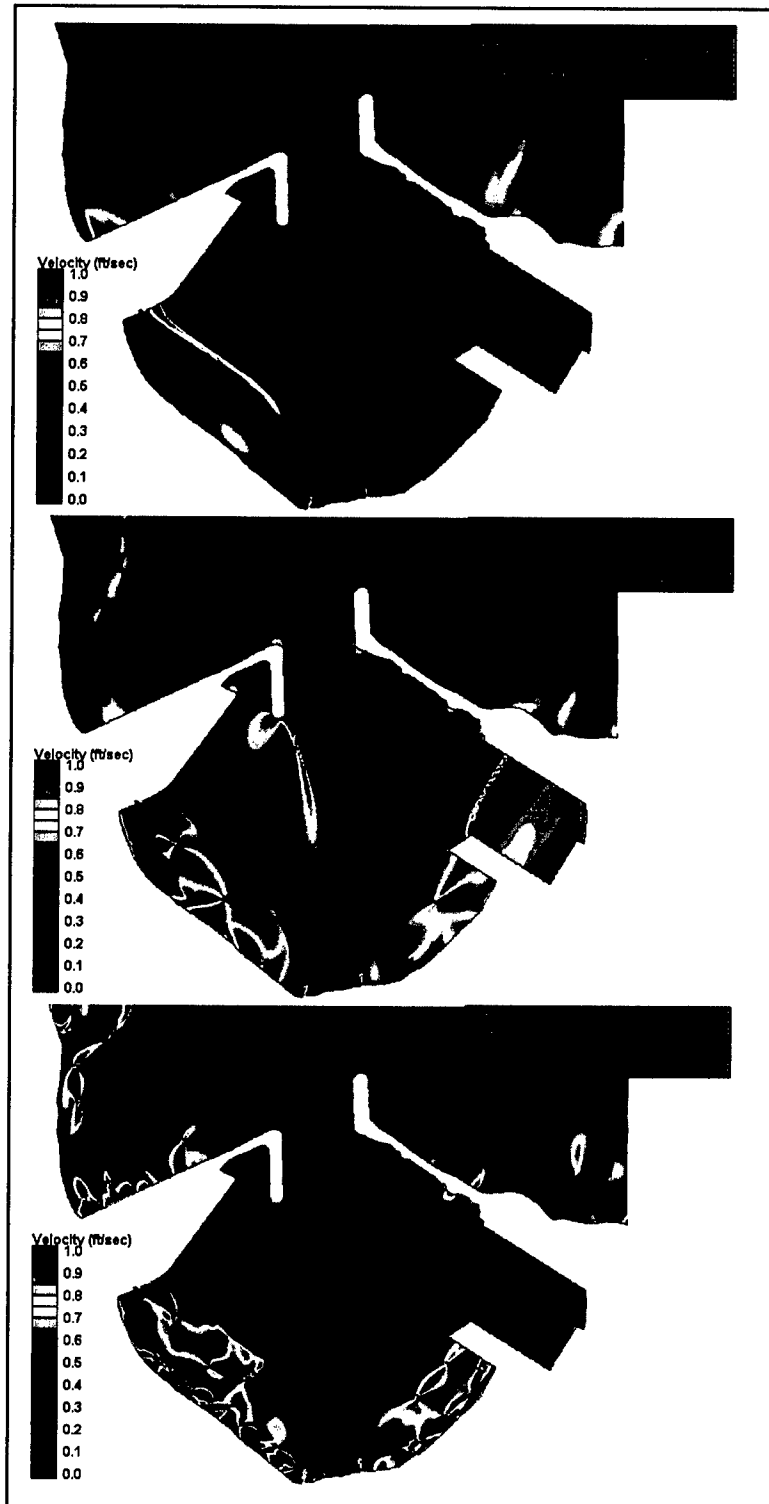
Figure 60. Resonant long wave velocity contours, Plan C
