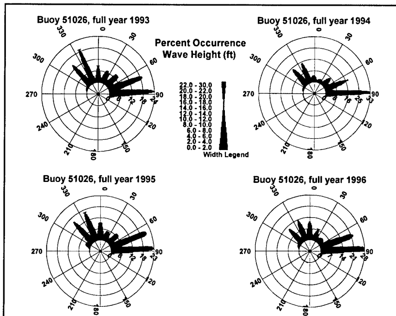
Figure 8. Wave height roses, annual, NDBC buoy 51026
