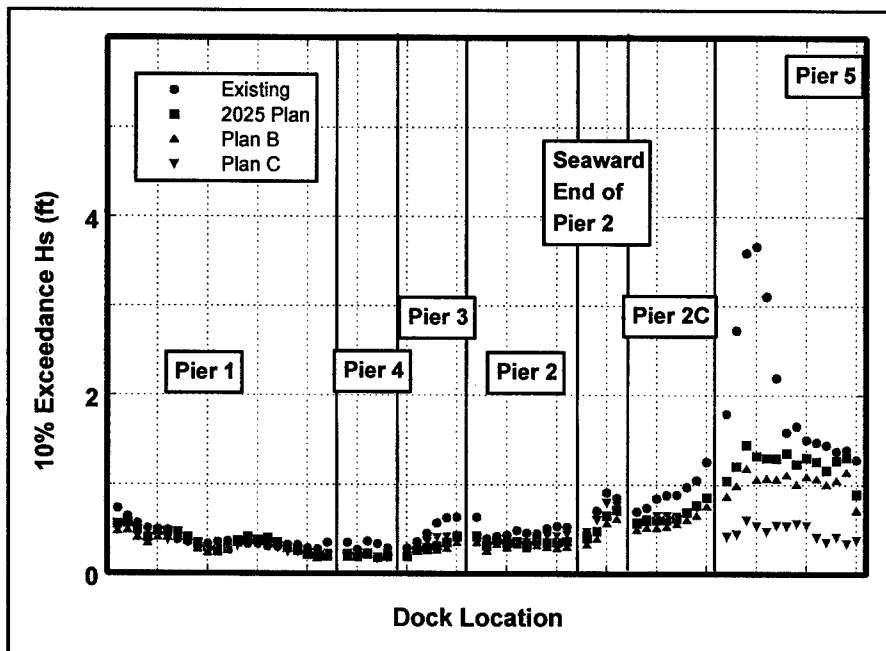
Figure 43. Comparison of H_s exceeded 10 percent of time at piers
