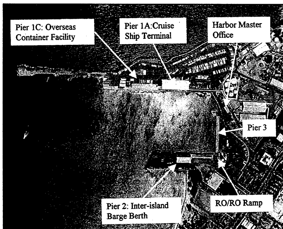
Figure 3. Kahului Harbor aerial photo, commercial piers (State of Hawaii 2000)
