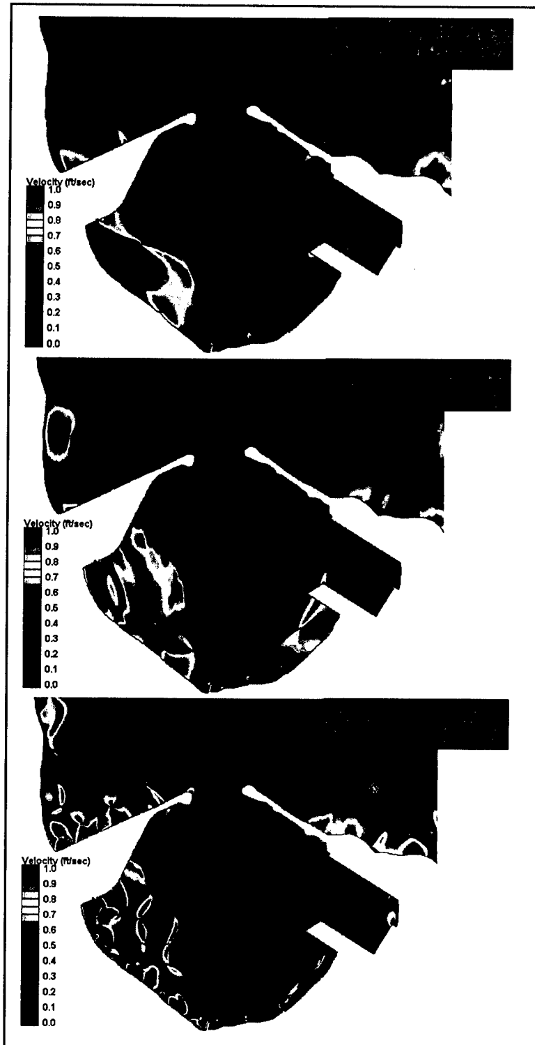
Figure 58. Resonant long wave velocity contours, existing harbor
