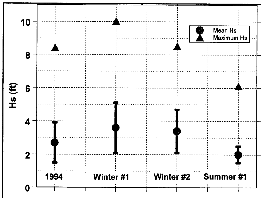
Figure 19. Wave height statistics, Kahului array
