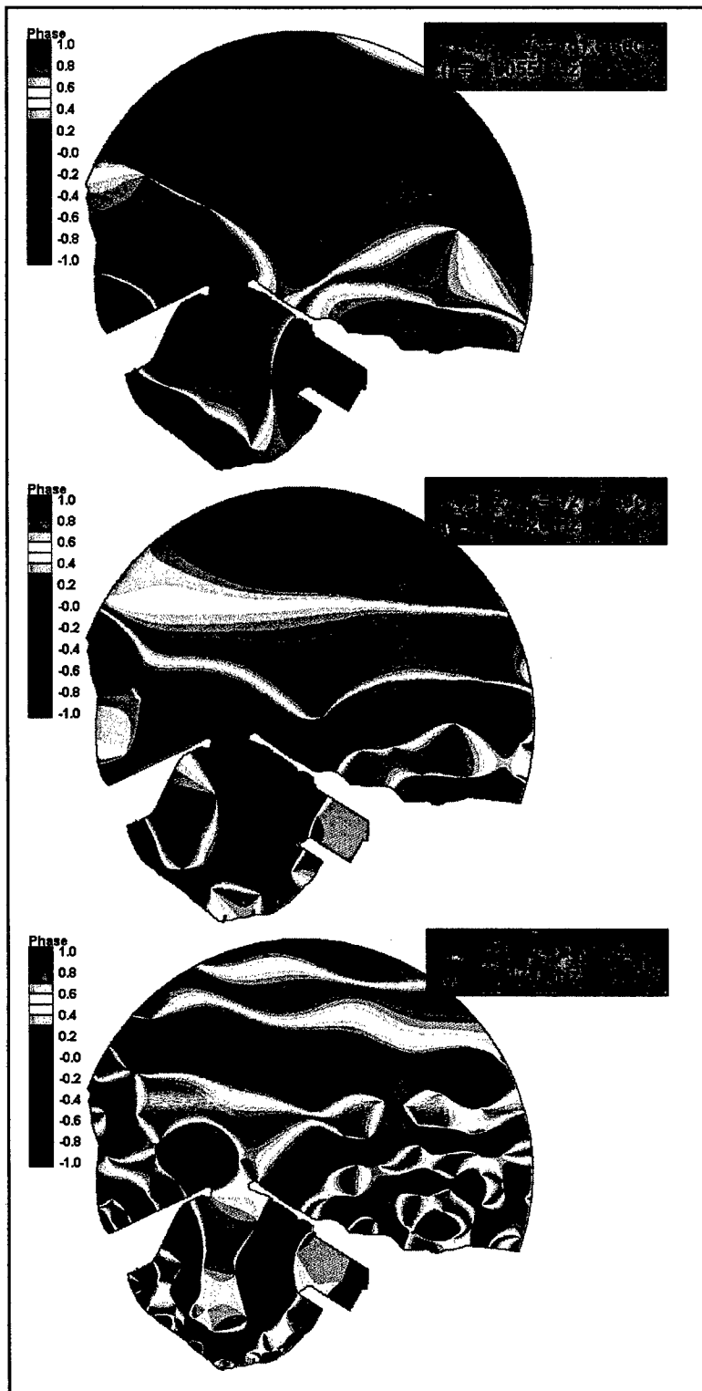
Figure 48. Resonant long wave phase contours, existing harbor
