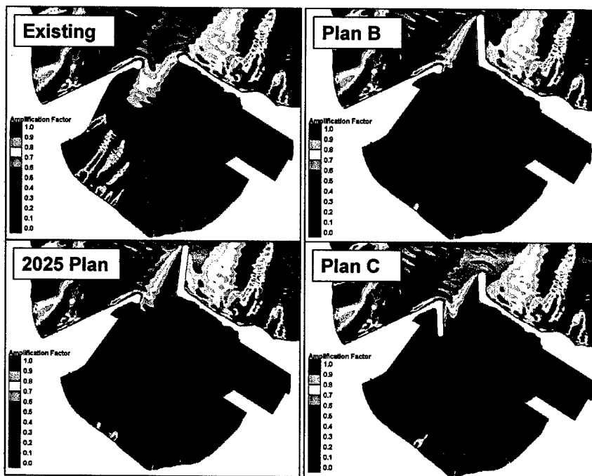
Figure 38. Wave height amplification factor, storm event of 20 Jan. 1994
