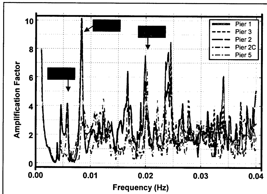
Figure 53. Long wave response, Plan C
