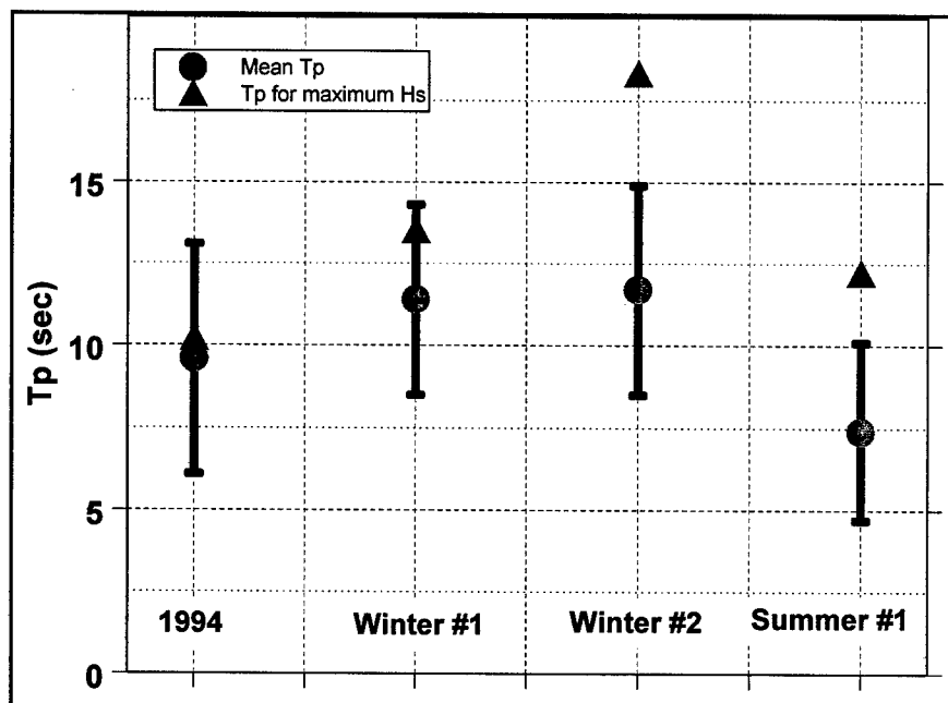
Figure 20. Wave period statistics, Kahului array
