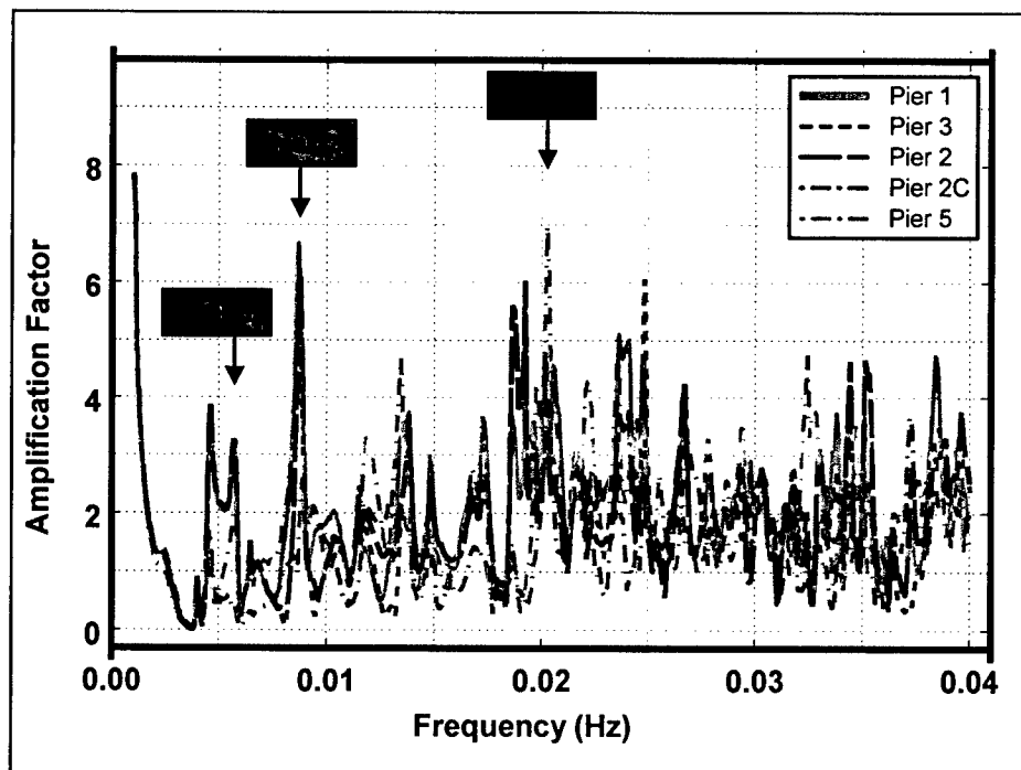
Figure 49. Long wave response, 2025 plan
