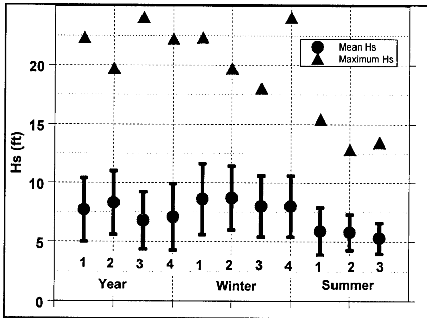
Figure 14. Wave height statistics, NDBC buoy 51026
