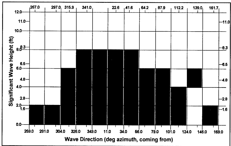
Figure 21. Percent occurrence, significant wave height vs. direction, Kahului array, 1994
