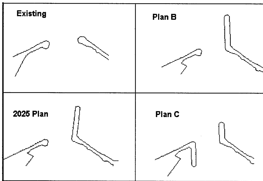
Figure 6. Kahului Harbor entrance plans for modeling
