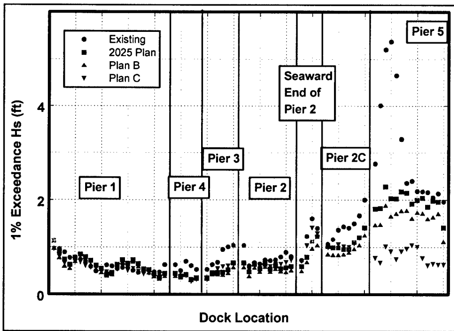
Figure 44. Comparison of H_s exceeded 1 percent of time at piers
