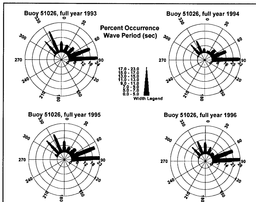
Figure 9. Wave period roses, annual, NDBC buoy 51026
