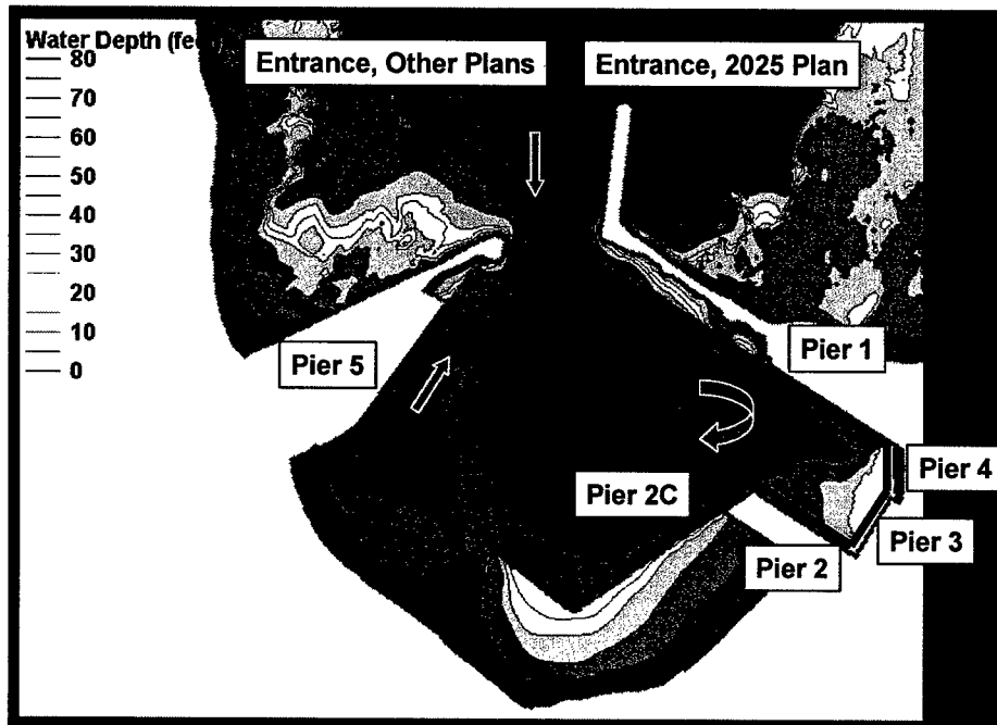
Figure 36. Model output lines
