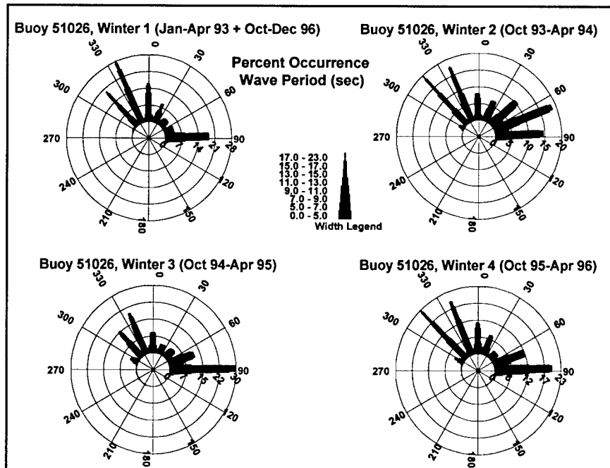
Figure 11. Wave period roses, winter, NDBC buoy 51026
