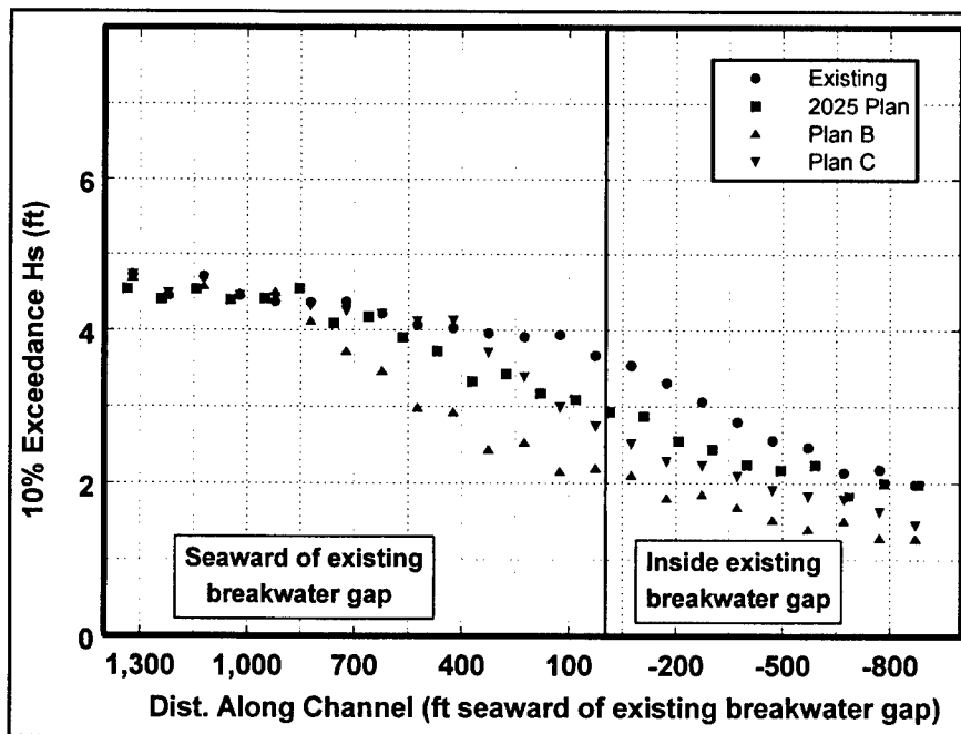
Figure 41. Comparison of H_s exceeded 10 percent of time in entrance channel
