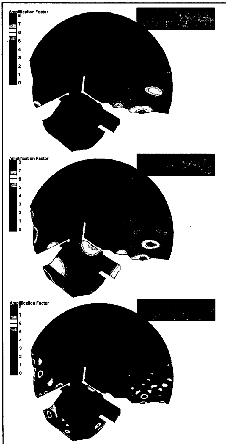
Figure 50. Resonant long wave amplification factor contours, 2025 plan
