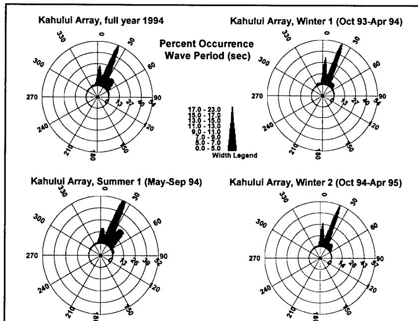
Figure 18. Wave period roses, Kahului array
