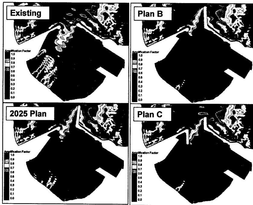
Figure 37. Wave height amplification factor, storm event of 3 Jan. 1994
