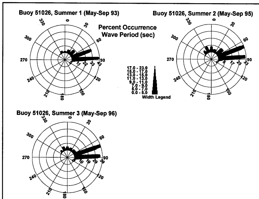
Figure 13. Wave period roses, summer, NDBC buoy 51026
