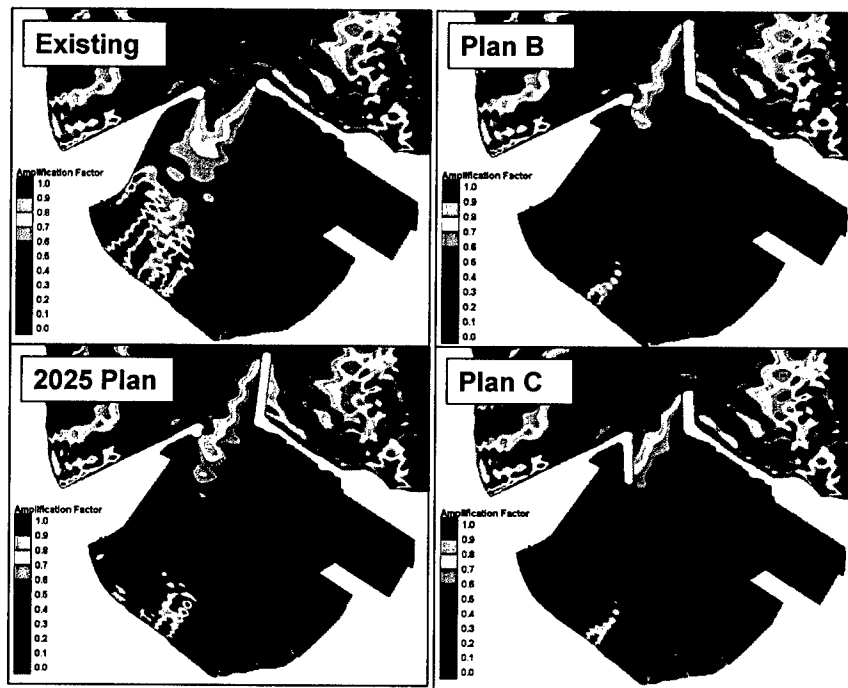
Figure 39. Wave height amplification factor, storm event of 31 Jan. 1994
