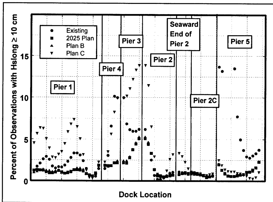
Figure 57. Percent occurrence of H_{s,long} \geq 10 cm at piers, T = 30\text{--}100 sec
