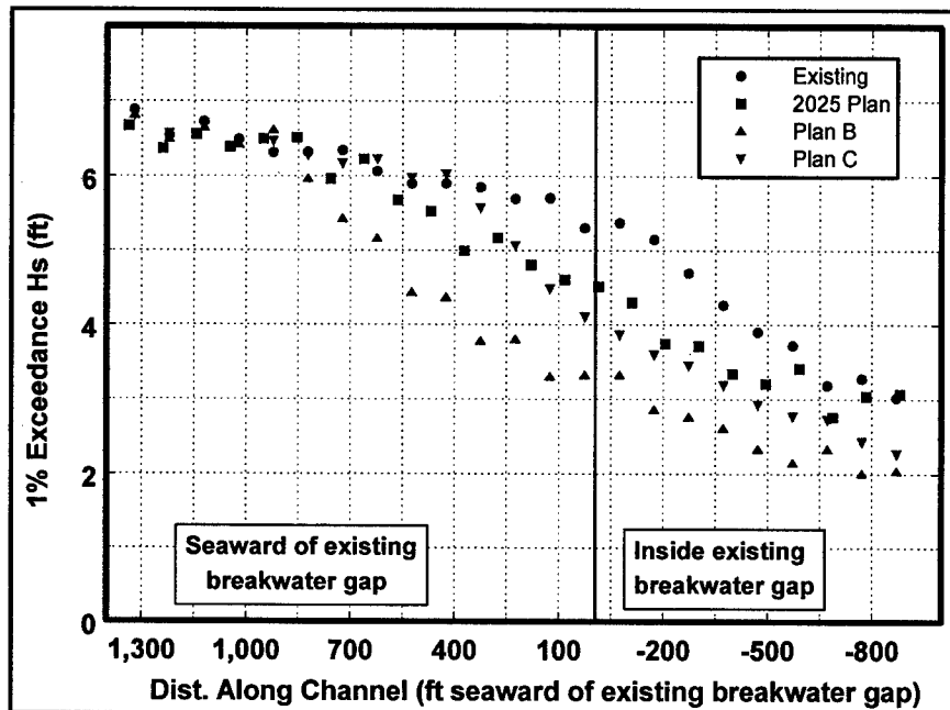
Figure 42. Comparison of H_s exceeded 1 percent of time in entrance channel
