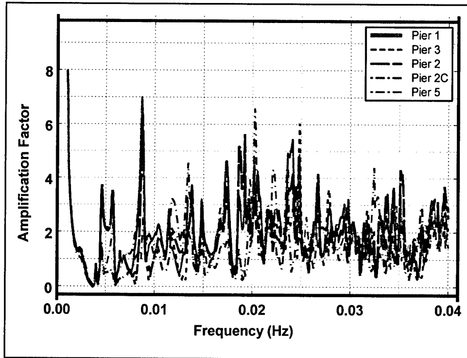
Figure 52. Long wave response, Plan B
