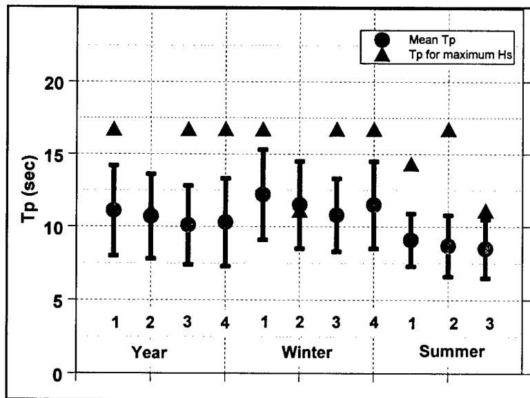
Figure 15. Wave period statistics, NDBC buoy 51026
