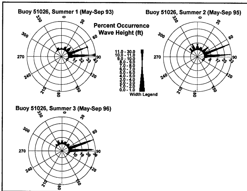
Figure 12. Wave height roses, summer, NDBC buoy 51026
