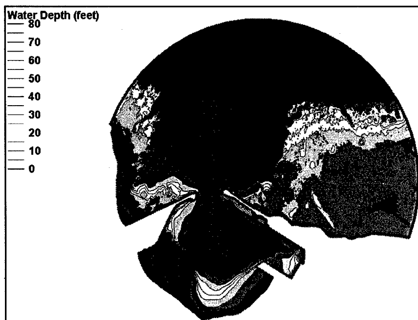
Figure 28. Model bathymetry, existing harbor
