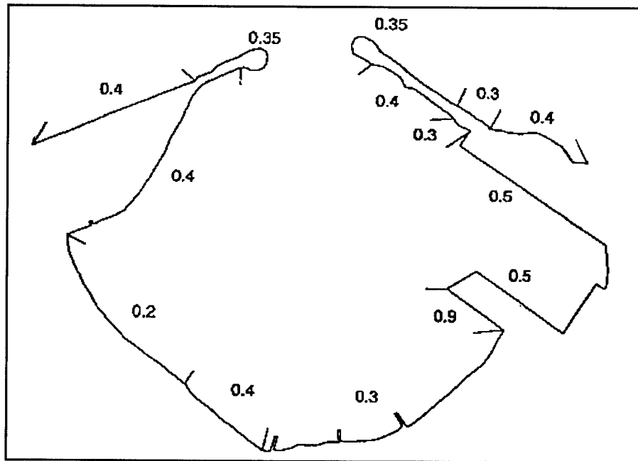
Figure 29. Model wave reflection coefficients, short waves, existing harbor
