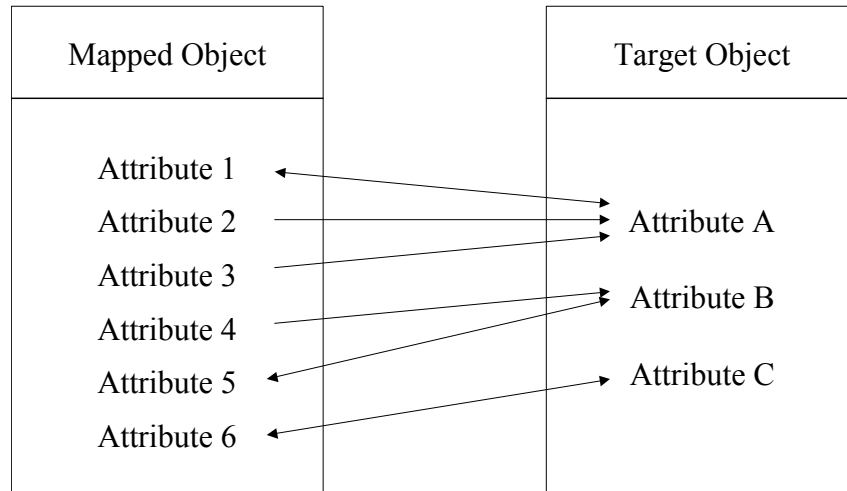
Figure 32 Imperfect Object Match with Two-Way Mapping
