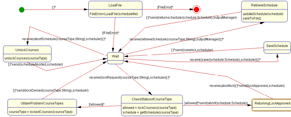
Figure 43 ManageSchedules Task Diagram
