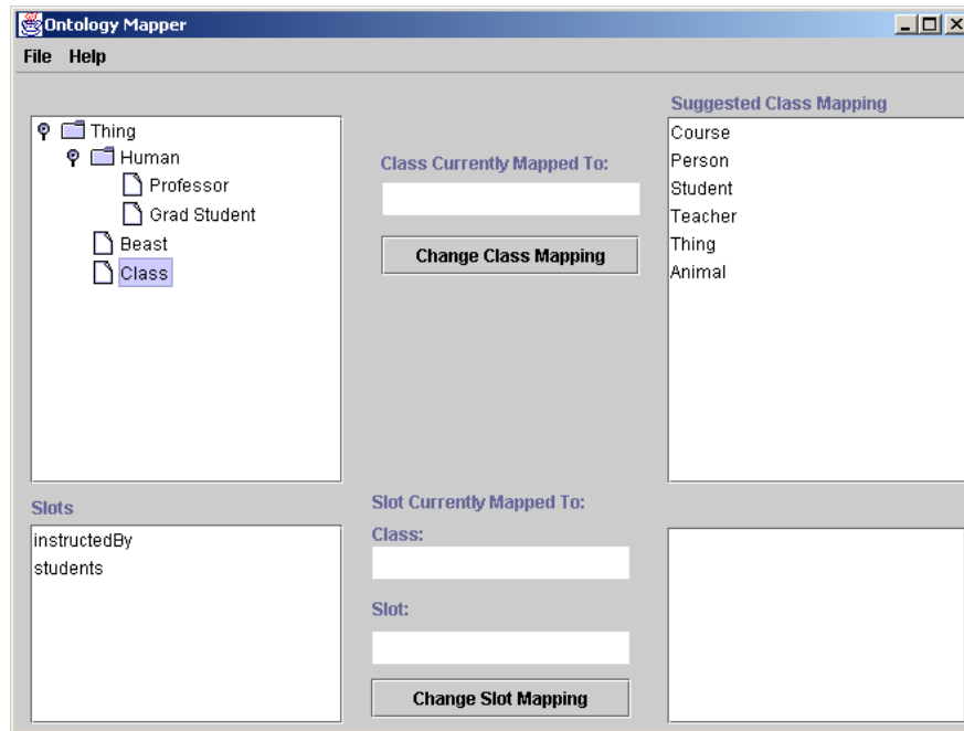
Figure 29 Ontology Mapper
