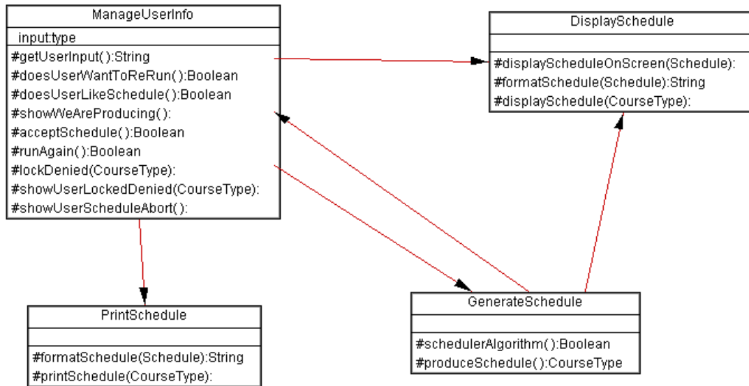
Figure 28 Example Agent Architecture Diagram
