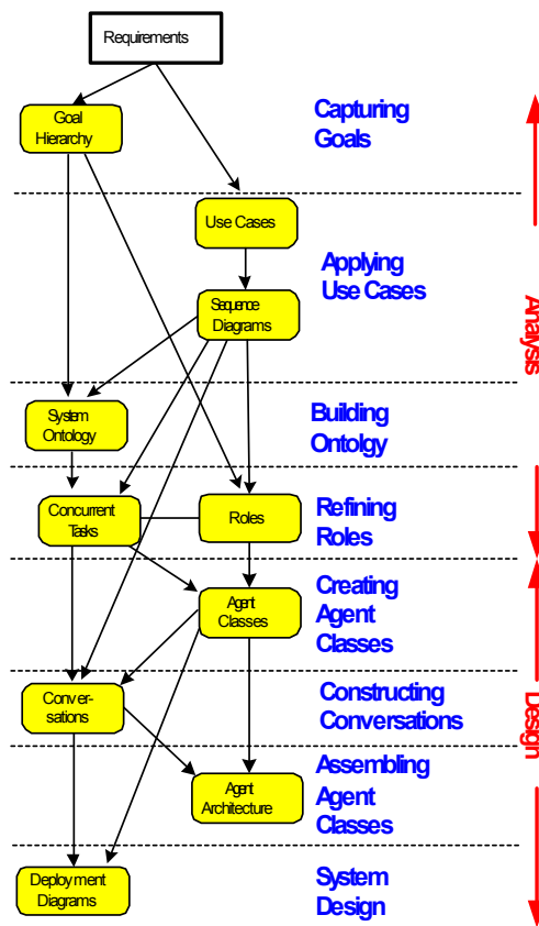
Figure 15 Extended MaSE Methodology
