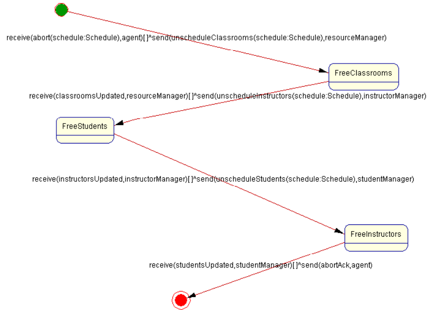
Figure 44 FreeScheduleResources Task Diagram
