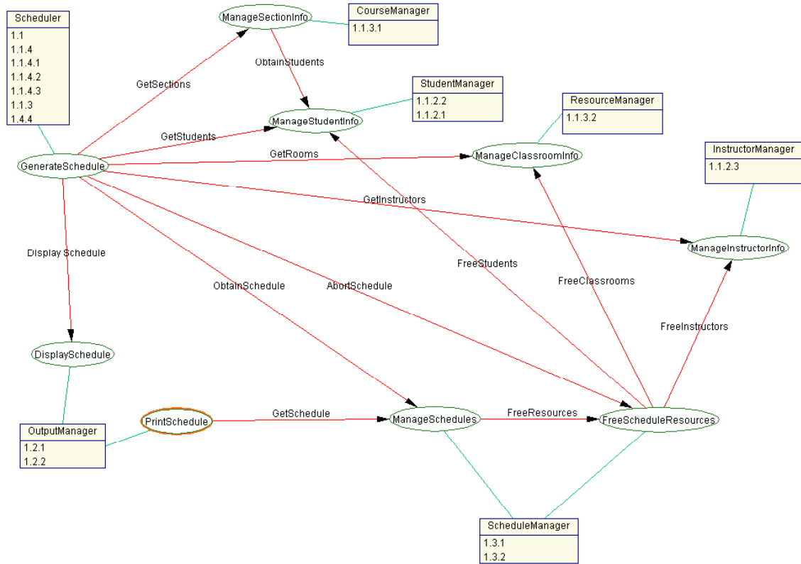
Figure 23 Example Role Diagram
