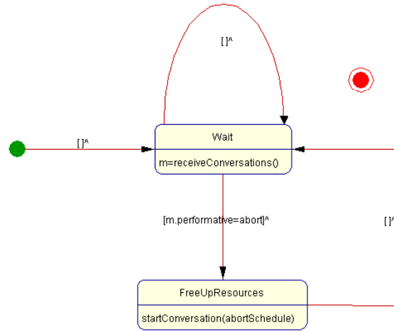
Figure 47 FreeScheduleResources Component State Diagram
