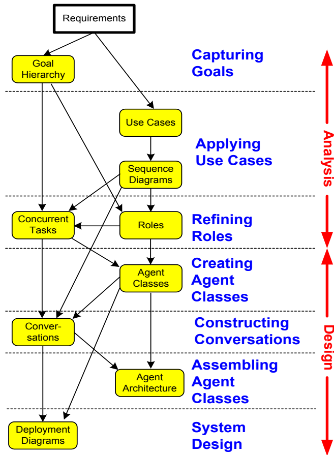
Figure 3 MaSE Phases, Steps and Models
