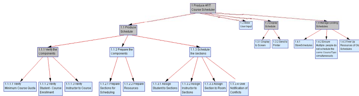
Figure 37 Distributed Course Scheduling Goal Hierarchy
