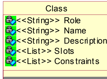
Figure 13 Structure of a Class in an Ontology
