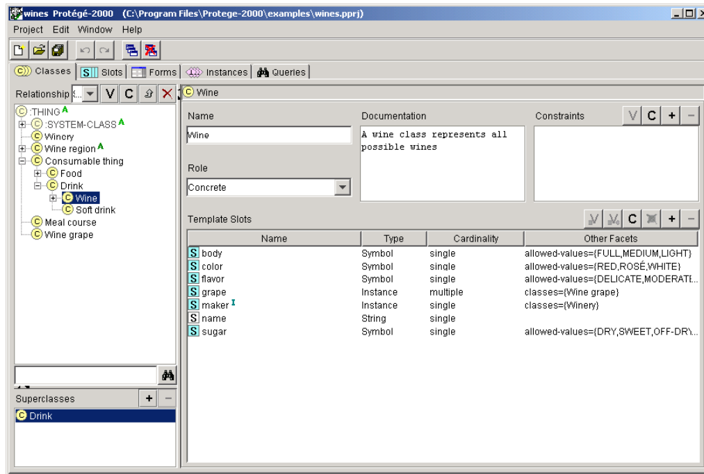
Figure 2 Protégé 2000 Main User Interface
