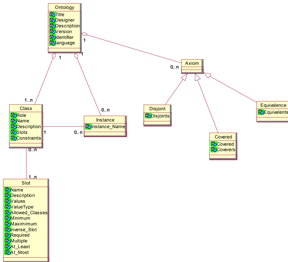
Figure 12 Structure of an Ontology
