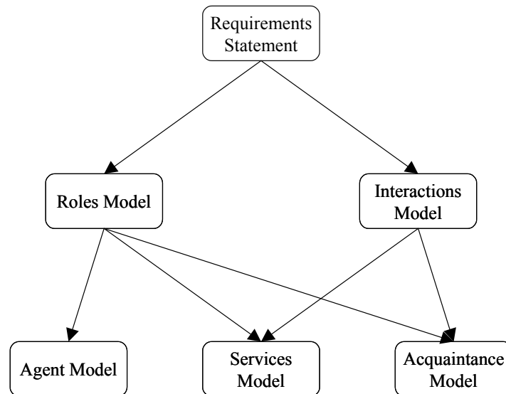
Figure 9 Relationships Between Gaia Models
