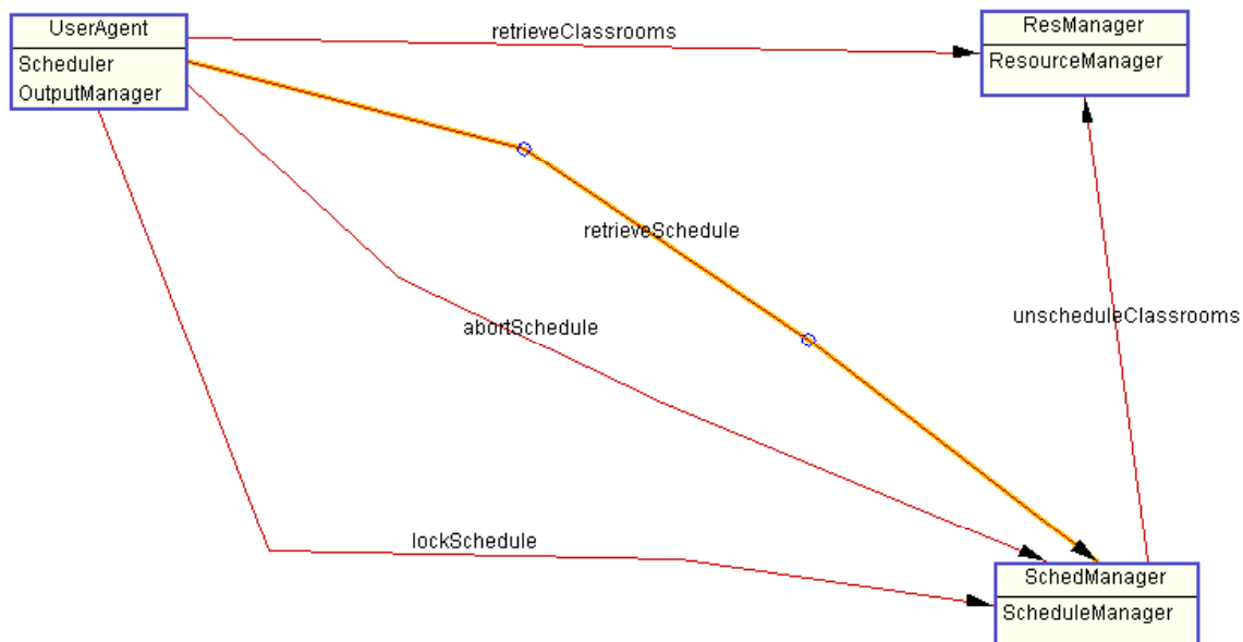
Figure 25 Example Agent Class Diagram
