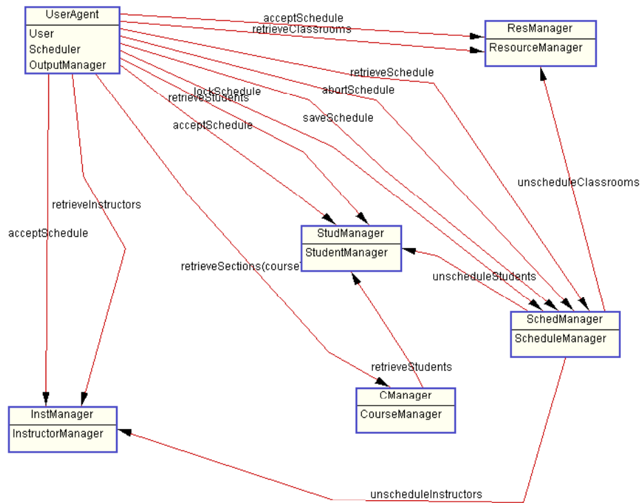
Figure 45 Agent Template Diagram
