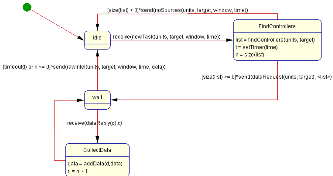
Figure 6 Example Concurrent Task Diagram [DeLoach and Wood 2000b]
