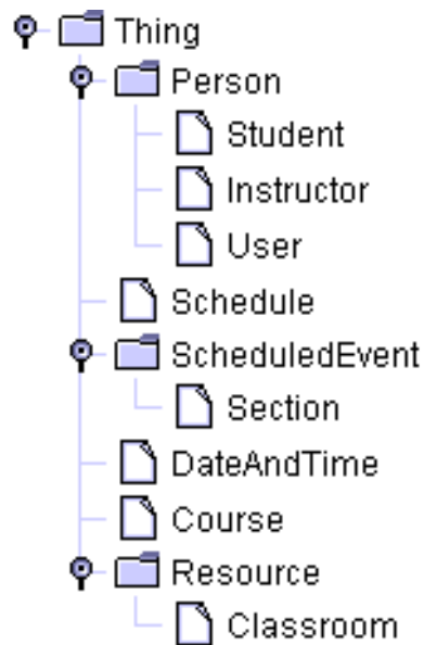
Figure 40 Final Class Hierarchy for the Registrar Ontology
