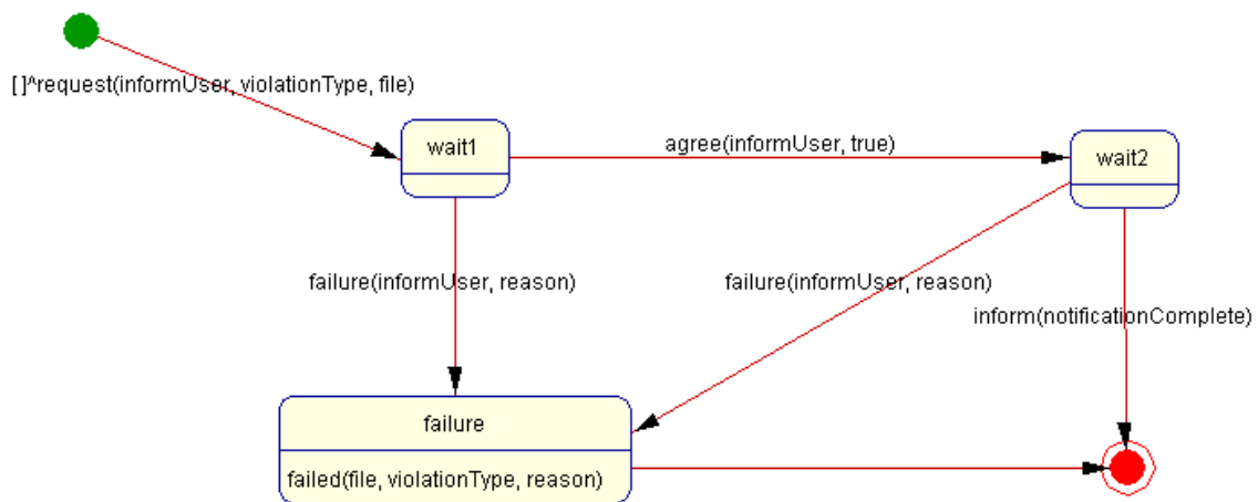
Figure 8 Example Conversation Diagram [DeLoach 2001]
