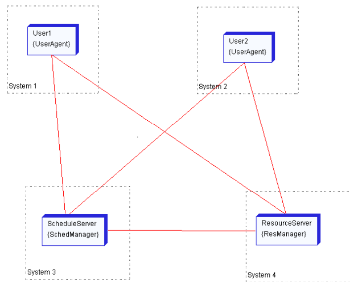
Figure 30 Example Deployment Diagram
