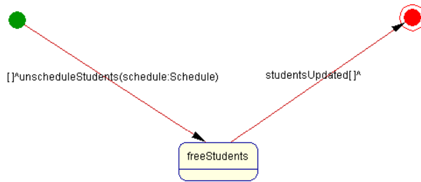
Figure 34 Sample Finite State Automata with Information Passing
