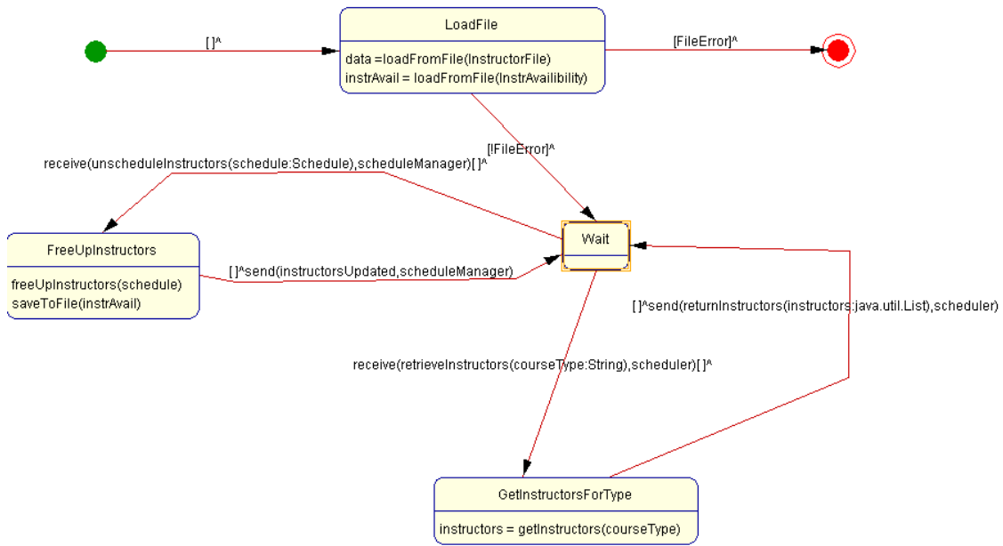
Figure 35 Task Diagram with Unspecified Variable
