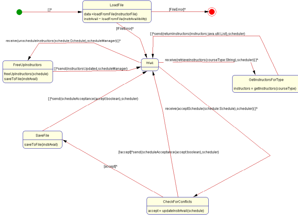
Figure 42 ManageInstructorInfo Task
