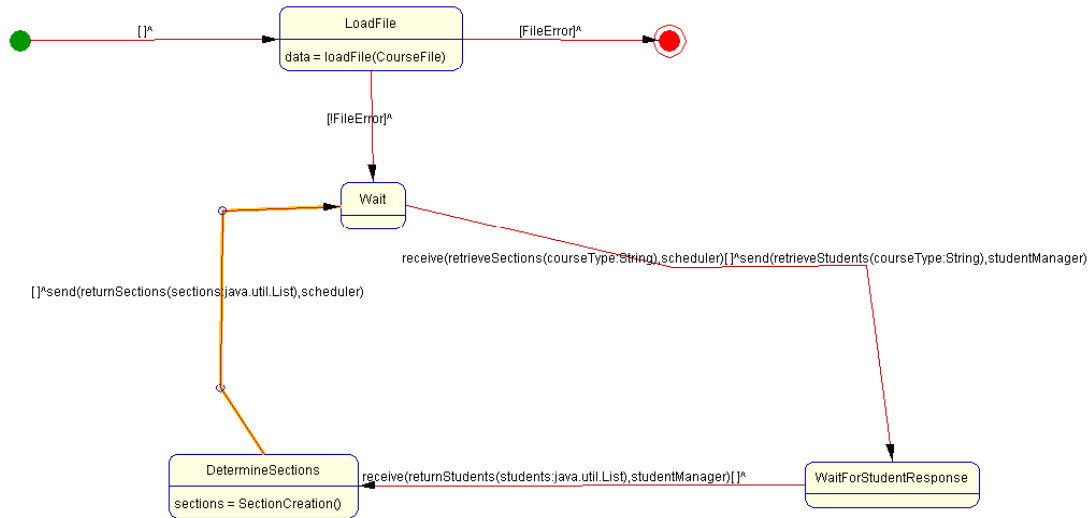
Figure 41 ManageSectionInfo Task
