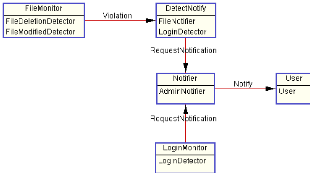
Figure 7 Example Agent Class Diagram [DeLoach 2001]
