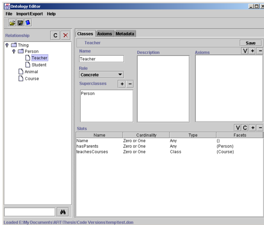
Figure 19 Main Window of Ontology Editor
