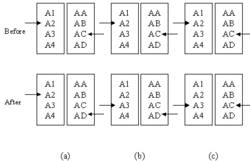
Figure 33 Possible Situations When Comparing Attributes With an Ordering
