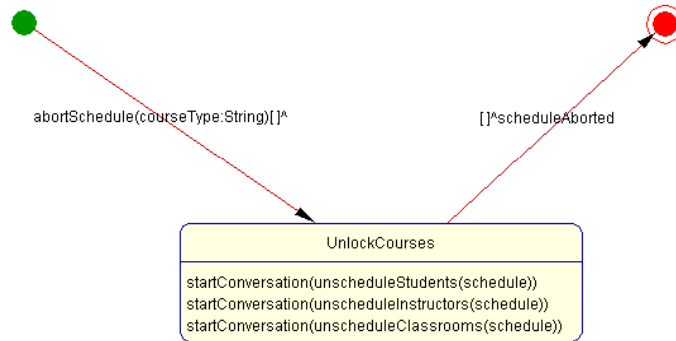
Figure 46 abortSchedule Conversation Responder Diagram
