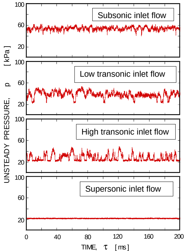
FIGURE 5.2.3 Oscillating Cascade Rig Test Results
