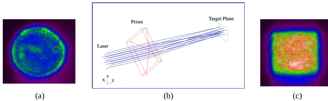
FIGURE 1.5.2.2 Spatial Profiles of the Laser Beam Showing the Transformation from a Round Spot (a) to a Square Spot (c) with the Use of Optics (b)
