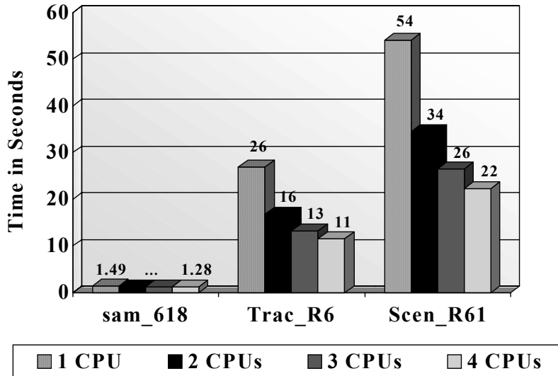
Figure 20 – Performance Scalability
