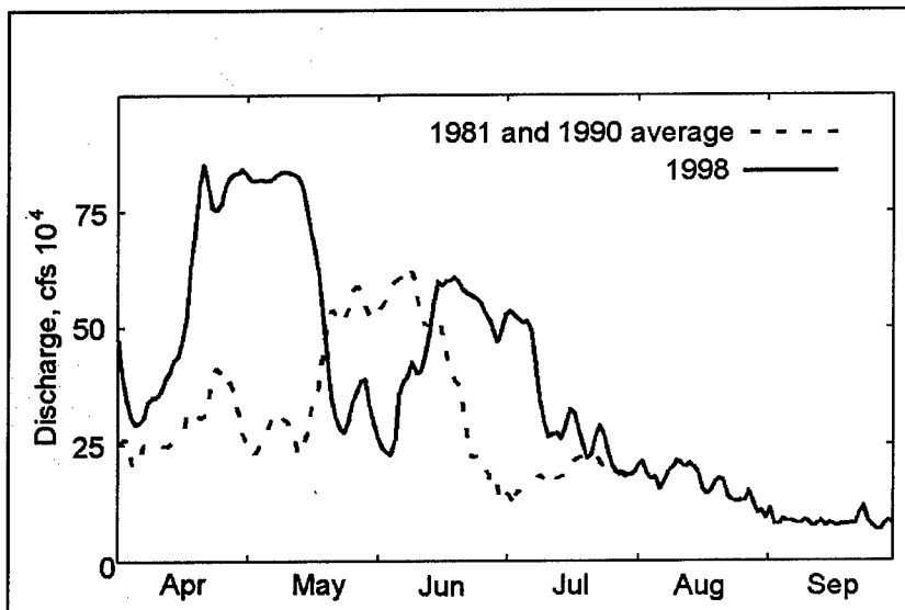
Figure 24. Discharge of the lower Ohio River at Metropolis, IL, averaged for 1981 and 1990 and compared to 1998
