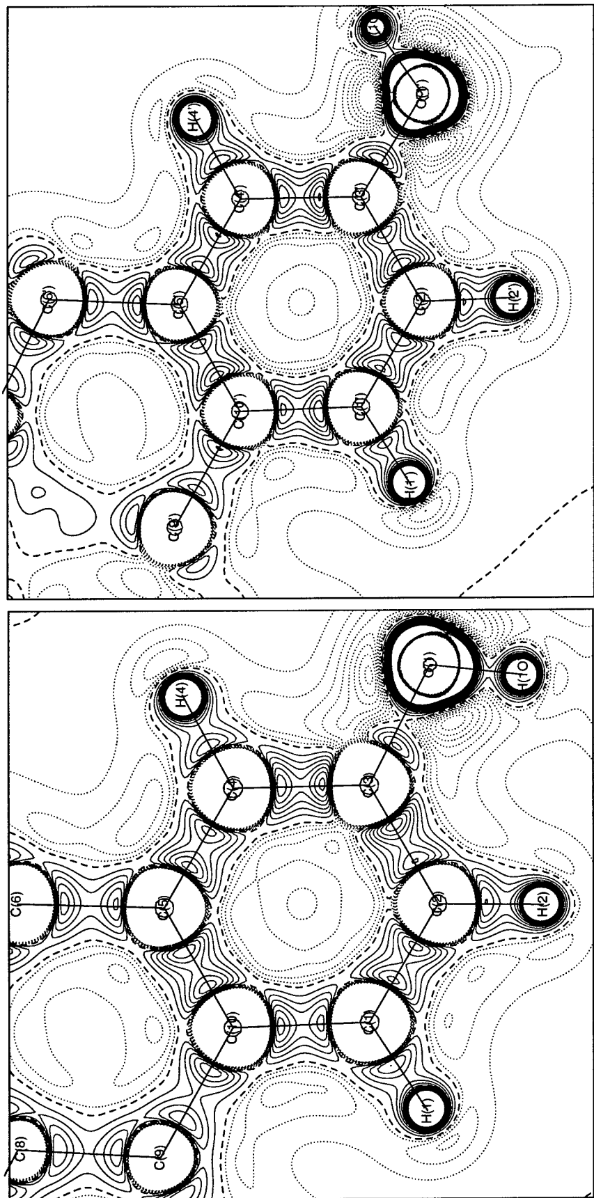
Figure C-10. The Laplacian of the total electron density of atoms at rest in the plane of the aromatic rings of 17 \beta -estradiol in methanol. Contour intervals are 5 eÅ -5 starting at 5 eÅ -5 (solid blue lines), -2 eÅ -5 (dotted red lines), and the dashed line plots 0 eÅ -5 .
