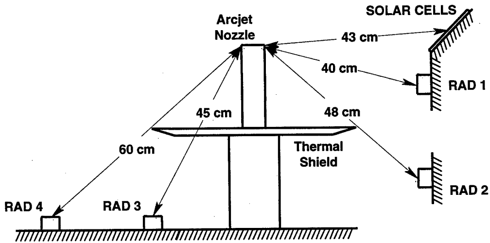
Fig. 5 Positions of the 4 Radiometers and the Solar Cell segment in relation to the arcjet nozzle.
