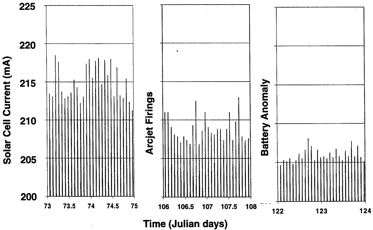
Fig. 16 Solar Cell current at selected times during the ESEX flight
