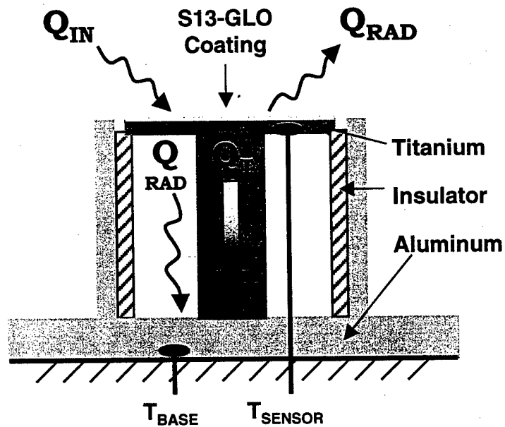
Fig. 6 Schematic diagram of the ESEX radiometer sensors to measure heat flux and material degradation of the S13-GLO thermal coating. The radiometer base is 2.9" in diameter.
