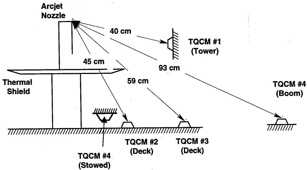
Fig. 3 TQCM Locations relative to the arcjet nozzle. TQCM 4 is in the deployed position for all of the arcjet firings.
