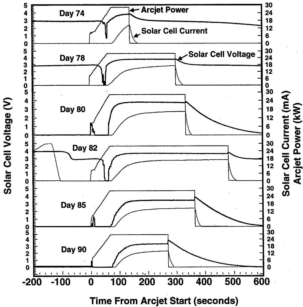
Fig. 14 Solar Cell response to the 6 primary ESEX firings
