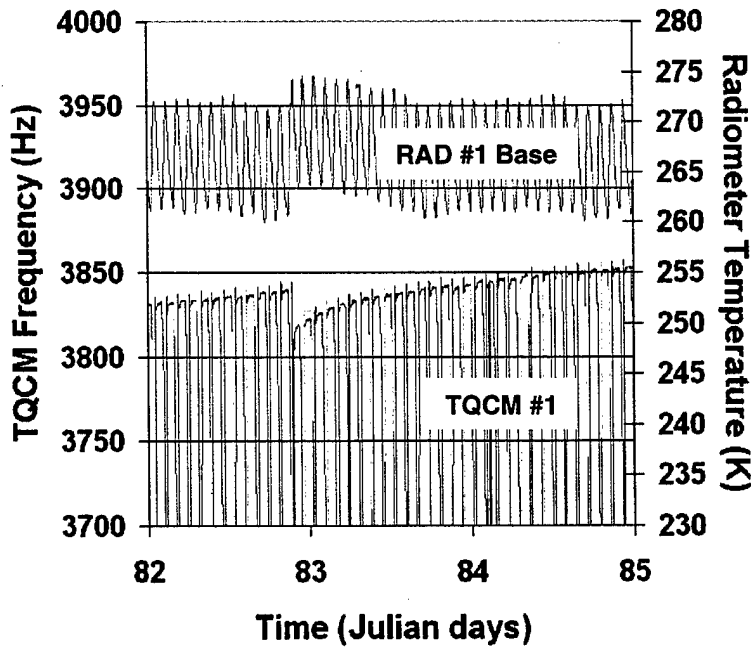
Fig. 8 TQCM#1 response to Firing #4 shown with a longer time base. Also shown is the local spacecraft temperature measured at the base of the adjacent radiometer #1.
