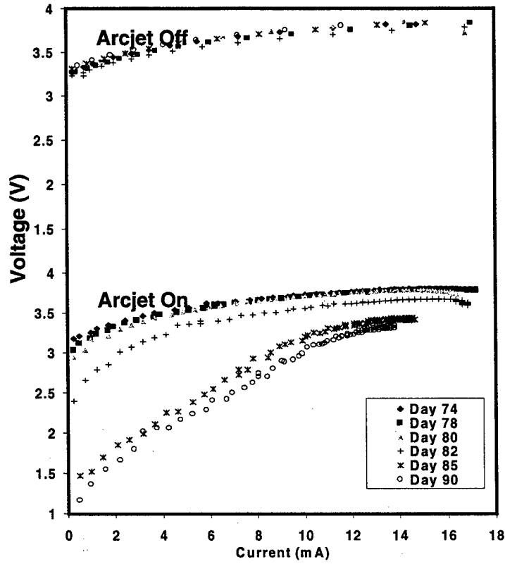
Fig. 15 Solar Cell IV curves during the ESEX firings
