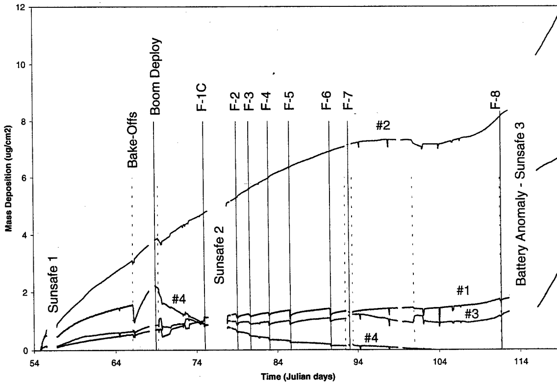
Fig. 10 TQCM behavior from launch through the battery anomaly.
