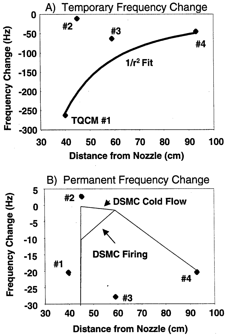
Fig. 17 TQCM frequency changes during arcjet firings. A) Shows the Temporary changes, and B) shows the Permanent changes
