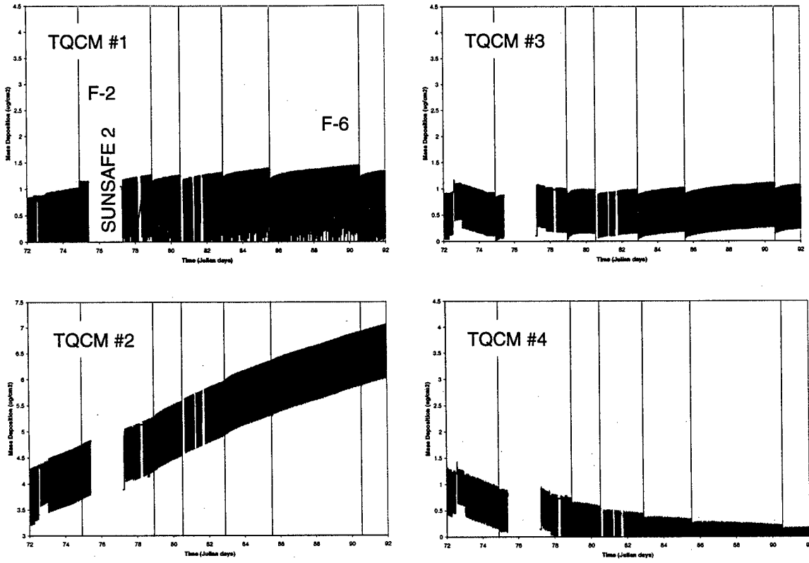
Fig. 9 Mass deposition measured on each of the 4 TQCMs through the primary 6 ESEX firings.
