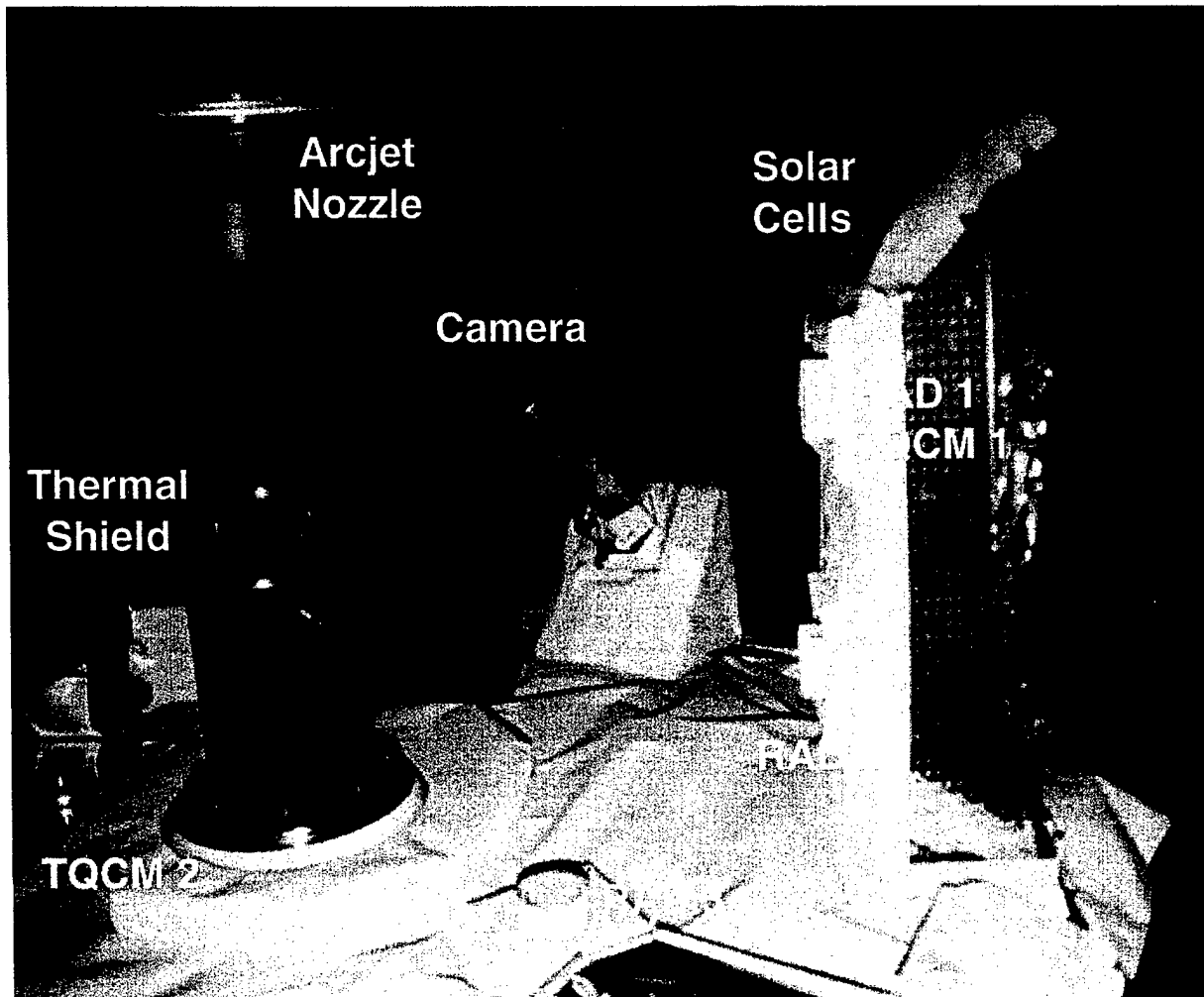
Fig. 2 Photograph of the ESEX platform in its pre-flight condition
