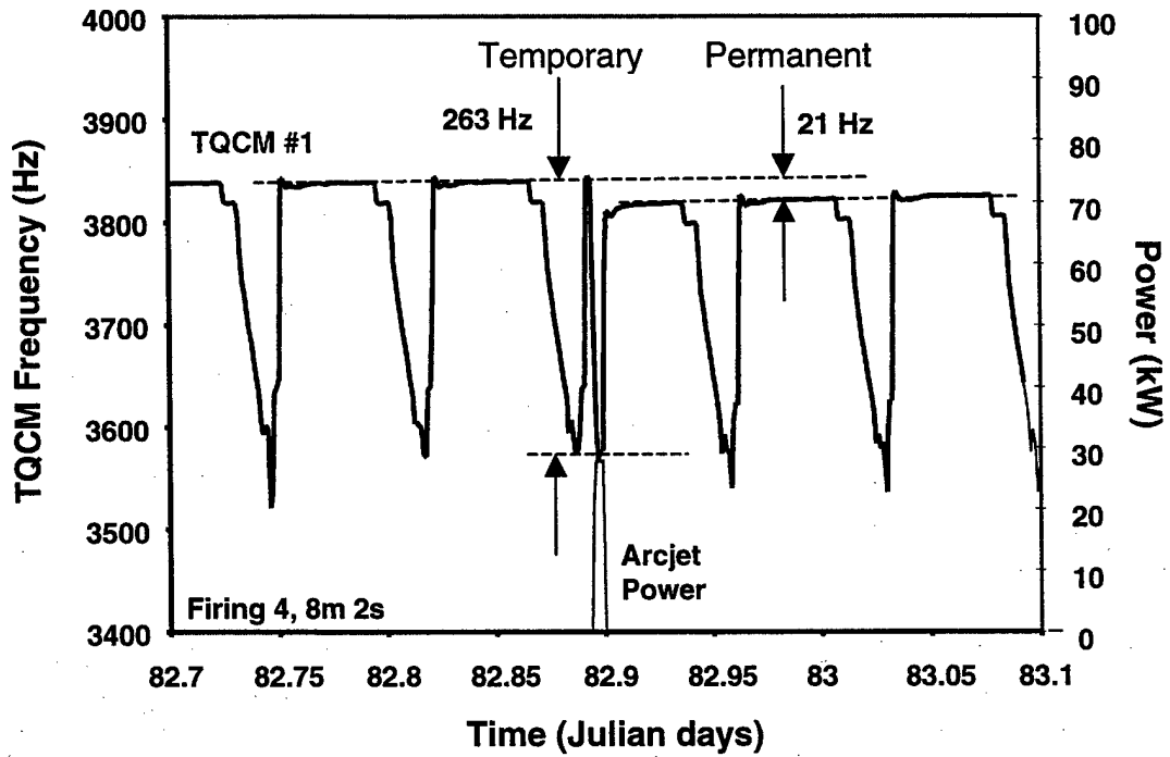
Fig. 7 Typical TQCM response to an arcjet firing. Shown is the output frequency from TQCM #1 during Firing 4.
