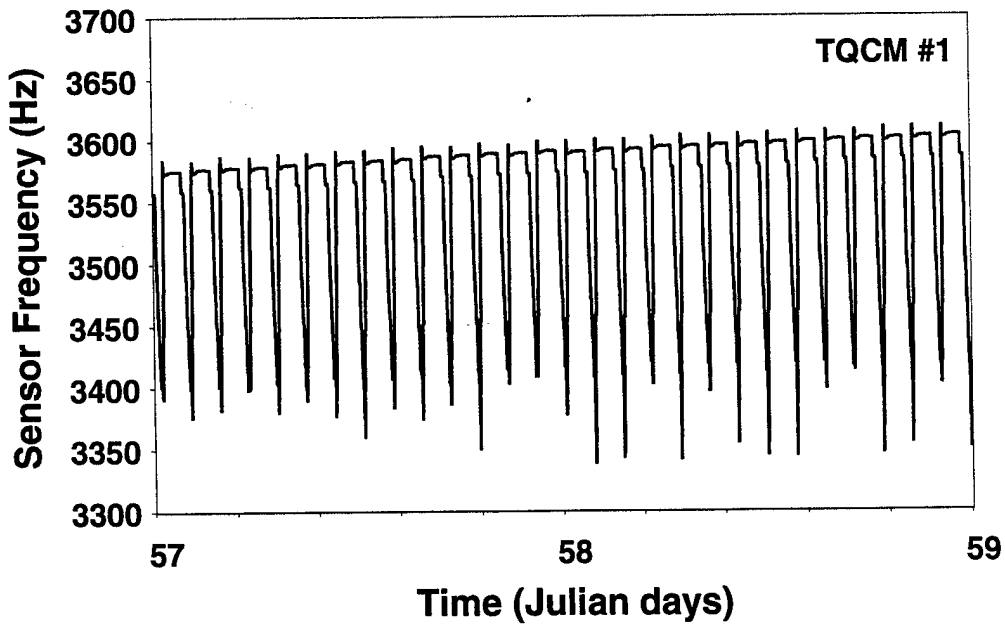
Fig. 4 Representative TQCM data showing the slow frequency increase due to mass deposition superimposed on the larger solar cycle.
