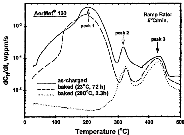
Fig. 7—The H desorption rate as a function of temperature, measured by TDS at a ramp heating rate of 5^\circ\text{C}/\text{m} , showing the effect of baking compared with the as-charged condition (charged at \eta_{\text{chg}} = -0.62 V and 60^\circ\text{C} ). At least three peaks are observed, as indicated by the arrows.
