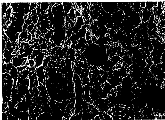
Figure 9 - SEM fractograph of the NaCl fracture surface of annealed Ti-6-4 (ELI, LT) plate loaded at a slow dK/dt of 2.0 \times 10^4 \text{ MPa}\sqrt{\text{m/s}} .
