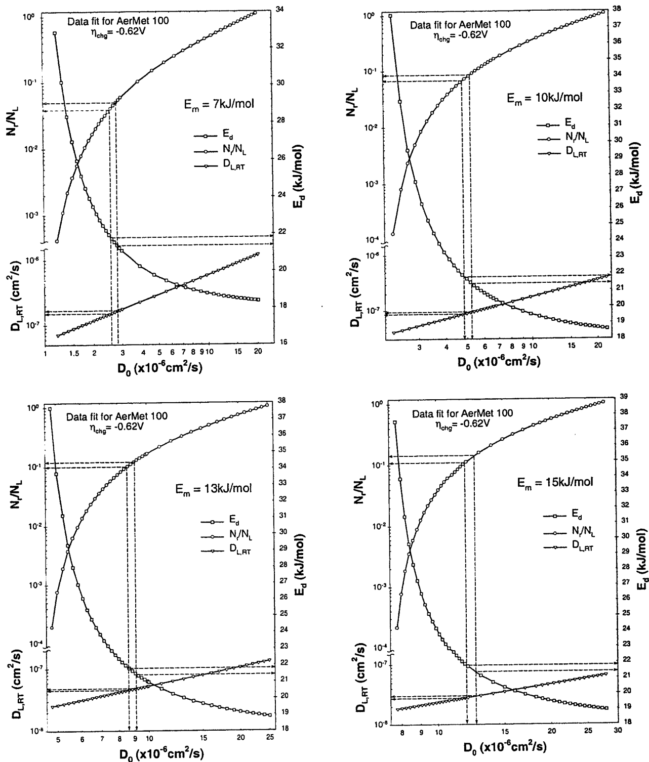
Fig. 14. Selected analytical results for optimizing desorption energy ( E_d ), trap fraction ( N/N_L ) and lattice diffusivity at room temperature ( D_{L,RT} ) by varying the pre-exponential constant D_0 and the migration energy E_m (data of D_{app} from AerMet ® 100 charged with \eta_{chg} = -0.62V )
