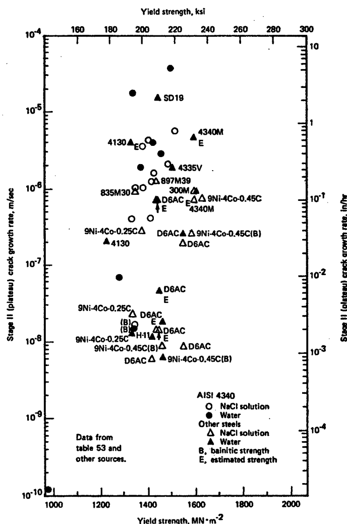
Figure 3 The dependence of da/dt_{II} on \sigma_{YS} for high strength steels in distilled water or chloride solution [68].
