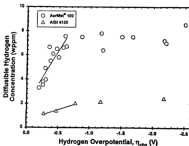
Fig. 9—Diffusible H concentration ( C_{H,diff} ) vs hydrogen overpotential for AERMET 100 and AISI 4130 charged in saturated Ca(OH) 2 at 23 °C. Hydrogen was extracted at 23 °C in saturated Ca(OH) 2 at an egress potential of -1.00 V Hg/Hg 2 SO 4 . The value of D_H from Eq. [6] was used in the calculation of C_{H,diff} with Eq. [5].
