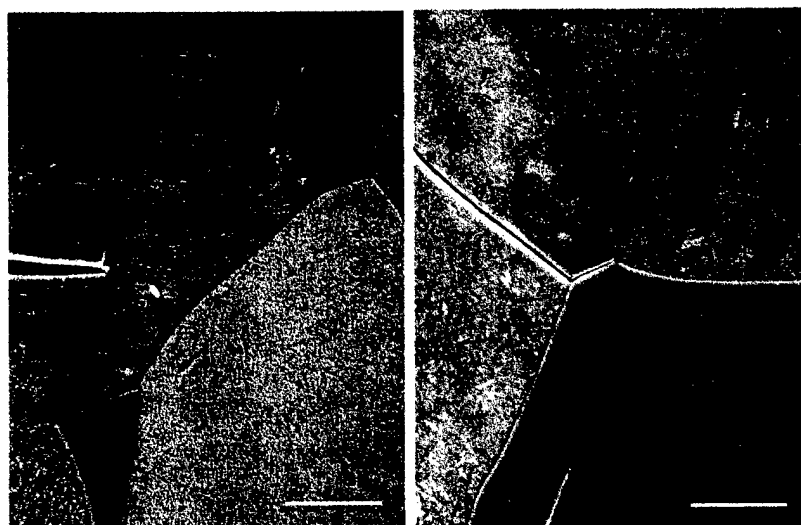
Figure 5 In situ SEM measurements of the Mode I crack tip opening vs. applied K for a transgranular fatigue precrack (left image and “TG crack”) and HEE-intergranular crack (right image and “TP IG crack”) in a high strength \beta+\alpha Ti alloy (Ti-8V-6Cr-4Mo-4Zr-3Al) [45,48]. The marker bar represents a distance of 20 \mu\text{m} and each specimen imaged was loaded in the vacuum chamber of an SEM to an applied K of 33 \text{MPa}\sqrt{\text{m}} .
