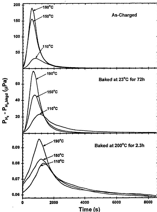
Fig. 5—Net H_2 pressure vs time at typical desorption temperatures for AERMET 100 specimens charged at \eta_{\text{chg}} = -0.62 V and 60^\circ\text{C} (background H_2 pressure, P_{H_2,\text{bkgd}} \approx 0.04 \mu\text{Pa} ). Conditions prior to the desorption are labeled on each plot.
