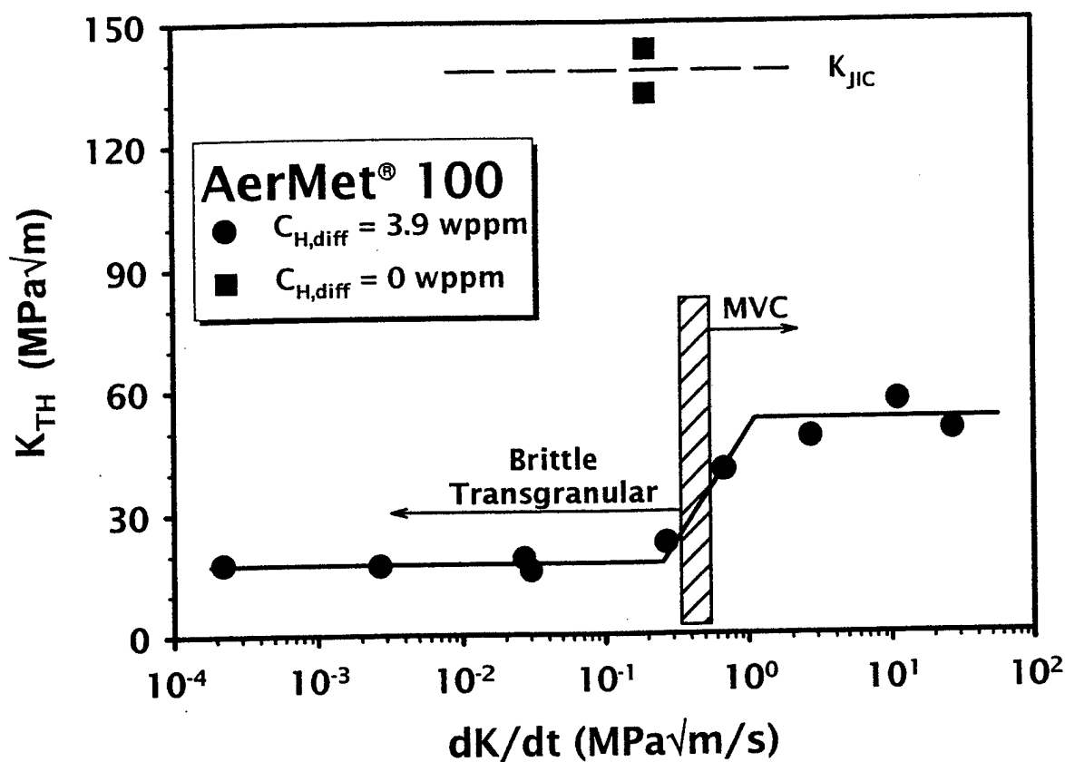
Figure 8. Threshold stress intensity, K_{TH} , vs. applied-initial dK/dt for AerMet®100 precharged to C_{H,diff} = 3.9 wppm. At dK/dt less than 0.3 MPa√m/s, brittle-TG fracture occurs at K_{TH} < 20 MPa√m. At dK/dt greater than 0.7 MPa√m/s, fracture occurs by MVC at K_{TH} < 60 MPa√m. The H-free plane strain elastic-plastic fracture toughness of AerMet®100 is 132-143 MPa√m.
