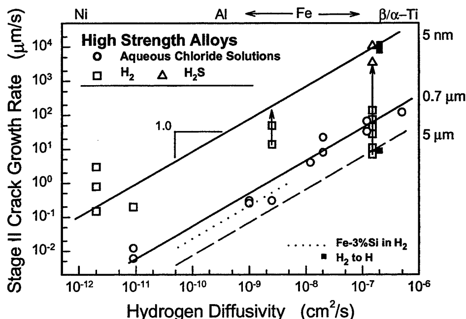
Figure 4 The dependence of da/dt_{II} on D_H for a wide variety of high strength alloys that exhibit HEE in various gases and electrolytes at 25°C.
