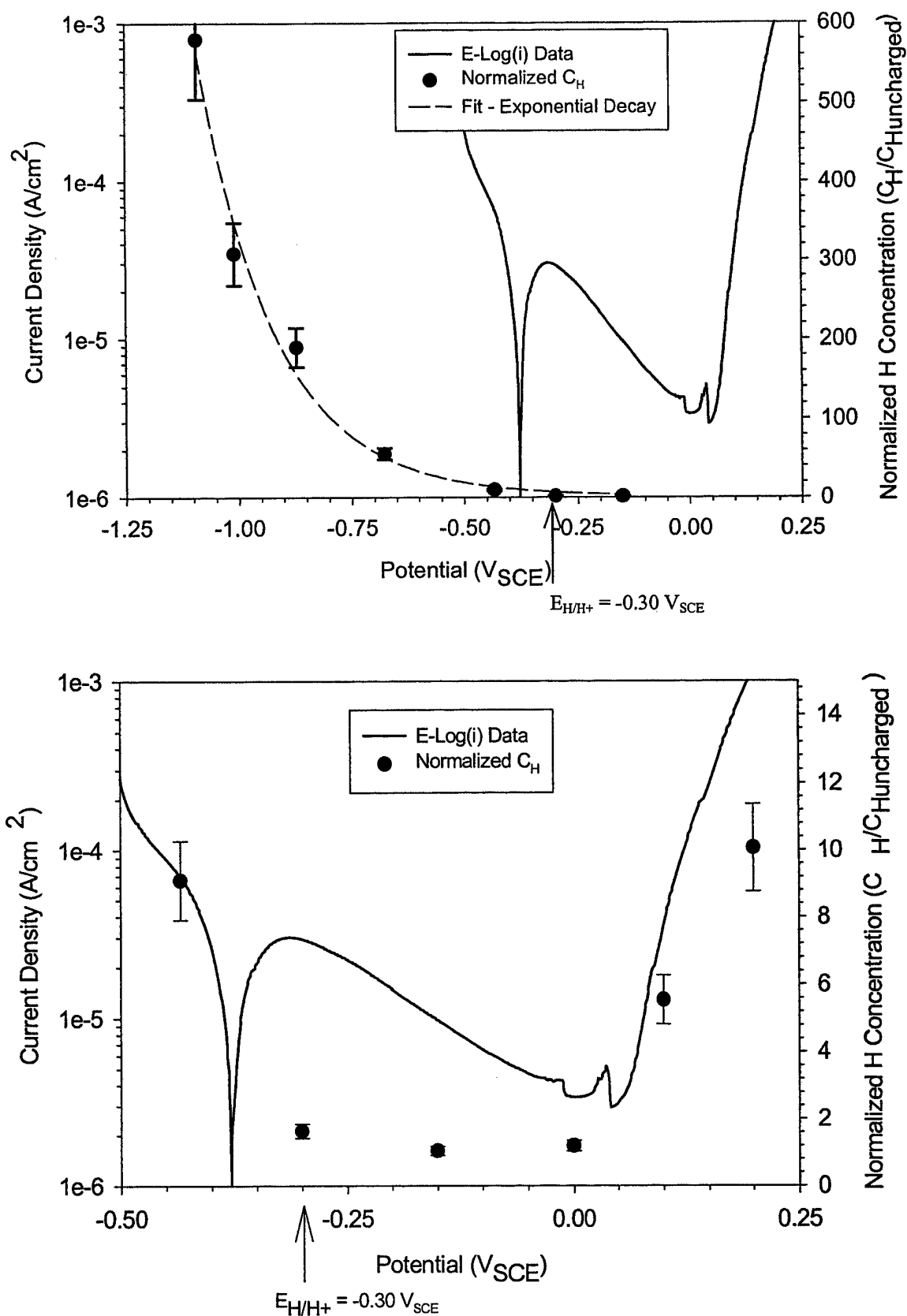
Figure 10. Relationship between C_H versus E_{true} from planar PH 13-8 Mo electrodes in deaerated 0.1 M HCl at 25°C (IR corrected). Top Figure illustrates exponential fit to data from near reversible hydrogen toward negative applied potentials (data at anodic potentials is omitted). Bottom plot illustrates enlarged view of hydrogen absorption near open circuit and after anodic polarization.
