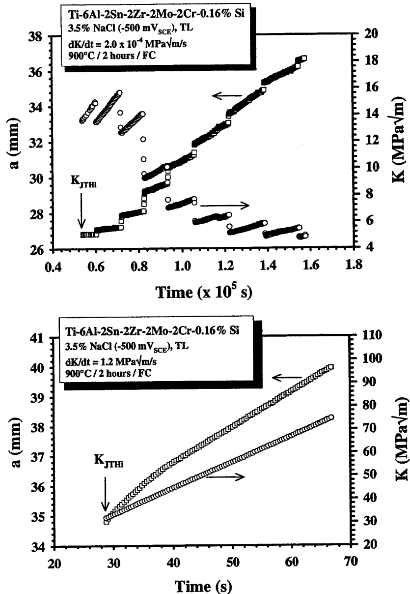
Figure 2 - Crack length and K vs. time for Ti-6-2222 plate in 3.5% NaCl (-500 mV SCE ) for: (a) initial dK/dt of 2.0 \times 10^{-4} MPa√m/s (top) and (b) 1.2 MPa√m/s (bottom).
