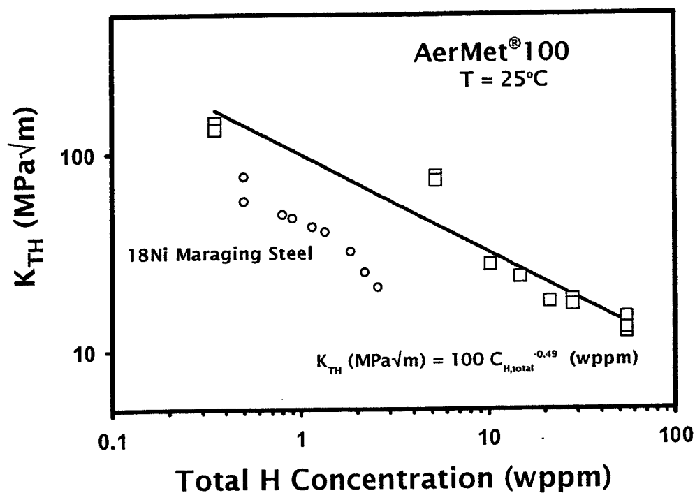
Figure 13. (a) The diffusible-hydrogen concentration dependencies of K_{TH} for IHE of AerMet®100 (□ from Fig. 4a), the combined IHE/HEE of 4340-type steels (dotted trend line and correlation equation from Yamakawa et al. [27]), and IHE of 4335 steel (○ [27]). (b) The total-hydrogen concentration dependencies of K_{TH} for IHE of AerMet®100 (□ from Fig. 4b), and IHE of 18Ni (270) and (290) Maraging steels (o from Ref. [19]).
