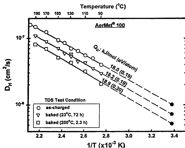
Fig. 6—Apparent hydrogen diffusivity, D_H , vs 1/T for specimens of AERMET 100 charged at a H overpotential of -0.62 V and 60^\circ\text{C} . Tests were performed in the as-charged condition and after two different baking conditions.
