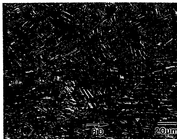
Figure 1 - Optical micrographs of annealed and furnace cooled Ti-6-4 (top) and Ti-6-2222 plates.
