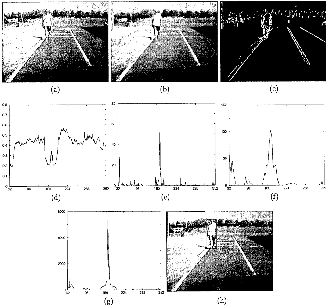
Figure 2: Intermediate results leading to the localization of bounding boxes: (a) original image; (b) clustered image; (c) vertical edges; (d) histogram representing grey level symmetries; (e) histogram representing vertical edges symmetries; (f) histogram representing vertical edges density; (g) histogram representing the overall symmetry S for the best bounding box for each column; (h) the resulting bounding box.
