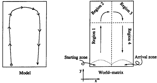
Figure 5: Artificial ants move through the world-matrix starting from the left half of the lower border, and moving through regions 1, 2, 3 and 4 until they reach the arrival line.
