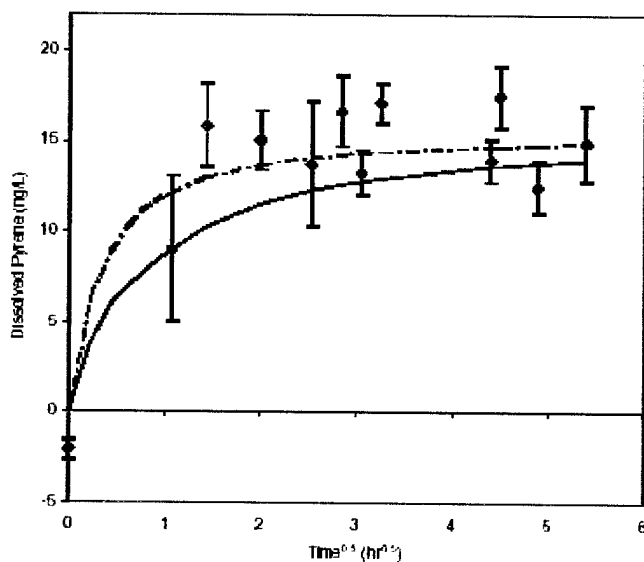
Figure 1. Dissolved pyrene (ng/L) (solid diamond) vs. time 0.5 at 25°C. The error bars are ±1 s.d. When the first four experimental data points were fit, the resulting De_{eff}/a^2 was 5.6E-7s^{-1} (dotted line). When only the first two data points were used to fit, the De_{eff}/a^2 was 1.0E-7s^{-1} (solid line).
