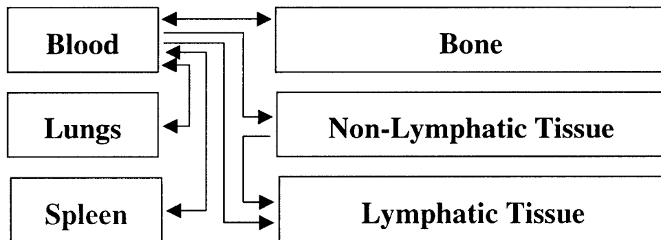
Figure 12 - Lymphocytopoiesis compartment model
