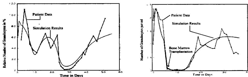
Figure 14 - Granulocyte dynamics modeling for acute irradiation exposure in Chernobyl (L) and Israel (R)
