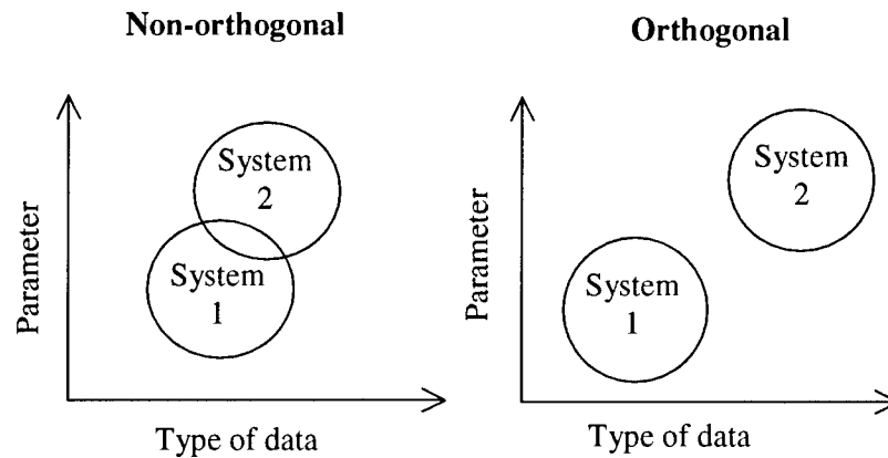
Figure 21 - Descriptive of orthogonality in phase space
