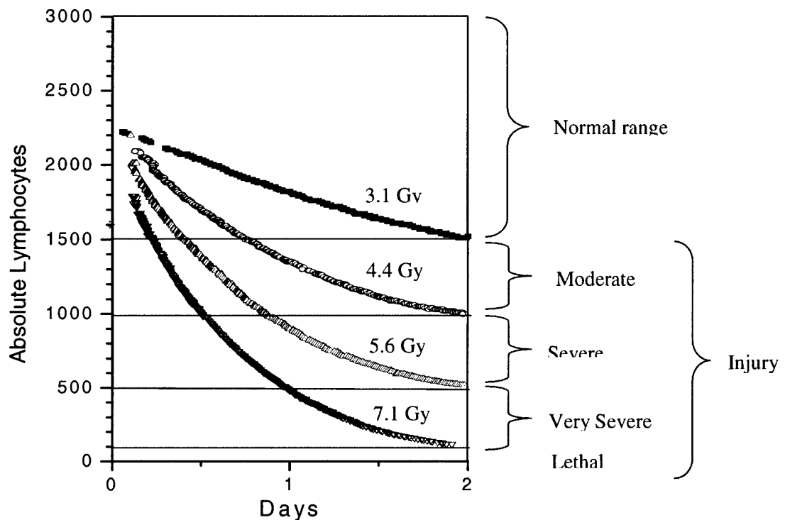
Figure 9 - Patterns of early lymphocyte depletion for radiation insults
