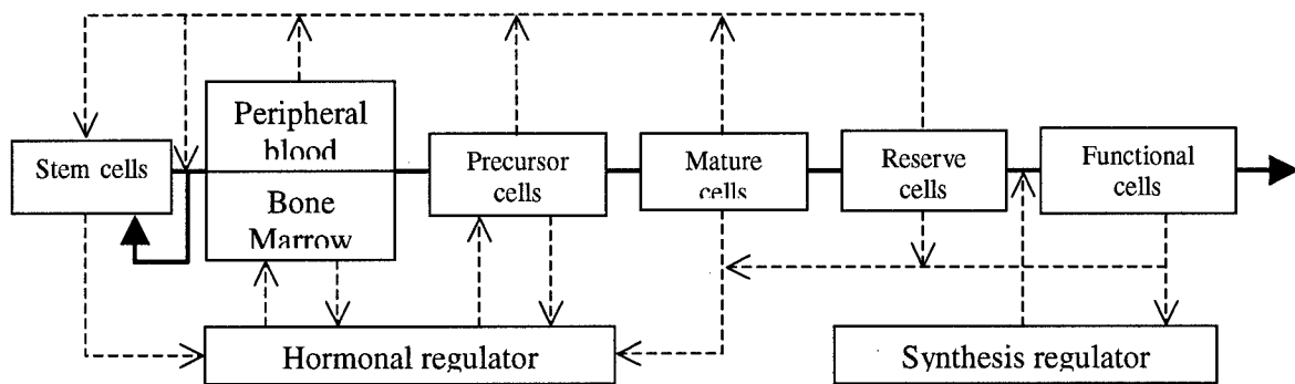
Figure 13 - Granulocytopoiesis compartment model
