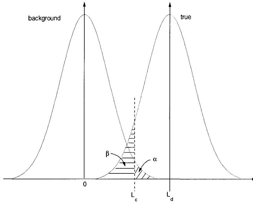
Figure 25 - Overlapping Gaussians depicting the distribution of net signal
