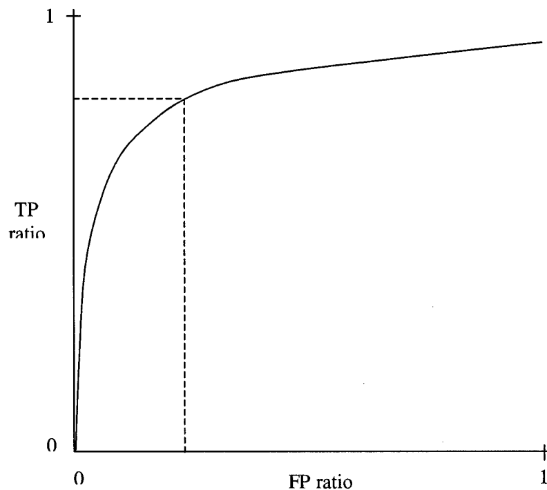
Figure 23 - Ideal ROC curve
