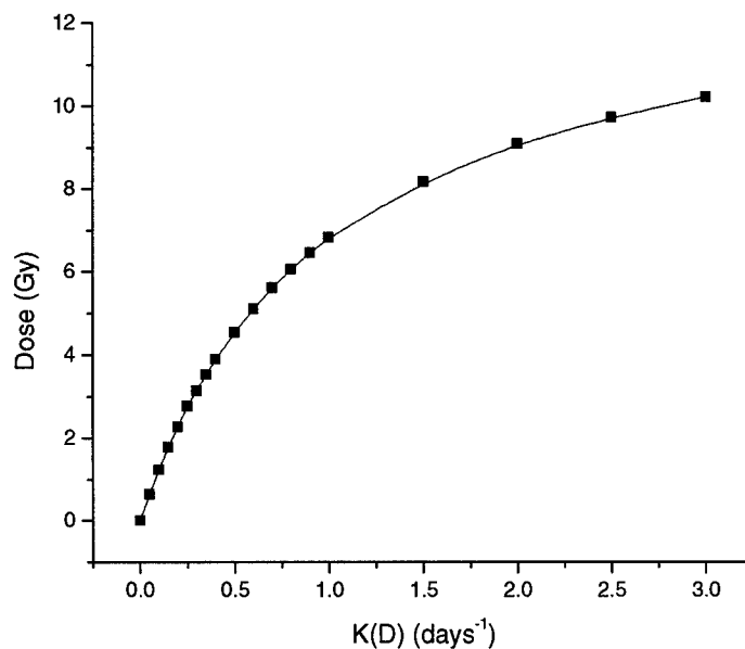
Figure 15 - Lymphocyte depletion rate constant as a function of dose
