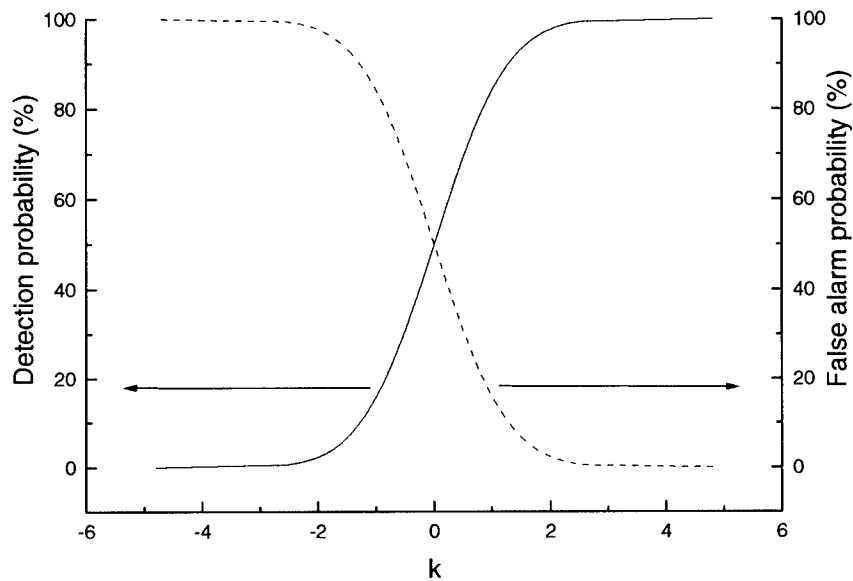
Figure 24 - Gaussian probability functions
