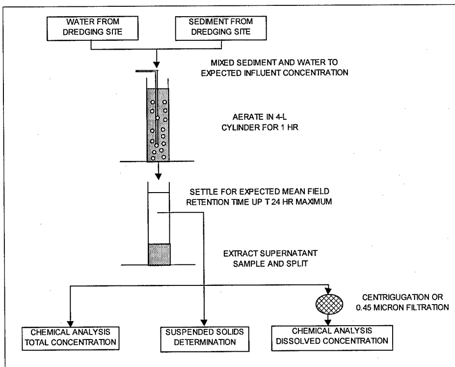
Figure B3. Modified elutriate test procedure
