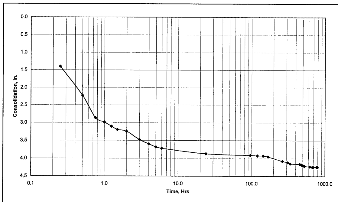
Figure A7. Self-weight consolidation test curve for Puddledock
