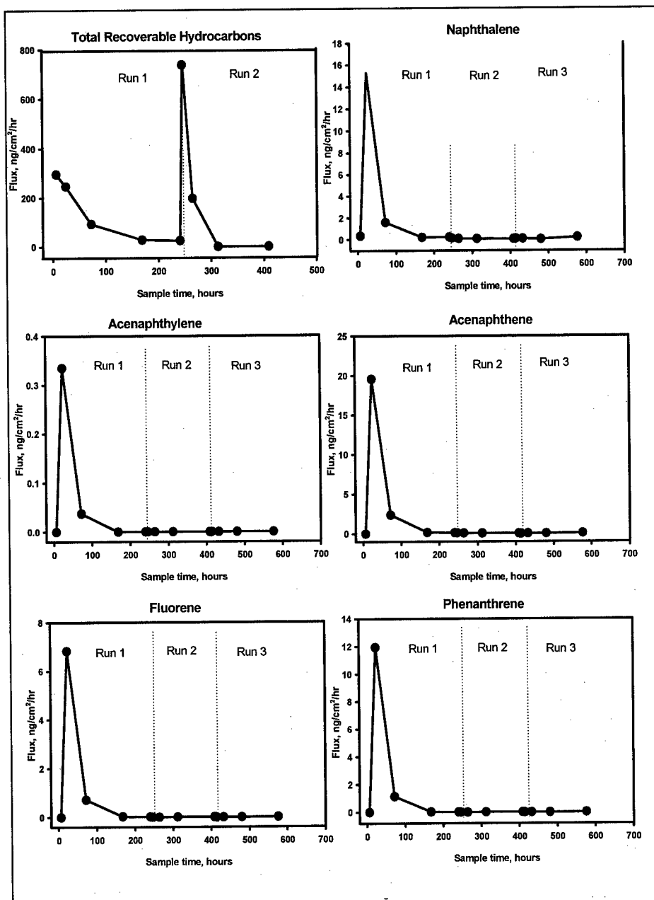
Figure F2. TRPH and PAH fluxes
