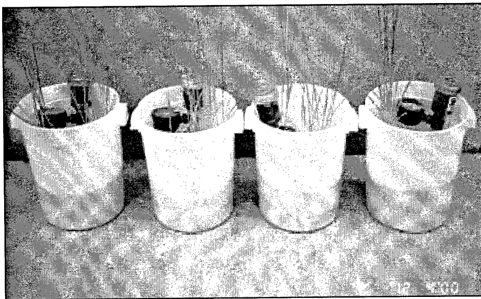
Figure D2. Appearance of C. esculentus in Puddledock sediment
