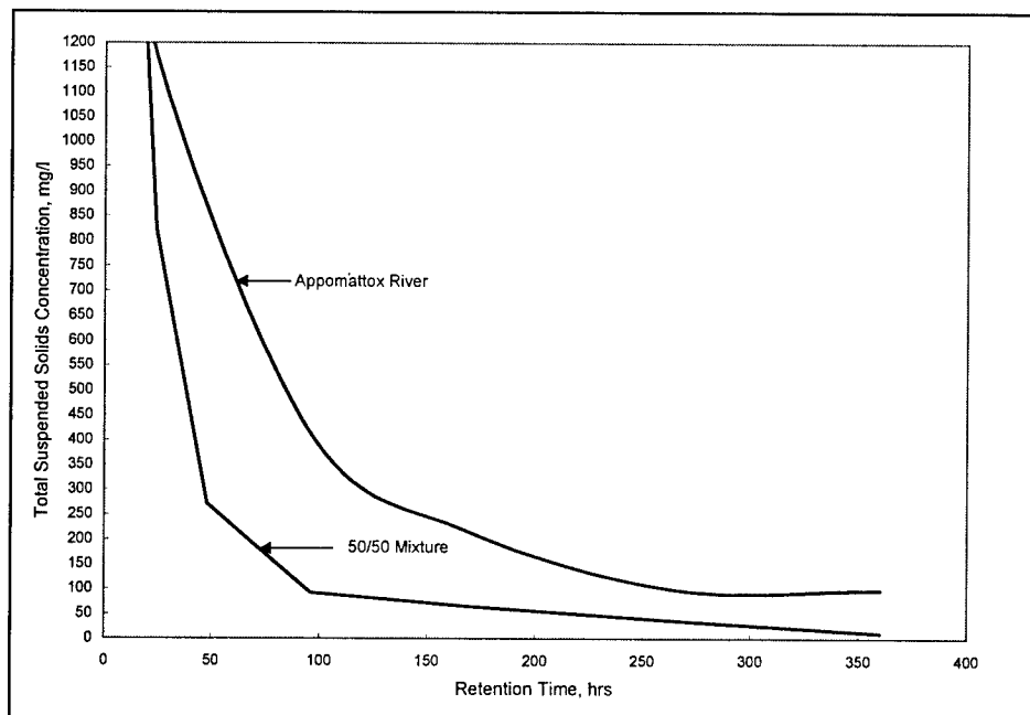
Figure B8. 2-ft ponding depth from supernatant suspended solids curve
