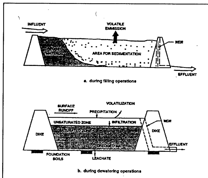
Figure 6. Upland CDF's contaminant pathways
