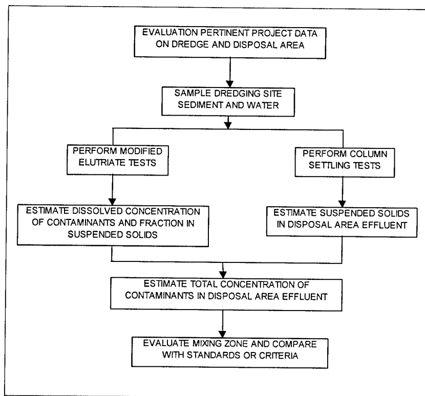
Figure B2. Steps for predicting effluent water quality
