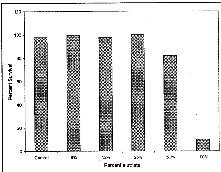
Figure 7. Survival of Pimephales promelas
