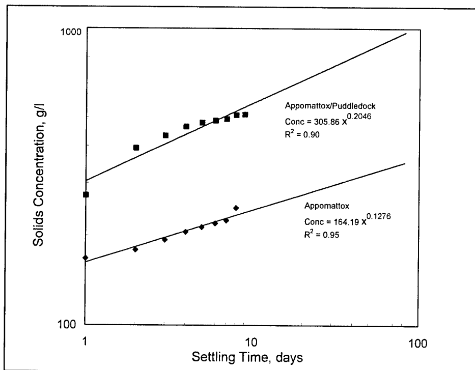
Figure A3. Compression settling curve
