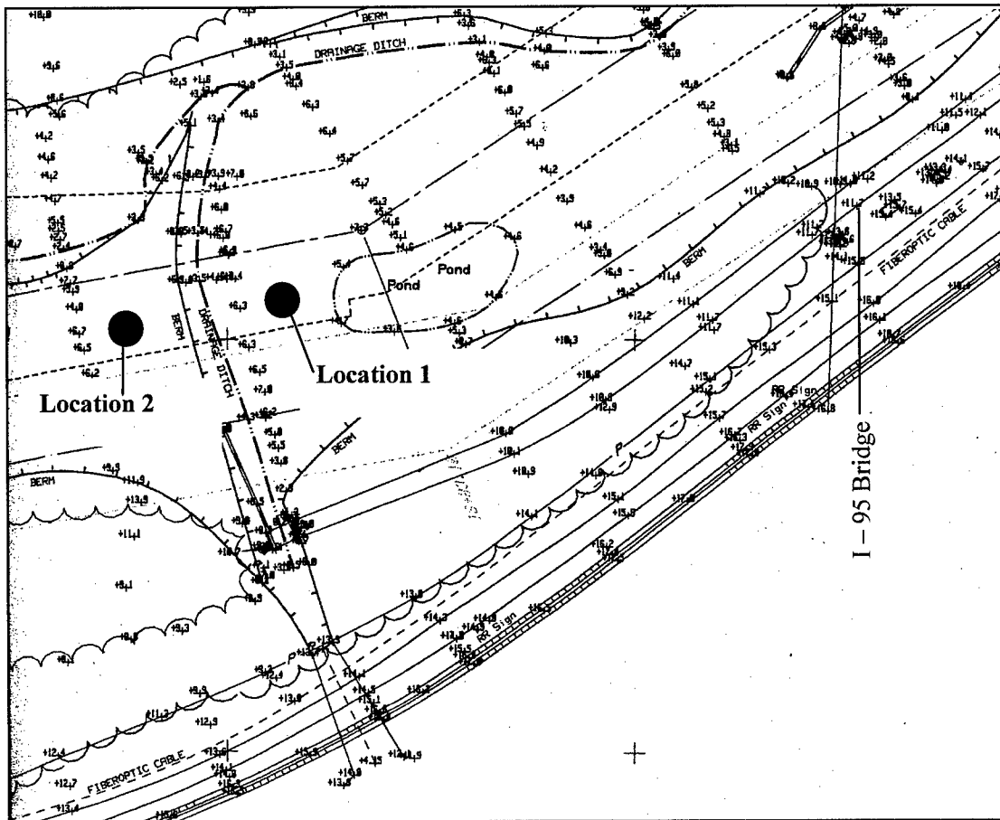
Figure 3. Appomattox River Navigation Channel sediment sample locations
