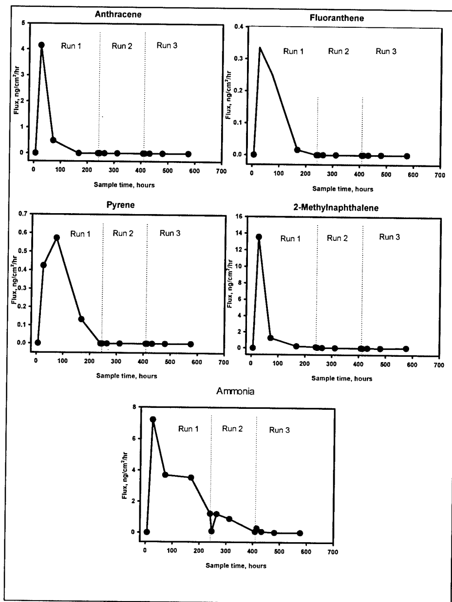
Figure F3. PAHs and ammonia fluxes
