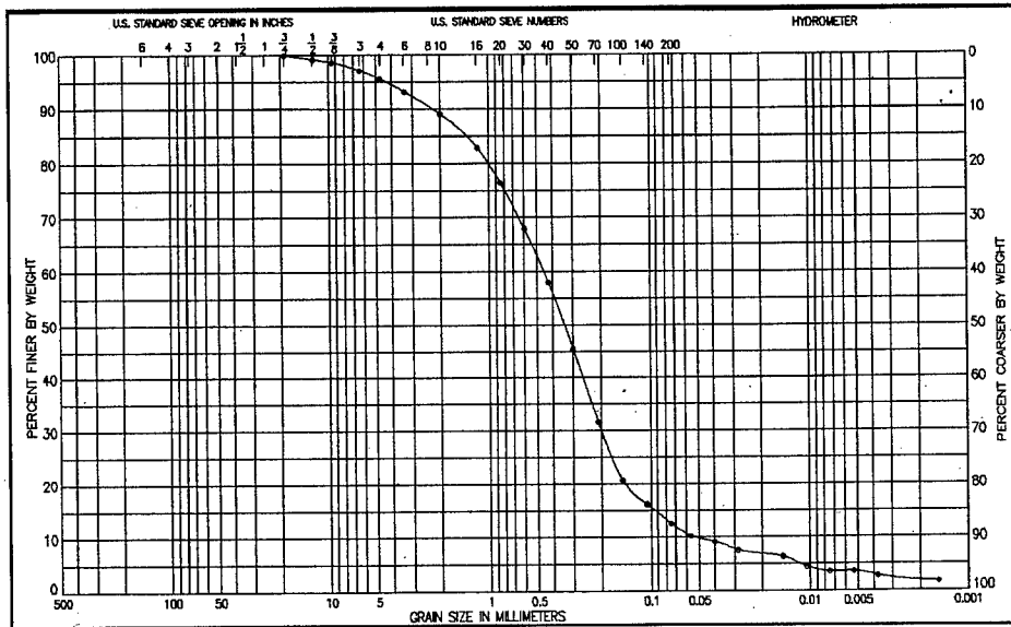
Figure A5. Appomattox River grain-size distribution curve
