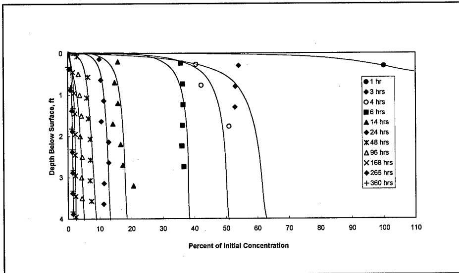
Figure B5. 50/50 Mix suspended solids relationship to time and depth below surface
