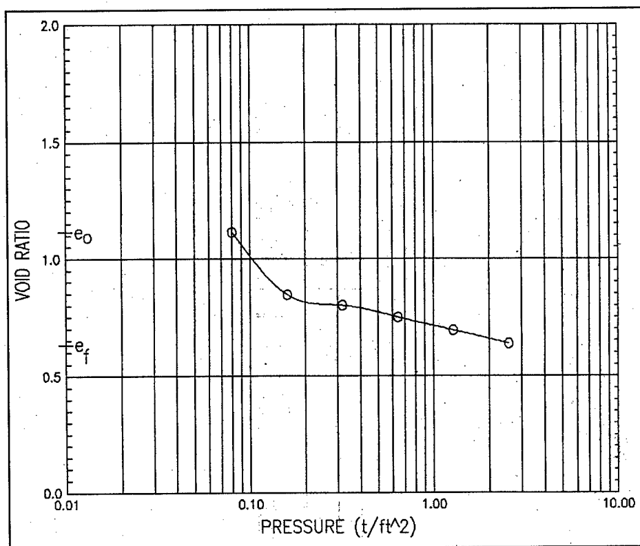
Figure A9. Void ratio-effective stress relationship for Puddledock
