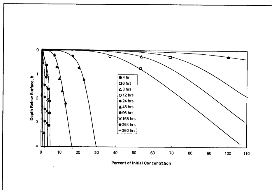
Figure B4. Appomattox River suspended solids relationship to time and depth below surface
