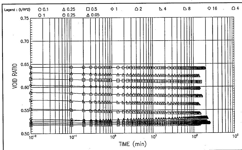
Figure A10. Time curve from standard oedometer consolidation test for Appomattox River sediment
