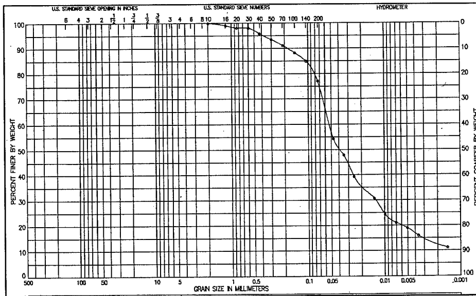
Figure A6. Appomattox River/Puddledock mixture grain-size distribution curve
