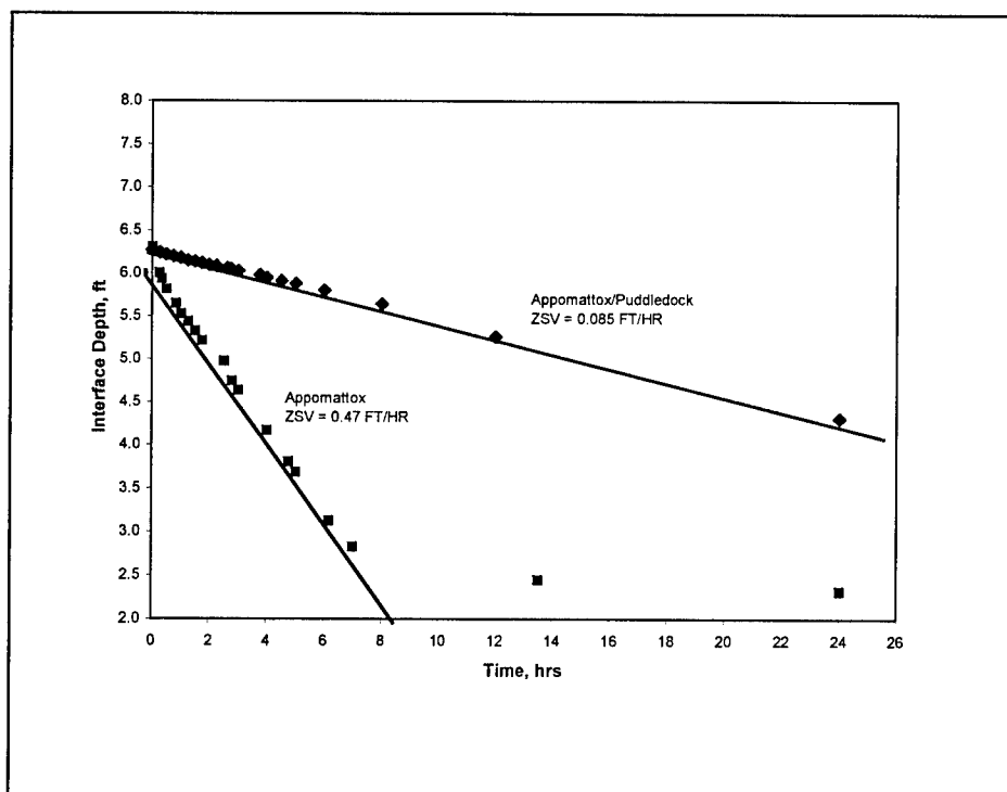
Figure A4. Zone settling curve
