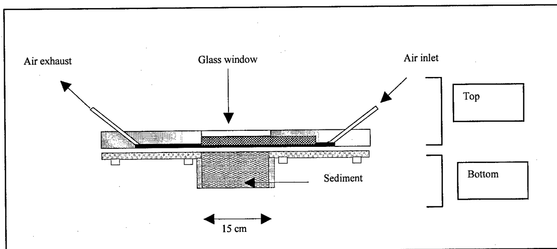
Figure F1. Laboratory flux chamber
