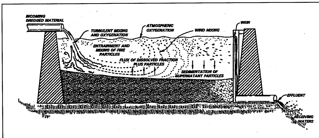
Figure B1. Schematic of an active CDF
