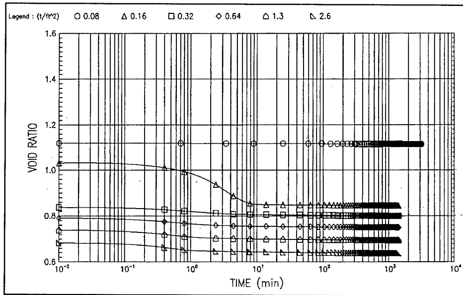
Figure A11. Time curves from standard oedometer consolidation test for Puddledock
