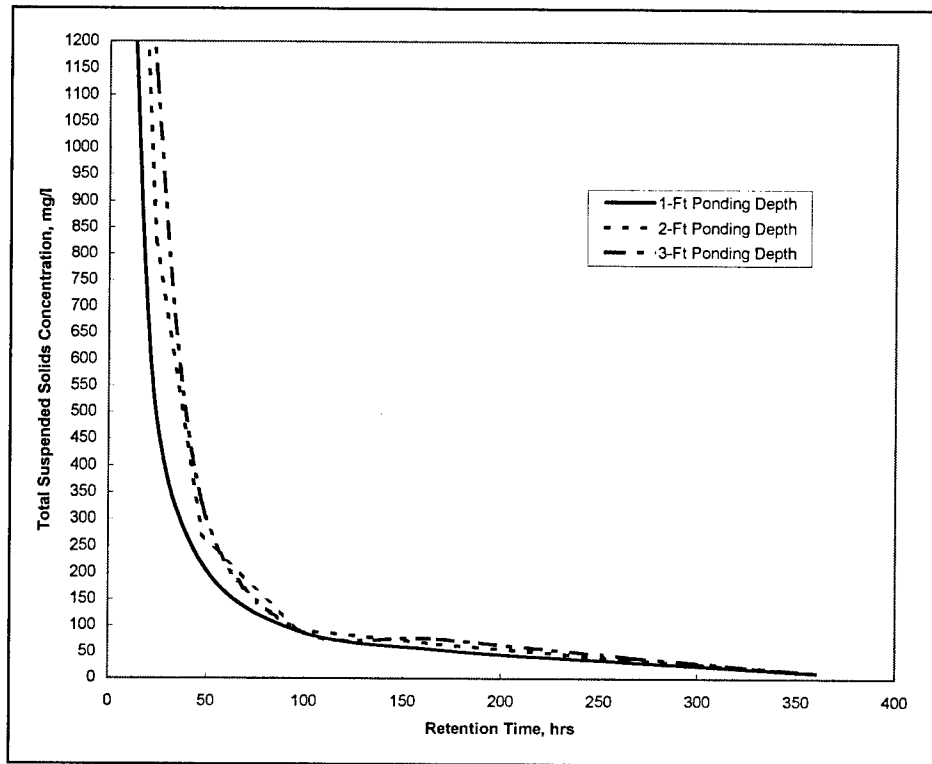
Figure B7. 50/50 Mix supernatant suspended solids curves
