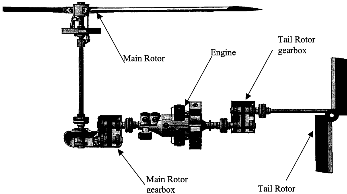
Figure 14 Transmission System Cross Sectional Drawing
