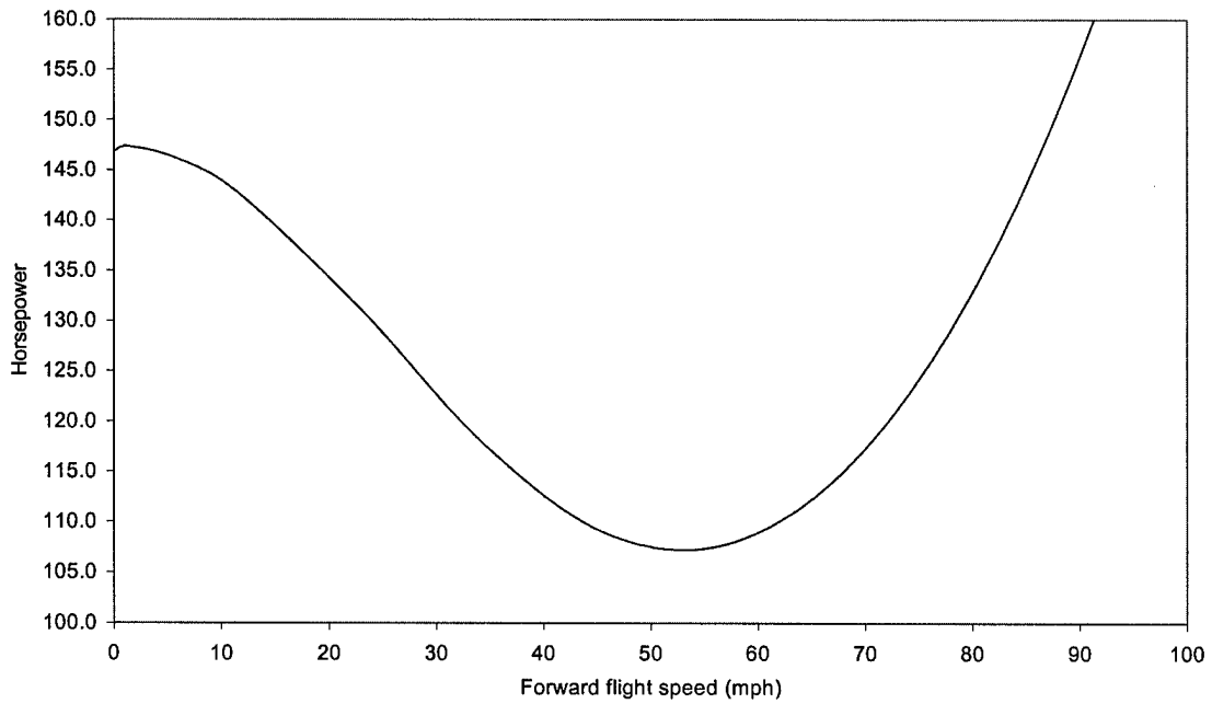
Figure 7 Power Required to Climb at 500fpm
