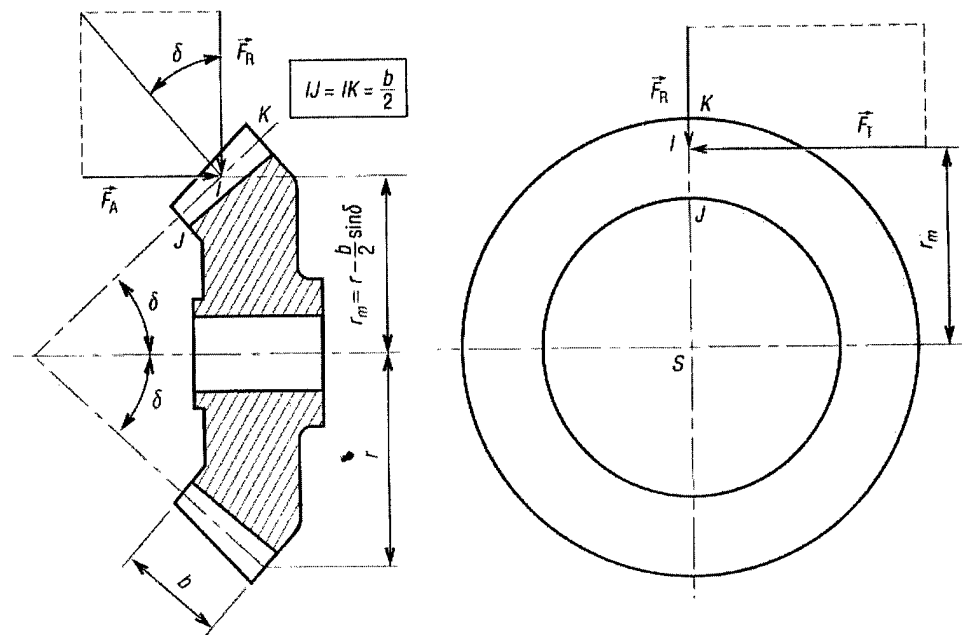
Figure 24 Cross sectional of bevel
