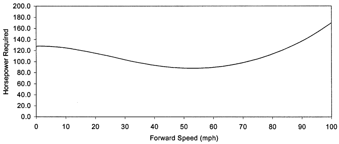
Figure 6 Total Power Requirements in Level Flight
