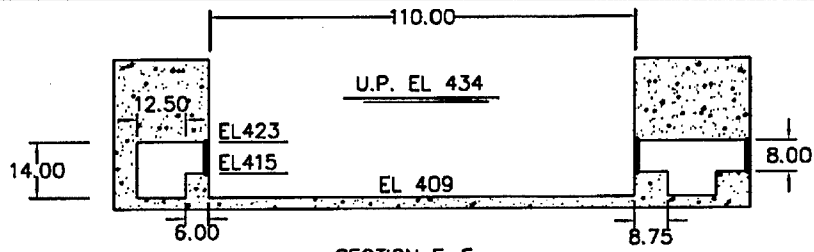
SECTION E-E AT INTAKE
