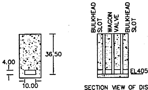
FRONT VIEW OF DISCHARGE PORTS
