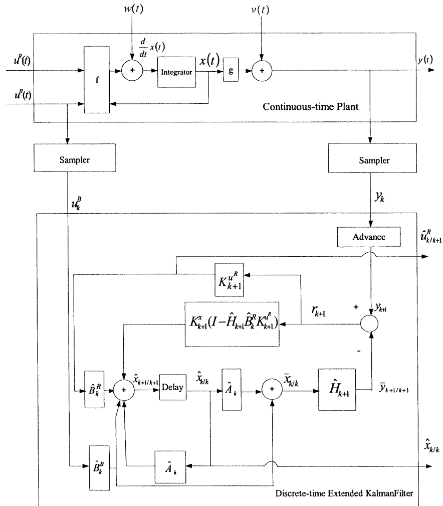
Figure 17.1: Block diagram of the extended Kalman filter
