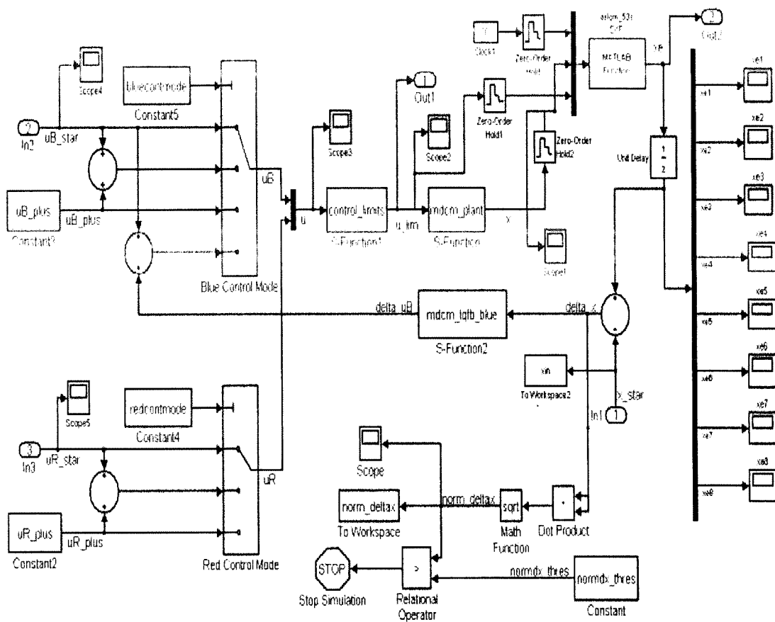
Figure 6.3: Closed-loop EKF combined with the game theoretic controller
