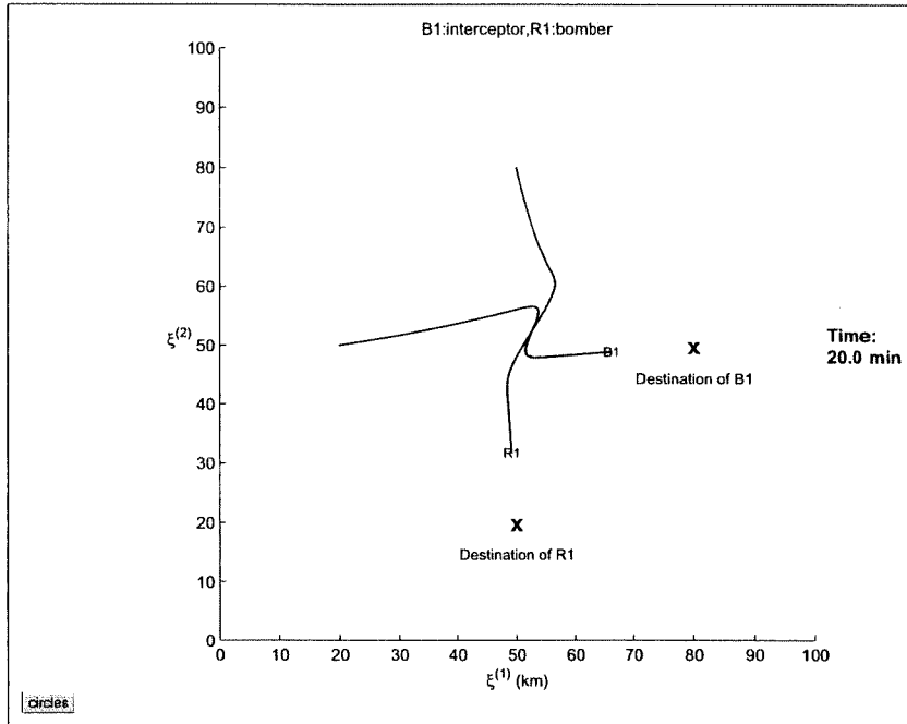
Figure 13.11: Comparison of MDCM (- -) and Averaged MDCM-SD (-) for Game Trajectories ( \Delta t = 0.01 ).
