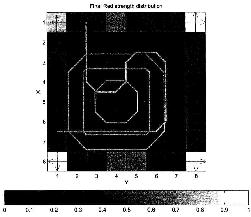
Figure 12.9: Final Strength Distribution for Red force. Arrows indicate magnitude of the velocity components across the boundaries.
