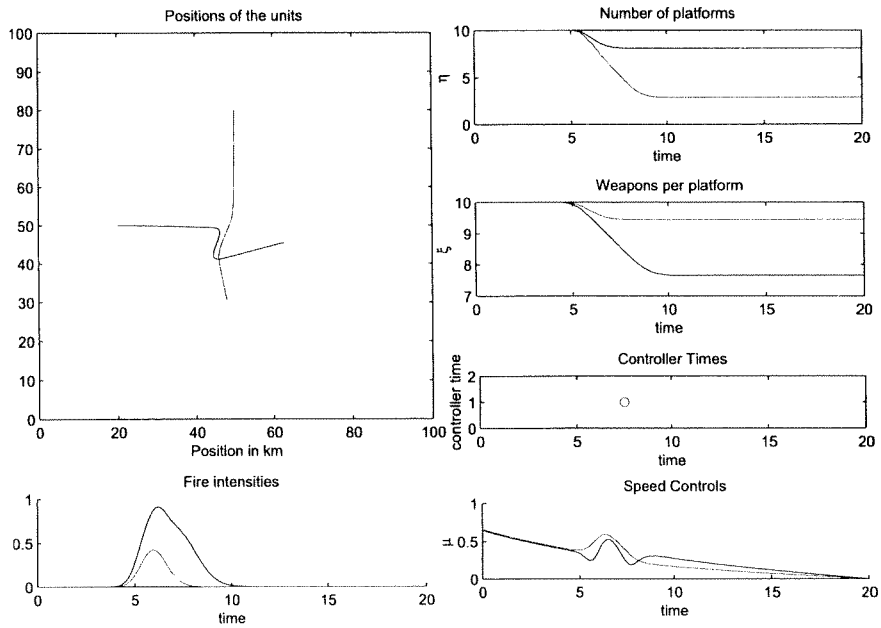
Figure 4.16: Blue Underestimates Red (Blue thinks \text{skillRed}=0.1 ) \text{pkill}:0.8
