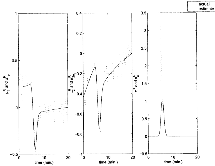
Figure 17.14: Red inputs for high process noise
