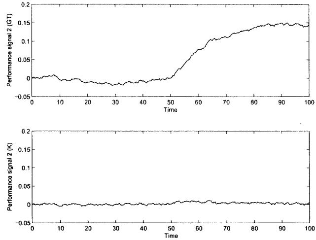
Figure 9.9: Response to Action 2 of the game-theoretic filter (top) and of the Kalman-like filter (bottom) under noise with energy equal to 25% of the energy of the noise-free output.
