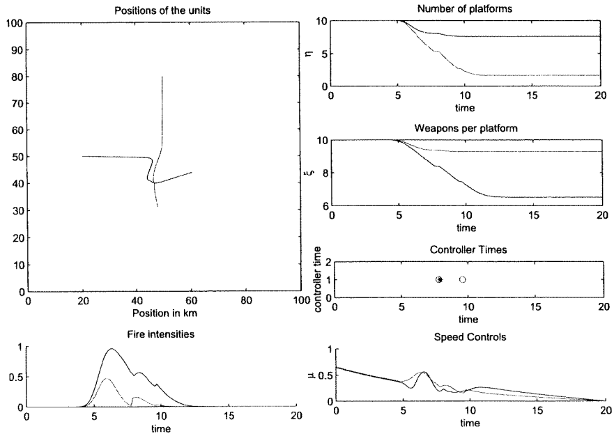
Figure 4.20: Both Sides Underestimate (Red thinks pkill_{Blue}=0.4 Blue thinks pkill_{Red}=0.1 ) pkill:0.8
