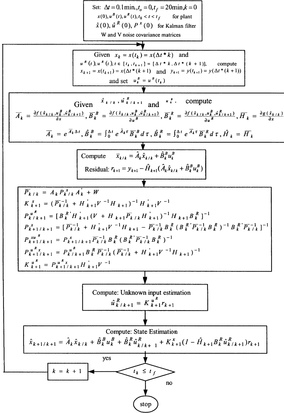
Figure 17.2: The flow chart of the estimation algorithm.
