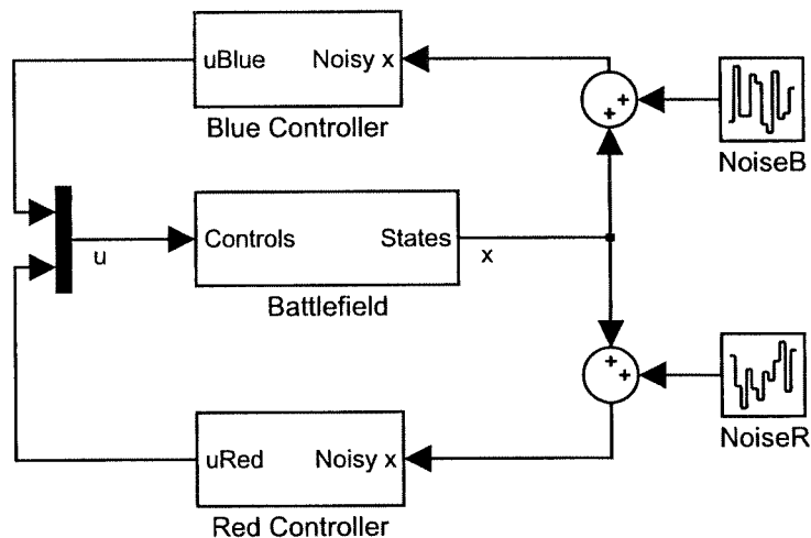
Figure 3.1: Controller-Plant-Controller Setup
