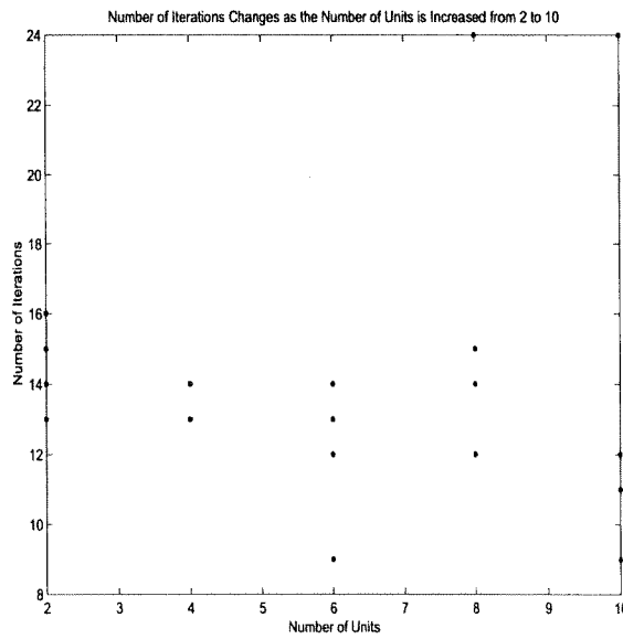
Figure 5.12: The Number Of Iterations Changes As The Number Of Units Is Increased
