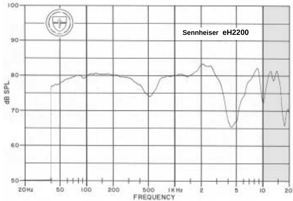
Figure 7. Averaged diffuse-field response of Sennheiser closed circumaural headset eH2200
