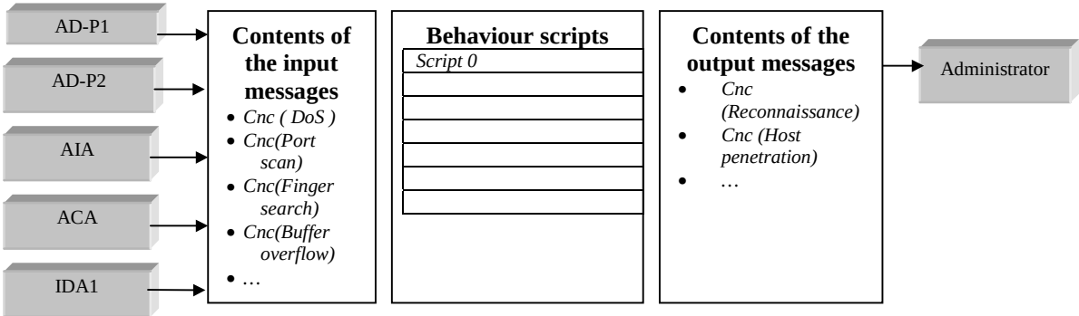
Fig.A.19. Common scheme of the agent IDA2 operation
