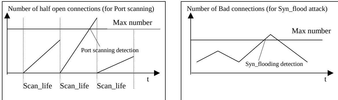
Fig.A.8. Graphical representation of rules of attack detection by the agent AD-P1
