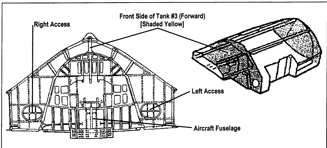
Figure 6. Aft Intermediate Fuselage Fuel Tank #3 Forward
