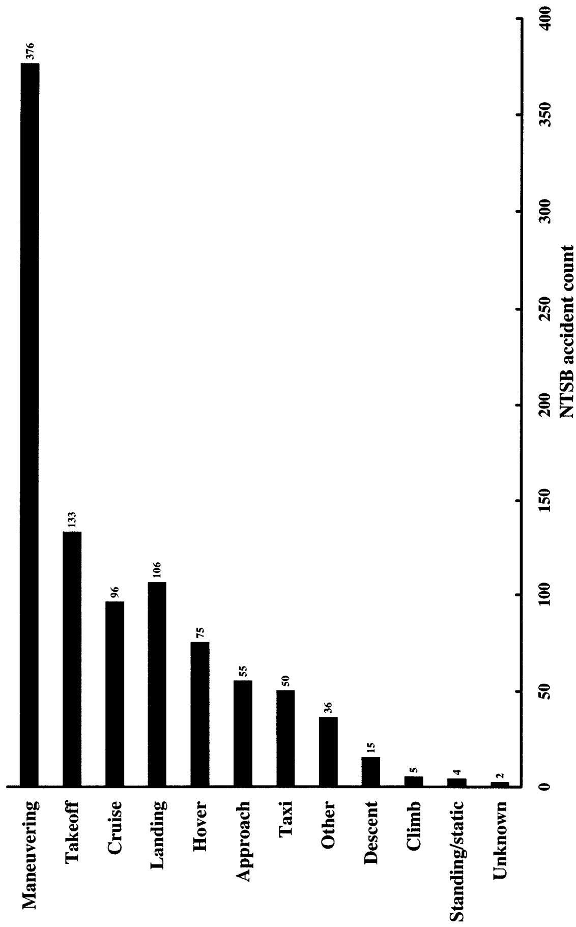
Figure 30. In flight collision with object accidents by phase of operation: single-piston helicopters (commercially manufactured).
