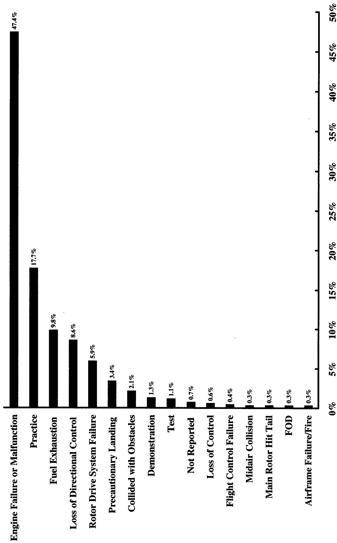
Figure C-6. Reasons for autorotation (problems during practice distributed to reasons).
