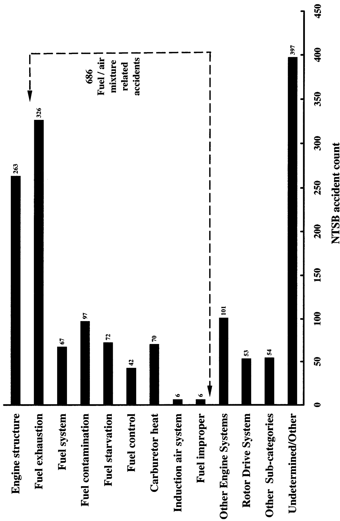
Figure 24. Loss of engine power accidents by category: single-piston helicopter (commercially manufactured).
