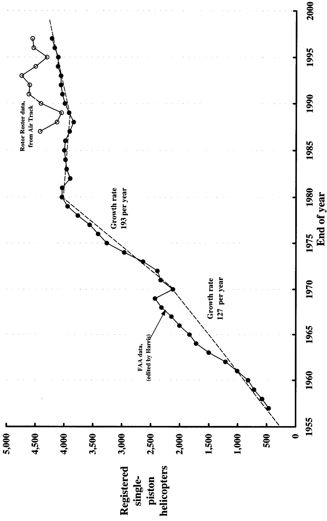
Figure 16. Single-piston helicopter fleet size (commercially manufactured).
