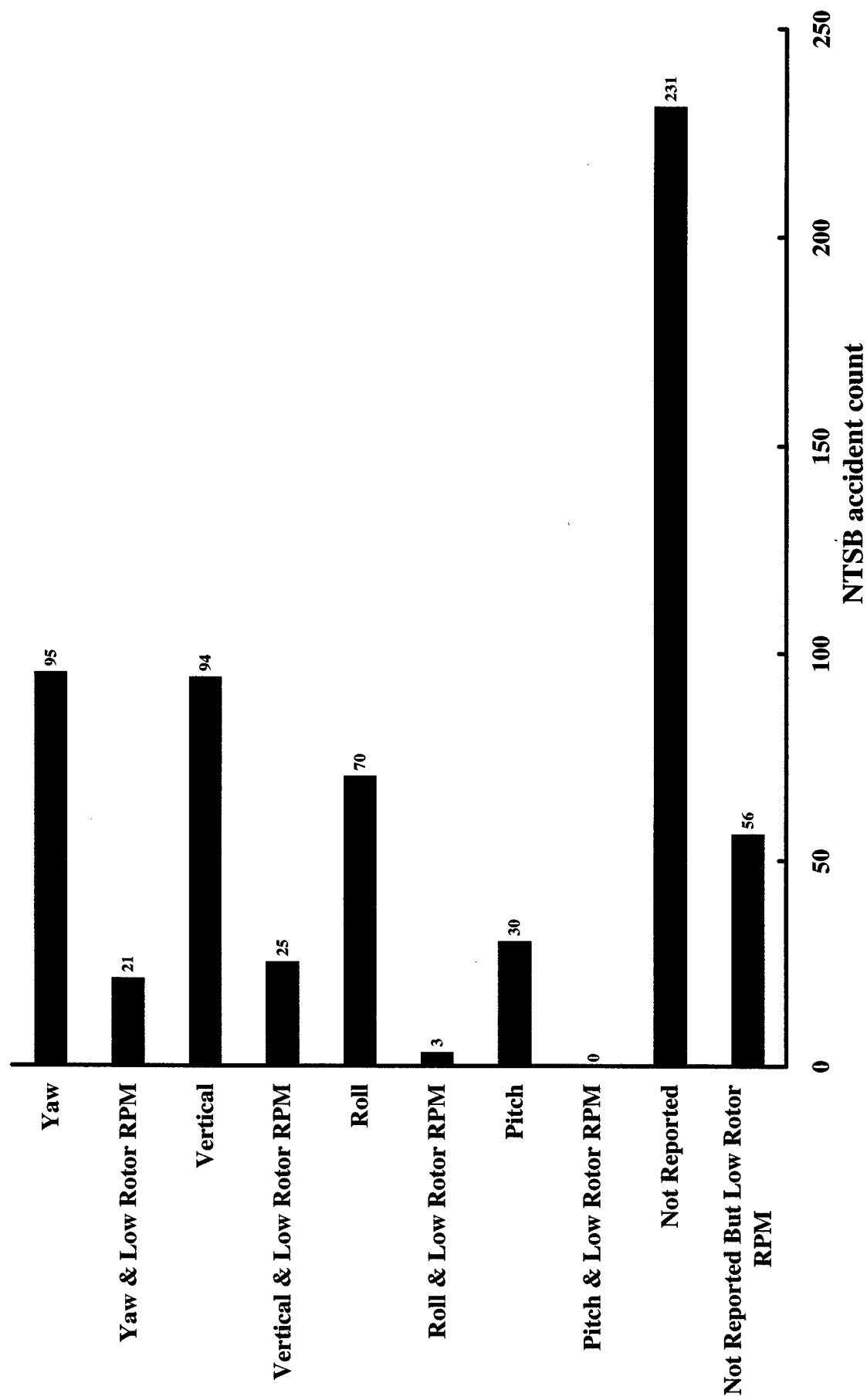
Figure 37. Loss of control accidents by axis lost: single-piston helicopters (commercially manufactured).
