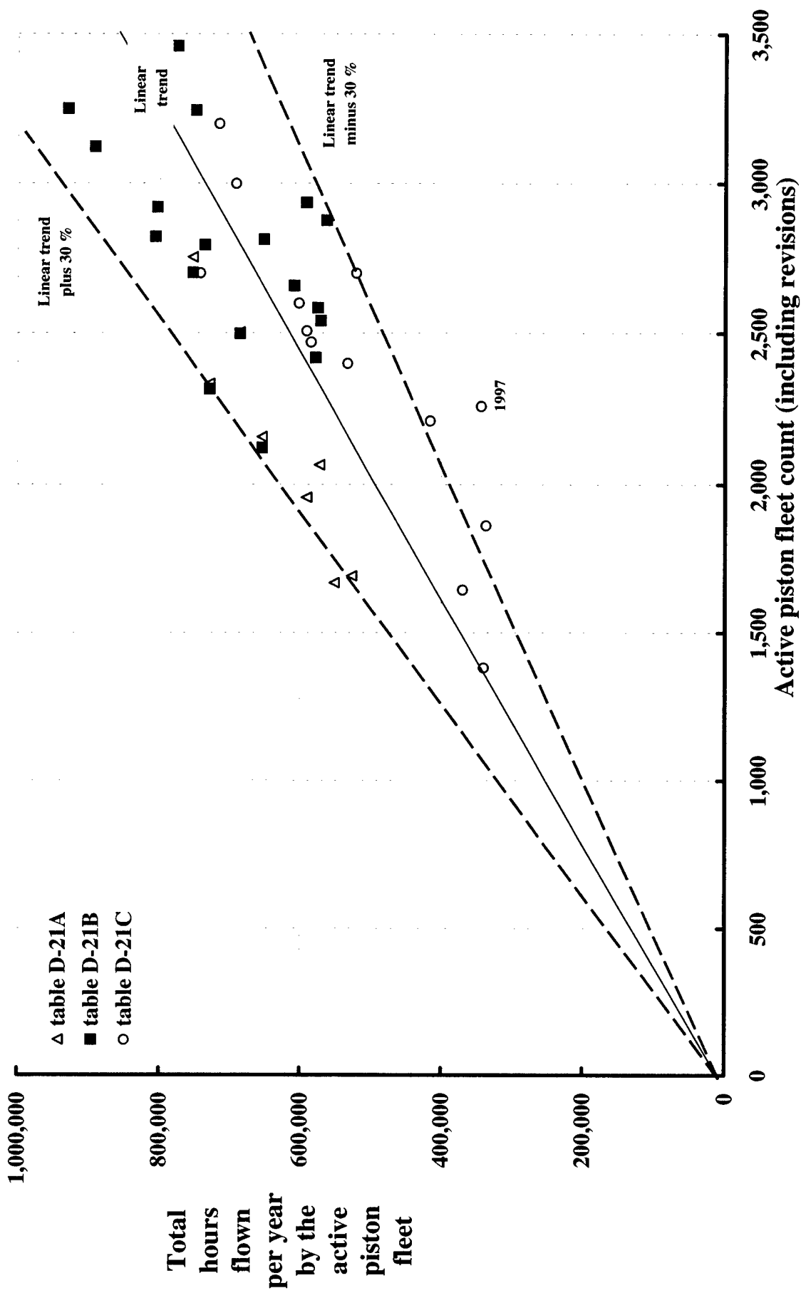
Figure B-8. Annual hours flown by active piston fleet vs. active piston fleet.
