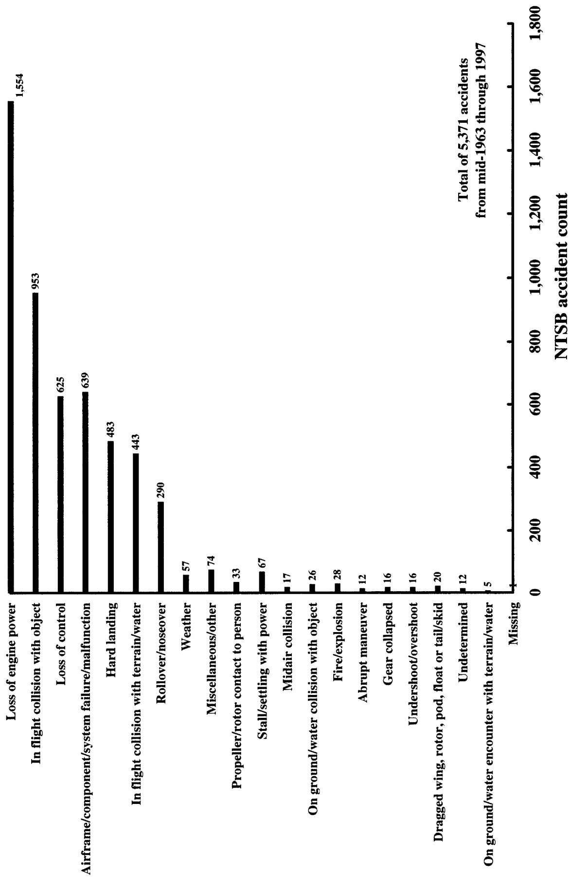
Figure 18. Accident count by first event category: single-piston helicopters (commercially manufactured).
