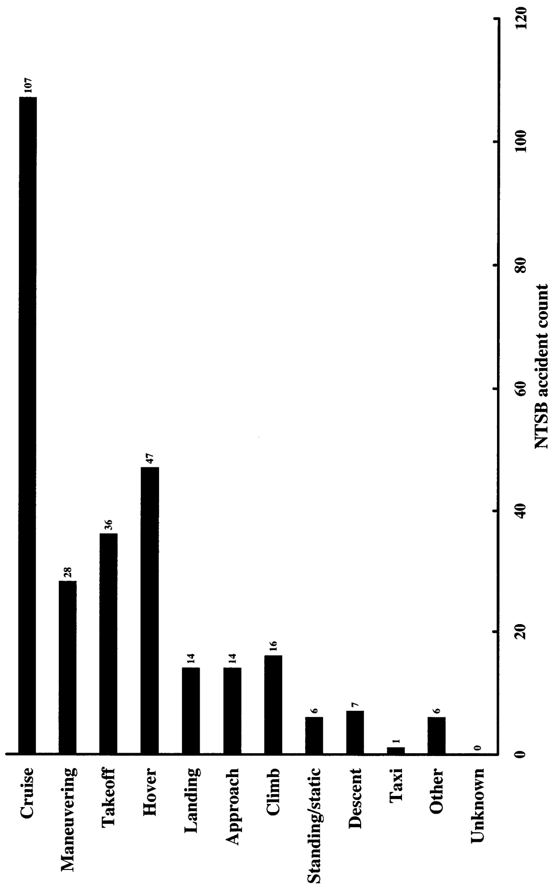
Figure 68. Airframe failure accidents by phase of operation: single-turbine helicopters (commercially manufactured).
