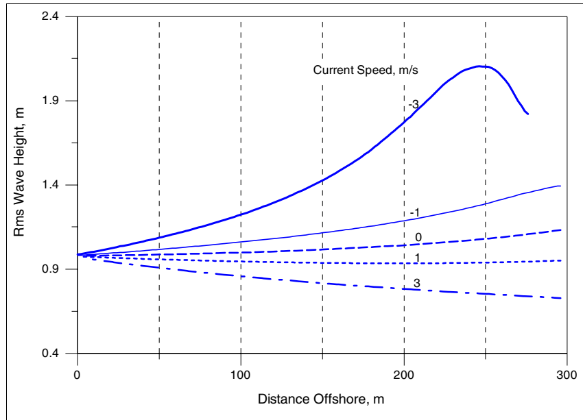
Figure 17. Calculated wave transformation on flood and ebb currents for conditions representative of Shinnecock Inlet, Long Island
