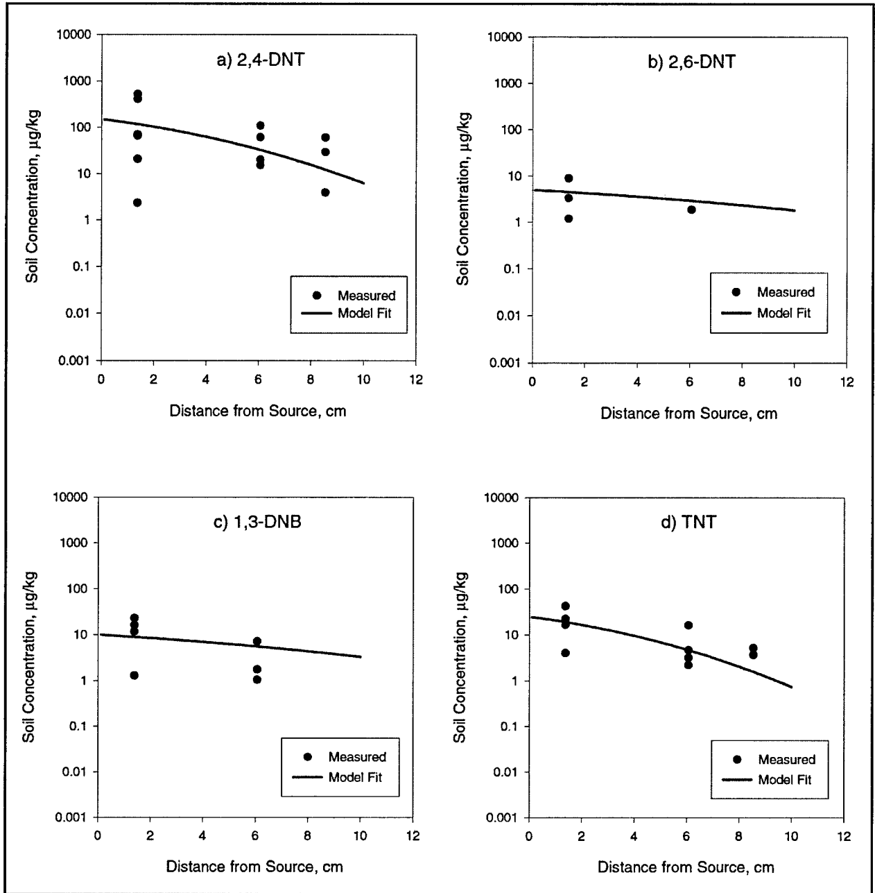
Figure 13. Comparison of experimental (data from Jenkins et al. (2000)) and model fit soil concentrations of 2,4-DNT, 2,6-DNT, 1,3-DNB, and TNT from buried TMA-5 type landmine, Fort Leonard Wood site, 41 days following burial
