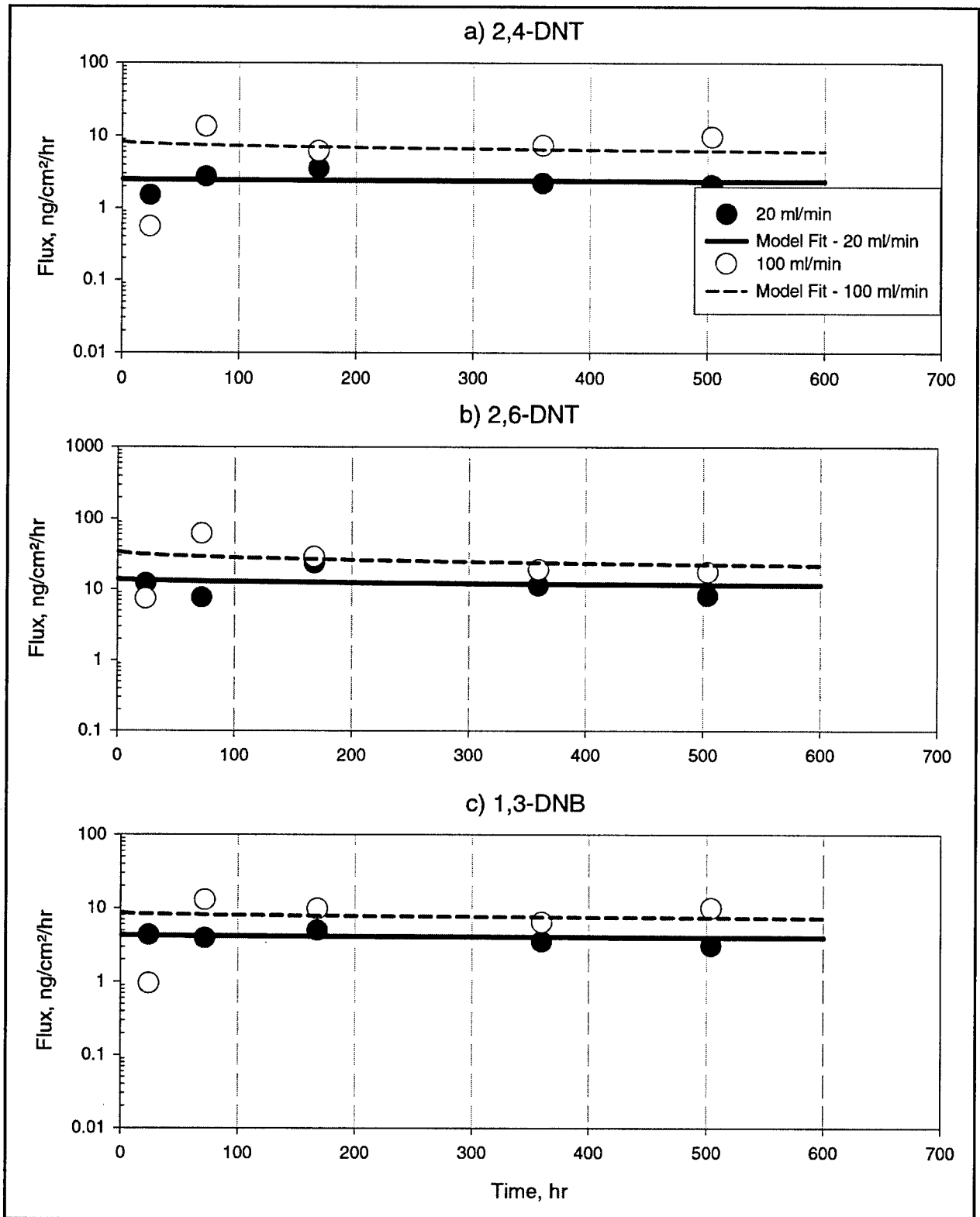
Figure 9. Comparison of experimental and model fit for 2,4-DNT, 2,6-DNT, and 1,3-DNB for case 4 for 20- and 100-ml/min airflow rates, LAAP-C soil, 20-percent soil moisture with humid air
