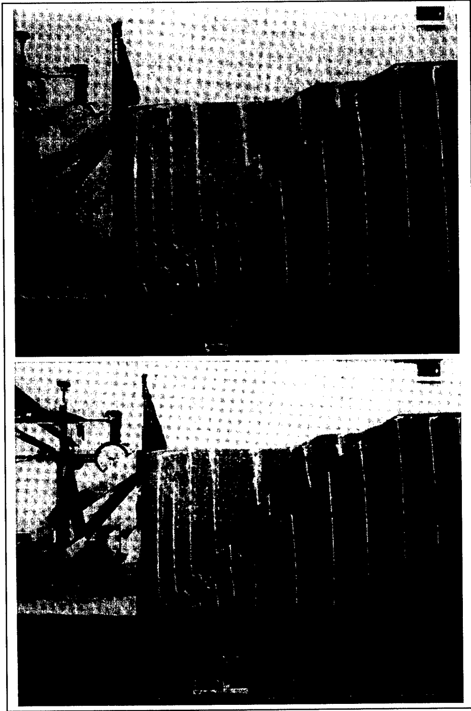
Figure 4-13. Shake table tests performed on scale models of retaining wall. Note the multiple failure planes in the backfill (from Aitken, Elms, and Berrill 1982)
