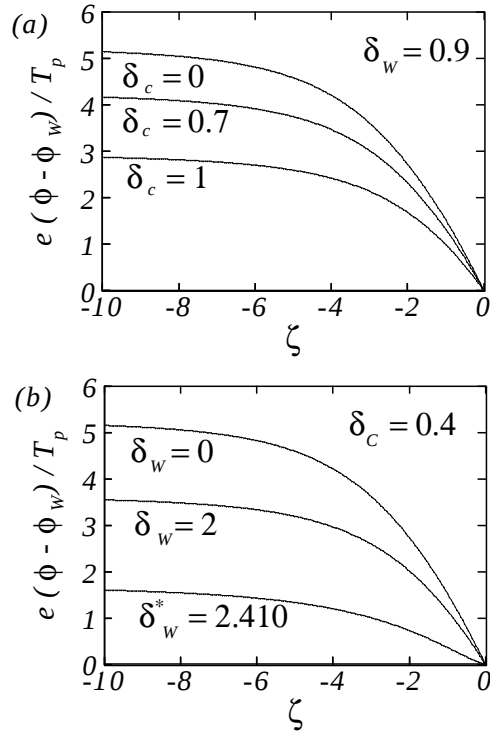
Figure 3.2: Sheath solution. Profiles of the electrostatic potential for: (a) \delta_w = 0.9 and several values of \delta_c from 0 to 1, (b) \delta_c = 0.4 and several values of \delta_w from 0 to 2.410.
