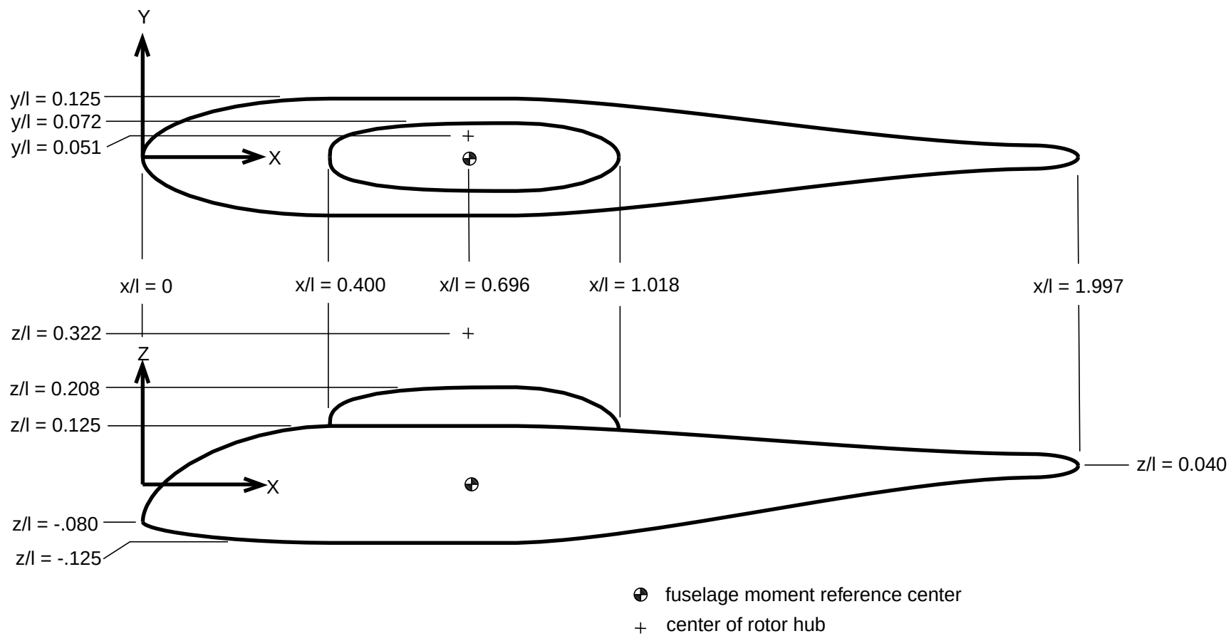
Figure 3. Sketch of the ROBIN configuration.
