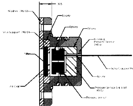
Figure 8 - Pressure Sensor Cross-Sectional View
