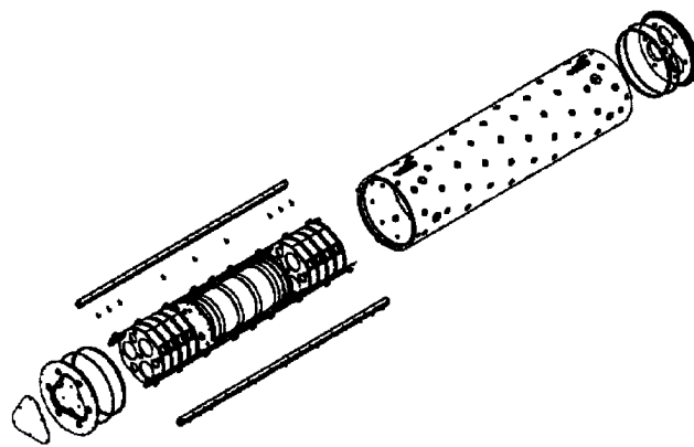
Figure 1 - Instrumented Mine Assembly Drawing
