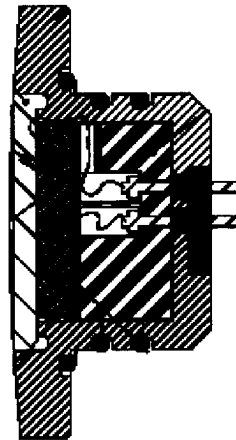
Figure 7 - Doppler Transducer Cross-Sectional View
