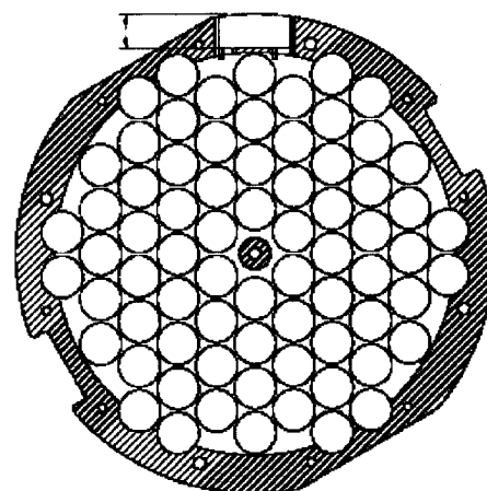
Figure 10 - Battery Pack Core
