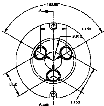
Figure 6 - ADCP Transducer Piezo Ceramic Element Configuration
