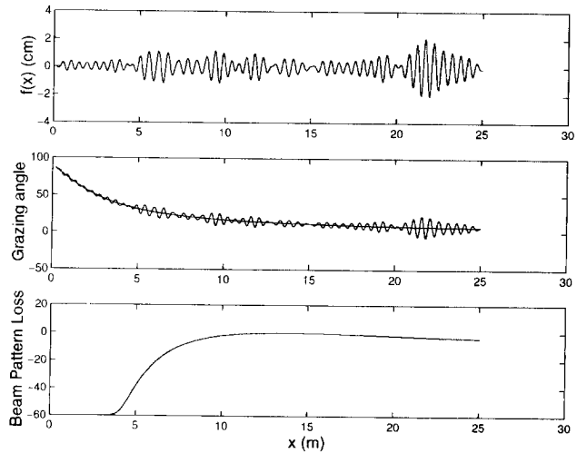
Fig. 2. One example of the rippled surface. The top panel gives the rough surface height. The middle panel shows the grazing angle in degrees: the fluctuating curve is the local grazing angle associated with the rough surface; the smooth curve is the grazing angle if the surface is flat. The bottom panel shows the source beam pattern loss in dB.
