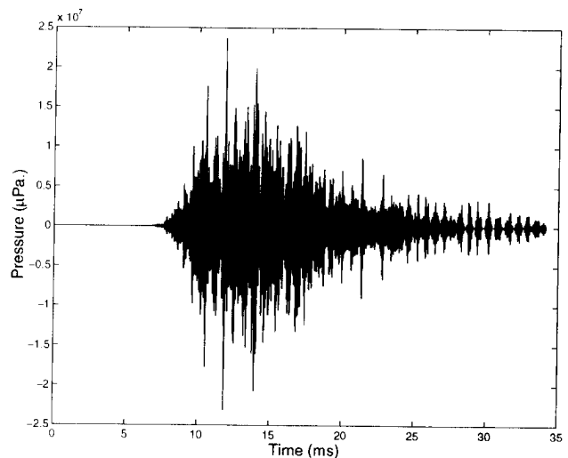
Fig. 3. Simulated pressure corresponding to the rough surface given in Fig. 2. The source level is 220 dB re 1 \mu\text{Pa} . The frequency is 300 kHz.
