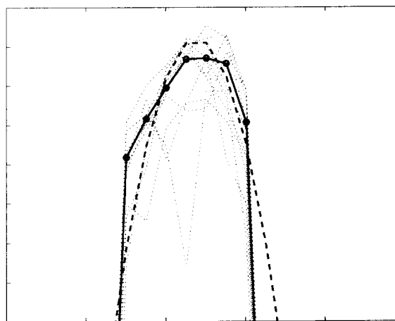
Fig. 10. Ripple surface. The dashed curve is the input rough surface. The solid curve is the inverted result based on results from Fig. 9.
