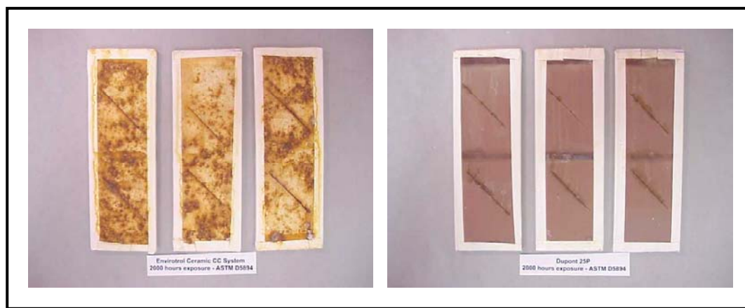
Figure 6. Comparison of (a) Envirotrol ceramic cover CC system coatings and (b) DuPont epoxy barrier coatings after 2000 hours of exposure in the ASTM D 5894.
