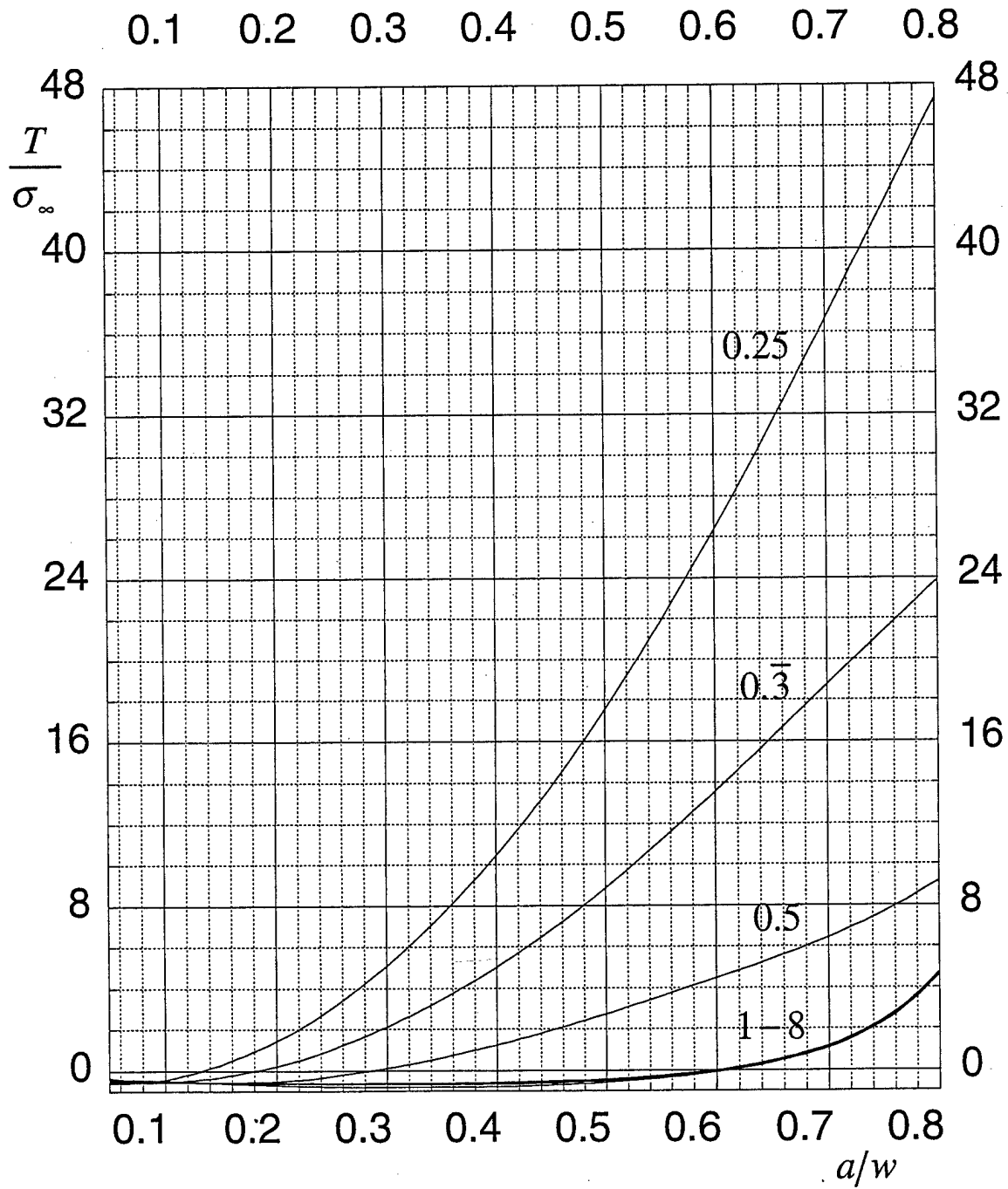
Normalized T-stress. Applied uniform load. Plane strain.
