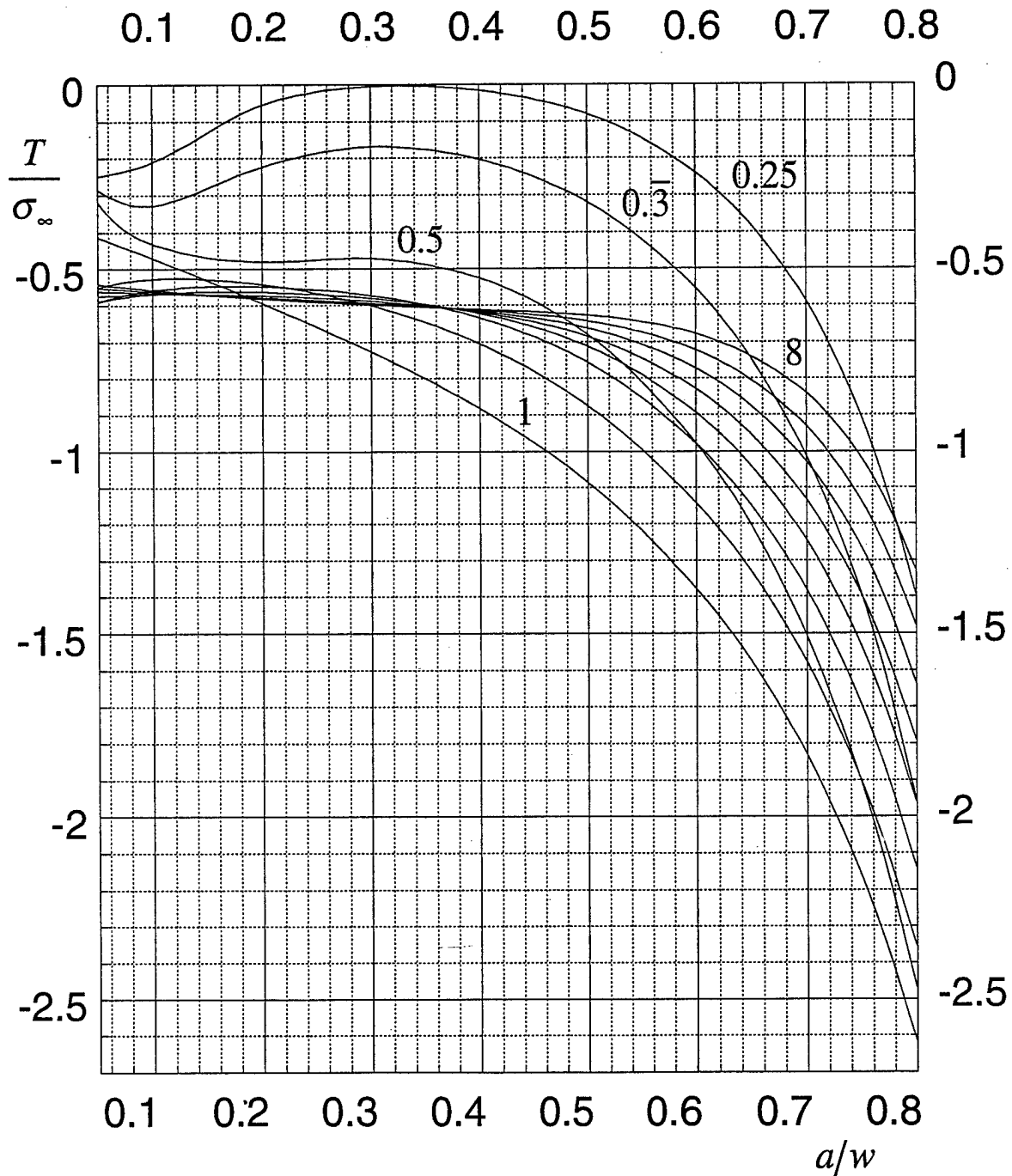
Normalized T-stress. Applied uniform displacement. Plane strain.
