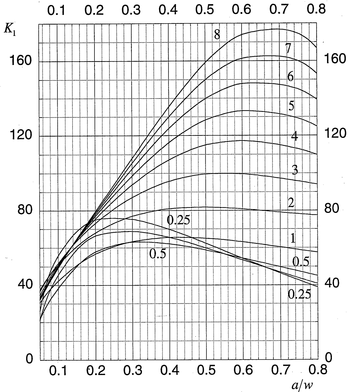
Stress intensity factor. Applied uniform displacement. Plane strain.
