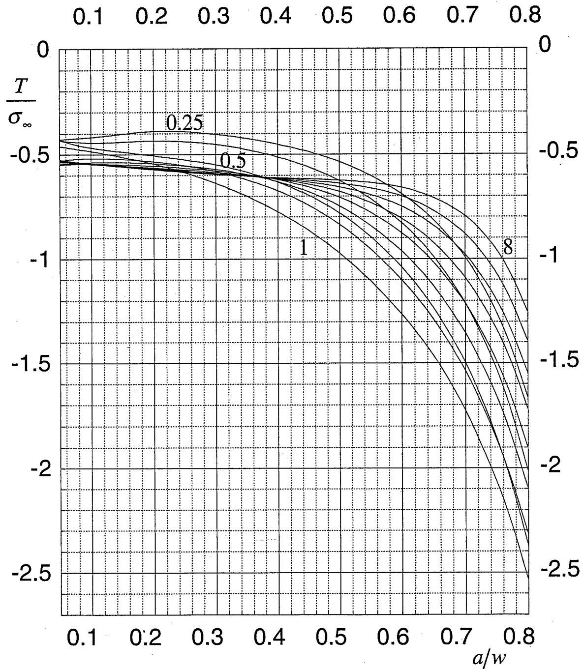
Normalized T-stress. Applied uniform displacement. Plane stress.
