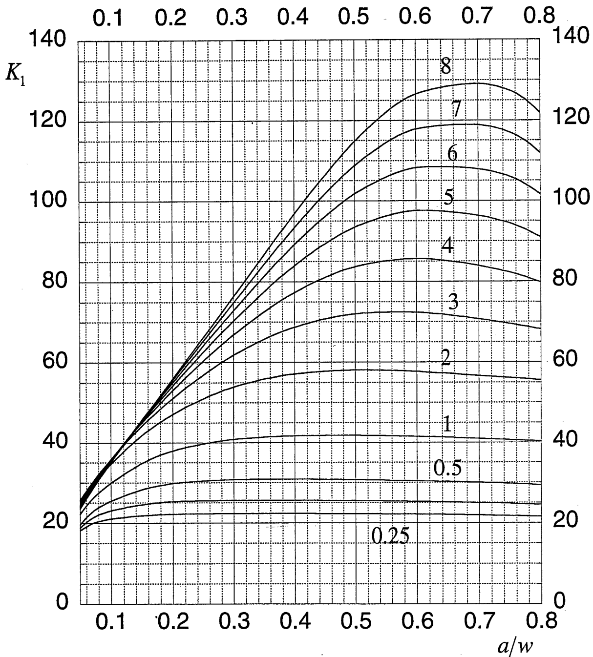
Stress intensity factor. Applied uniform displacement. Plane stress.
