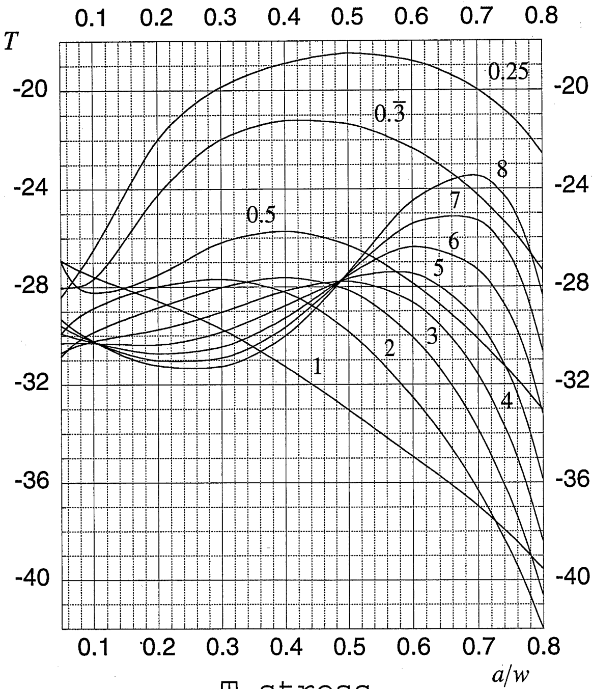
T-stress. Applied uniform displacement. Plane stress.
