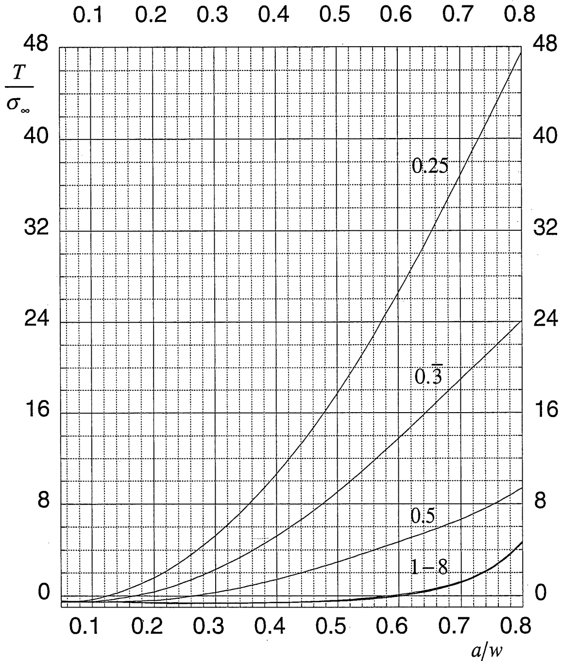
Normalized T-stress. Applied uniform load. Plane stress.
