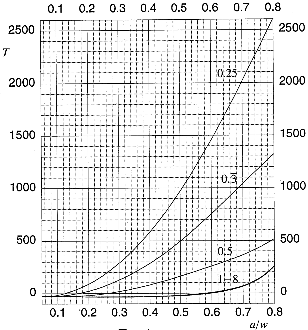
T-stress. Applied uniform load. Plane stress.
