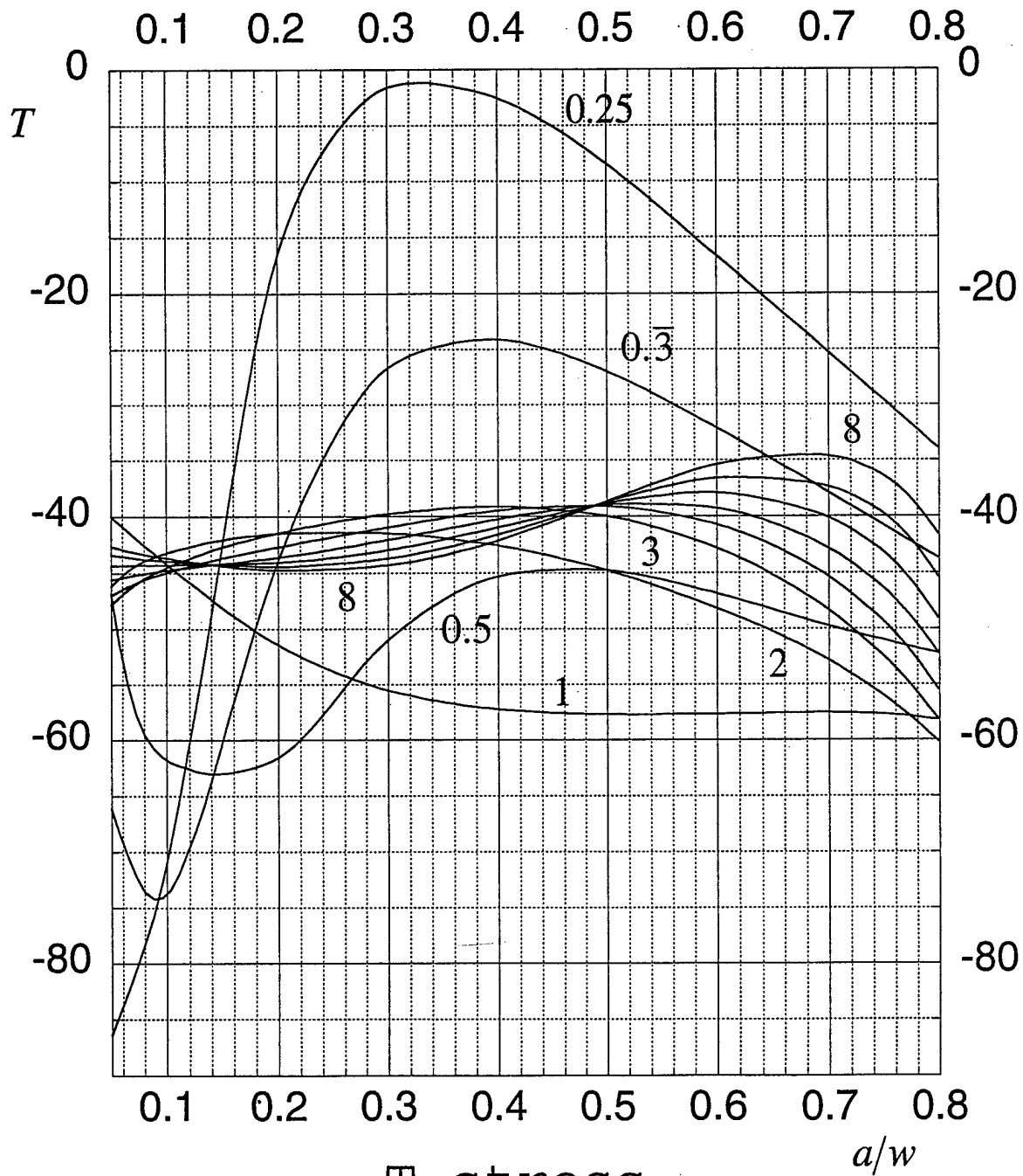
T-stress. Applied uniform displacement. Plane strain.
