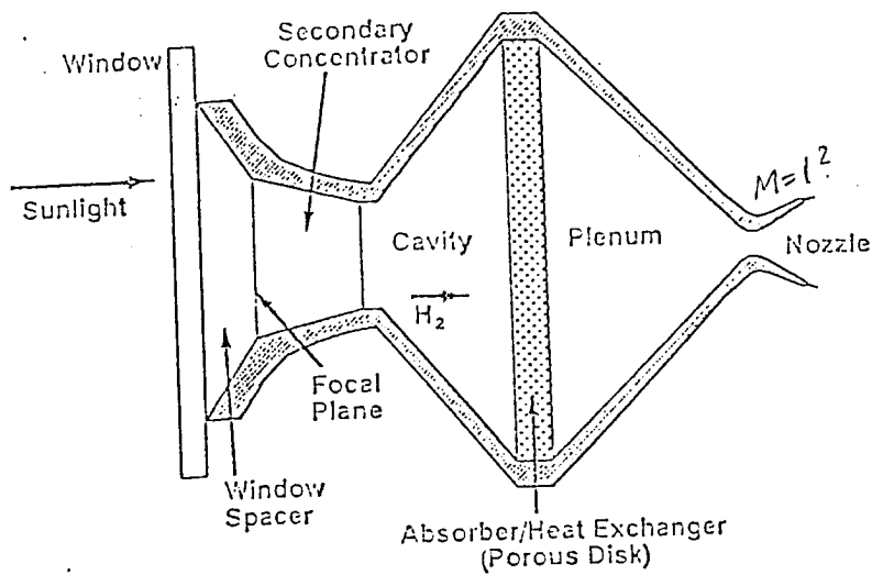
Figure 1: Schematic drawing of solar thruster model.
