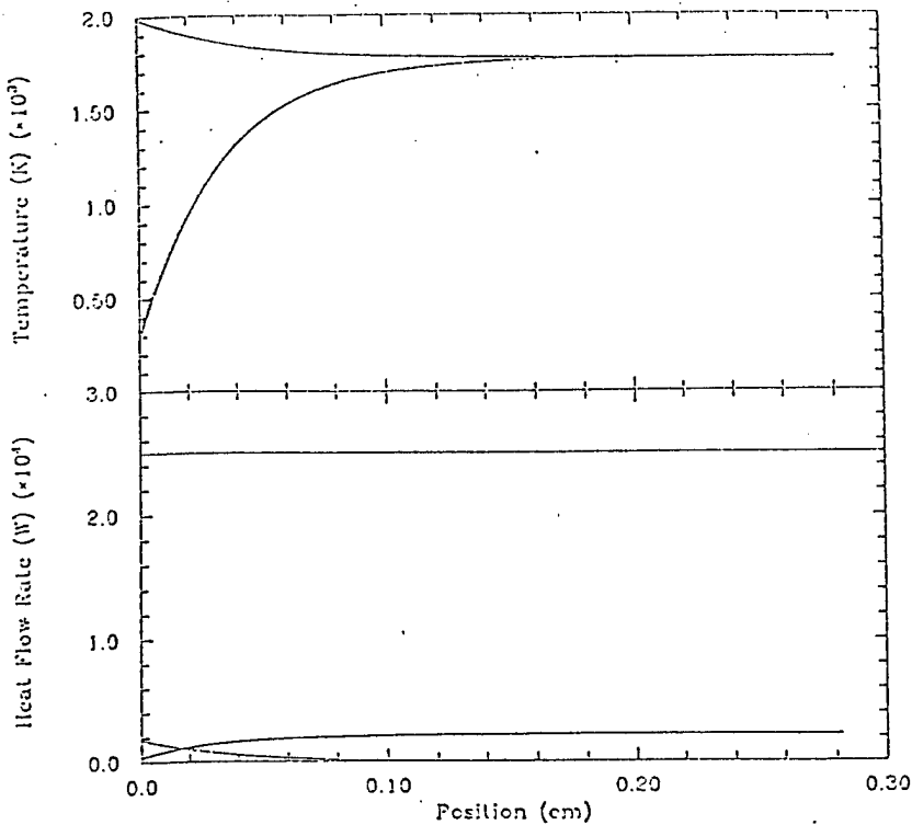
Figure 2: Propellant/Radiation temperatures and heat flow rates as a function of axial position. R_c = 650 . Power = 25 kW. \dot{m} = 0.1 \text{ gm/sec}
