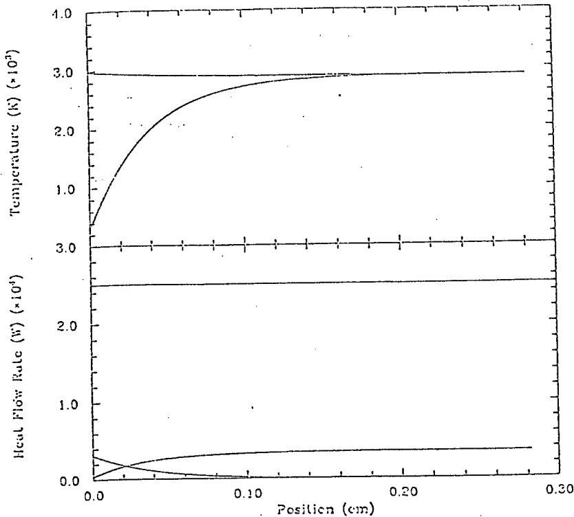
Figure 3: Propellant/Radiation temperatures and heat flow rates as a function of axial position. R_c = 3700 . Power = 25 \text{ kW} . \dot{m} = 0.1 \text{ gm/sec}
