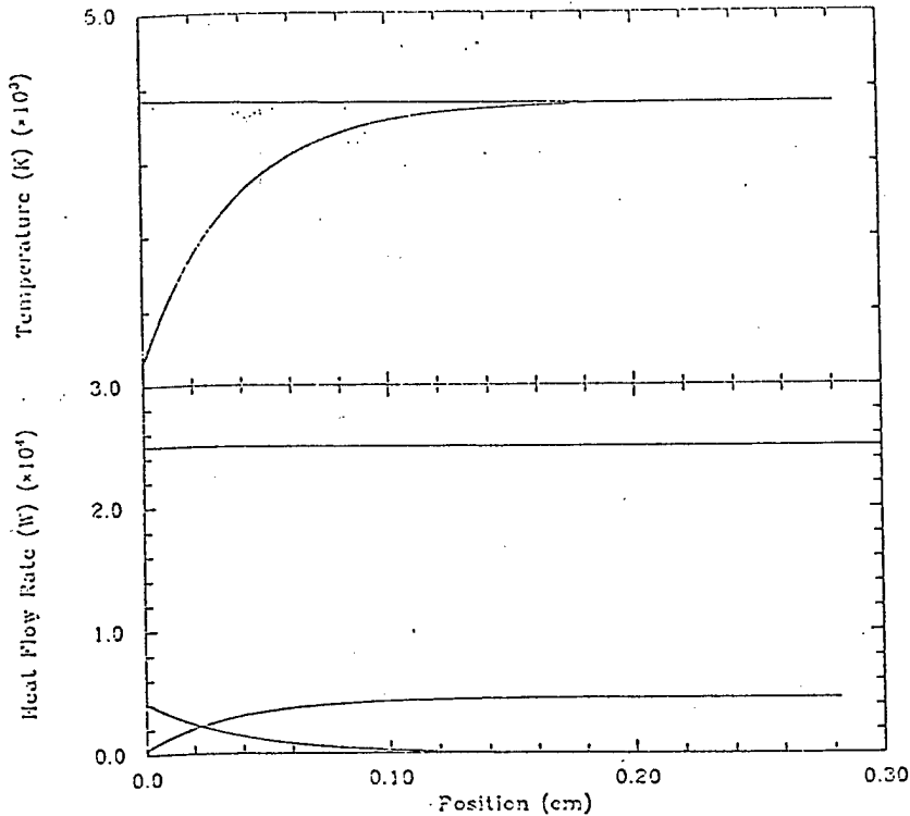
Figure 4: Propellant/Radiation temperatures and heat flow rates as a function of axial position. R_c = 11000 . Power = 25kW . \dot{m} = 0.1gm/sec
