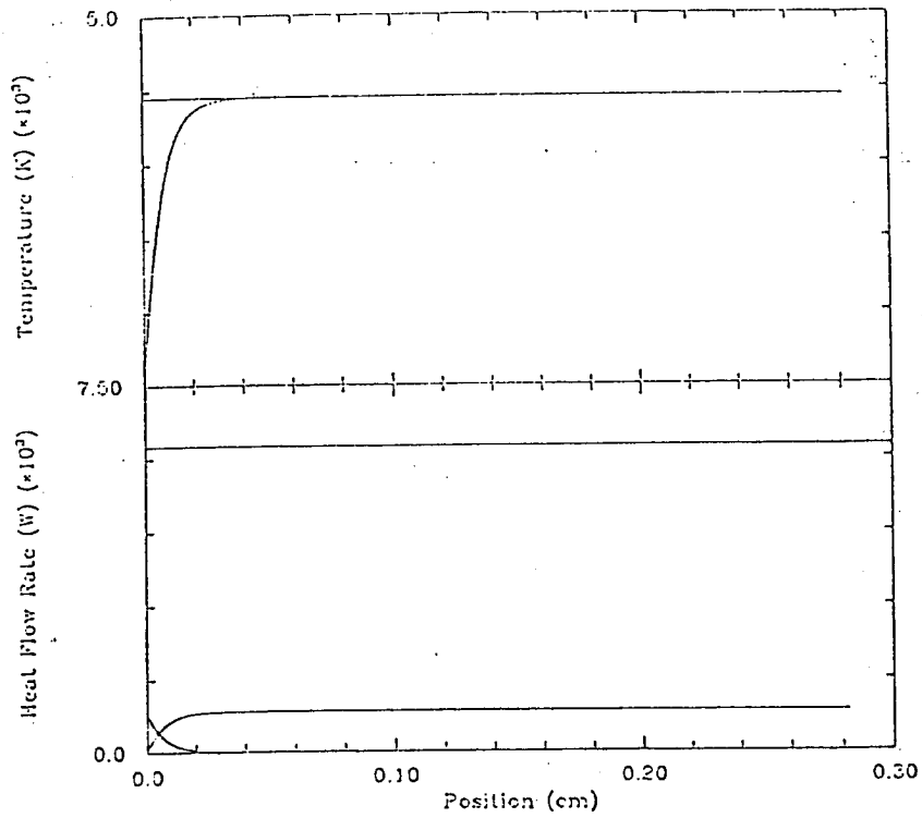
Figure 6: Propellant/Radiation temperatures and heat flow rates as a function of axial position. R_c = 11000 . Power = 6.25 \text{ kW} . \dot{m} = 0.025 \text{ gm/sec}
