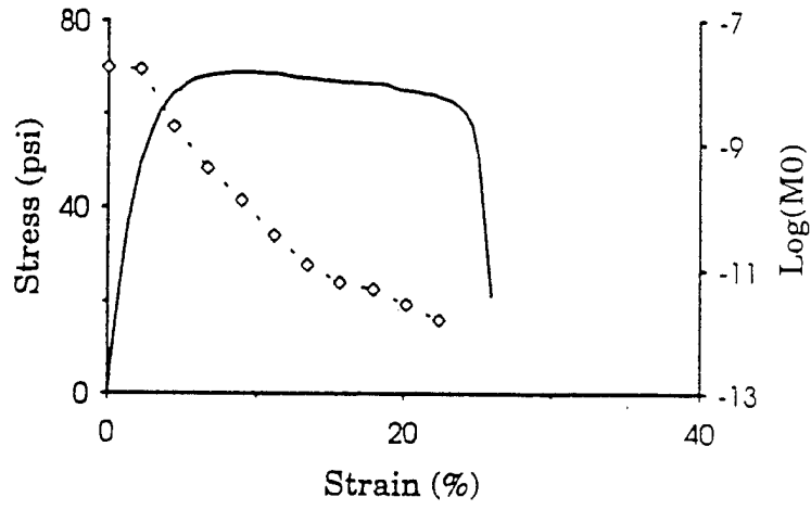
Fig. 6 Plot of stress and ultrasonic energy ( Mo ) as functions of strain ( constant strain rate loading )
