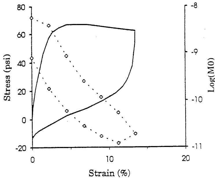
Fig. 7 Plot of stress and ultrasonic energy ( Mo ) as functions of strain ( cyclic loading )
