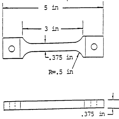
Fig.1 Specimen geometry
