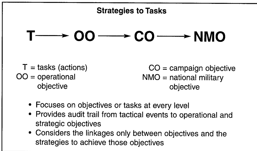
Figure 6. Objectives-Based Methodology
