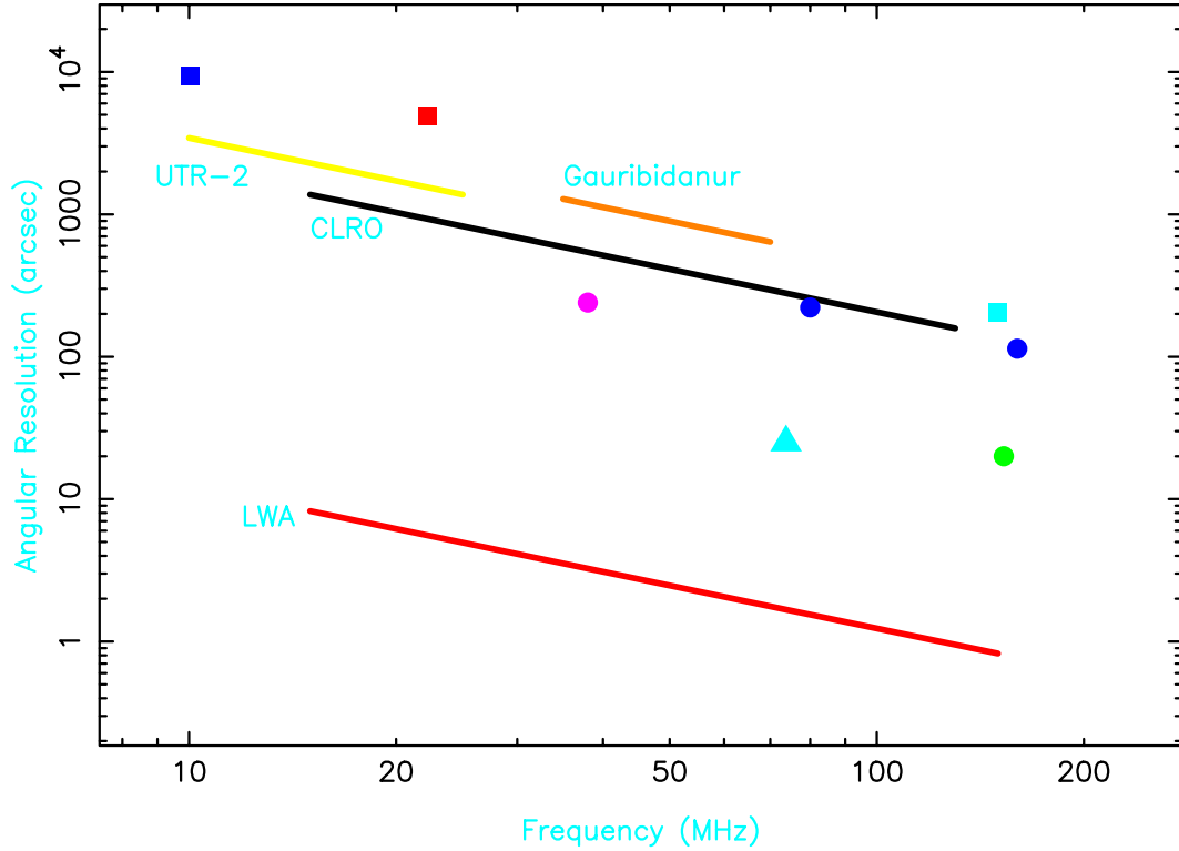
Fig. 4—Angular resolution (arcseconds) as a function of frequency (MHz) for past and present LW imaging instruments in the 10 to 200 MHz range. In addition to the broadband instruments labelled in the figure, various telescopes that operate or operated at “spot” frequencies are shown. These include the Giant Metrewave Radio Telescope (GMRT; green circle), Culgoora (blue circles); the 74 MHz VLA (cyan triangle); Cambridge Polar Cap survey (pink circle); the Dominion Radio Astronomy Observatory at 10 MHz (blue square) and at 22 MHz (red square); and the Mauritius Radio Telescope (cyan square). The LWA will result in a dramatic improvement in angular resolution and frequency coverage.
