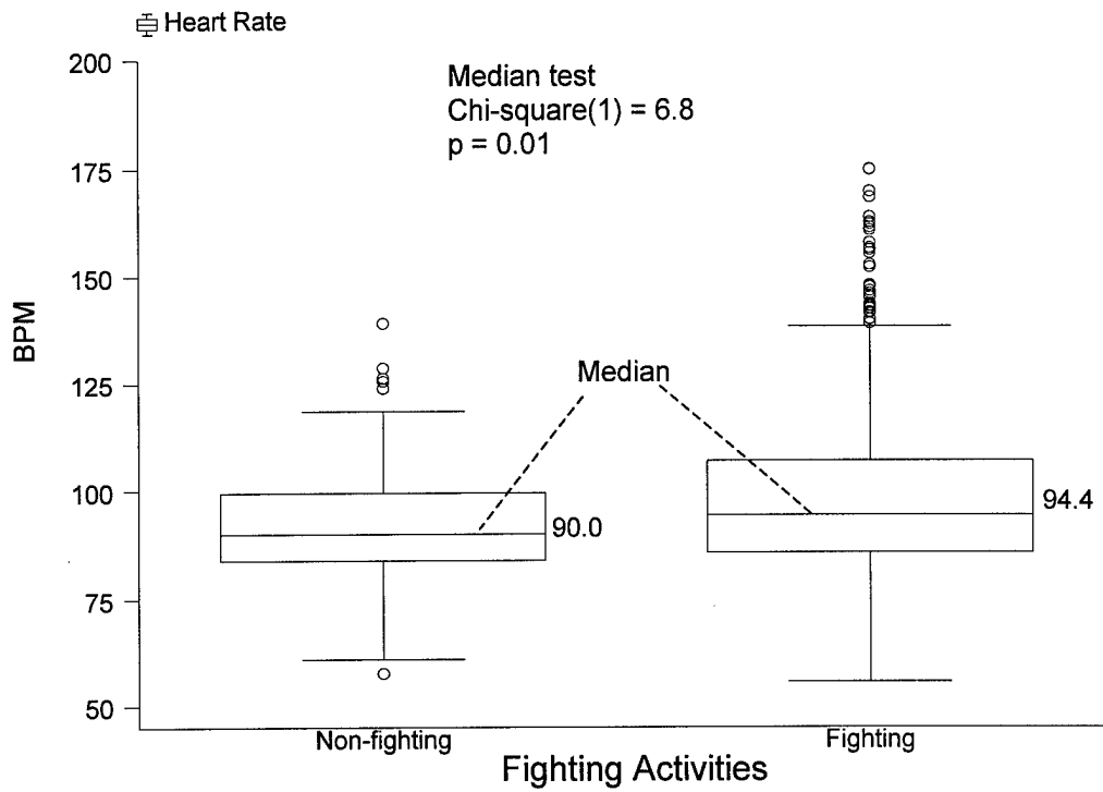
Figure 4. Median heart rate comparison between fighting and non-fighting activities
