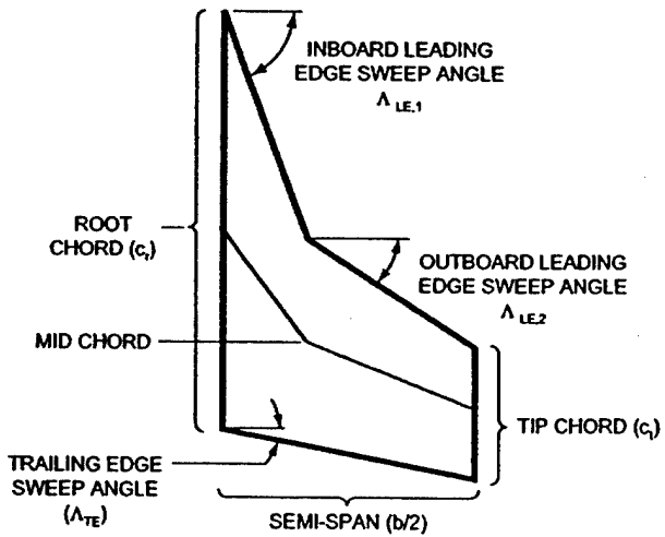
Figure 2. Wing Parameters.
