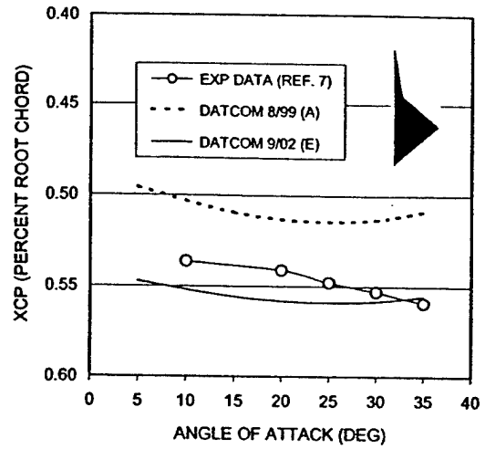
Figure 9. Wing x_{cp} Versus Angle of Attack, Configuration 16, Mach = 0.14.
