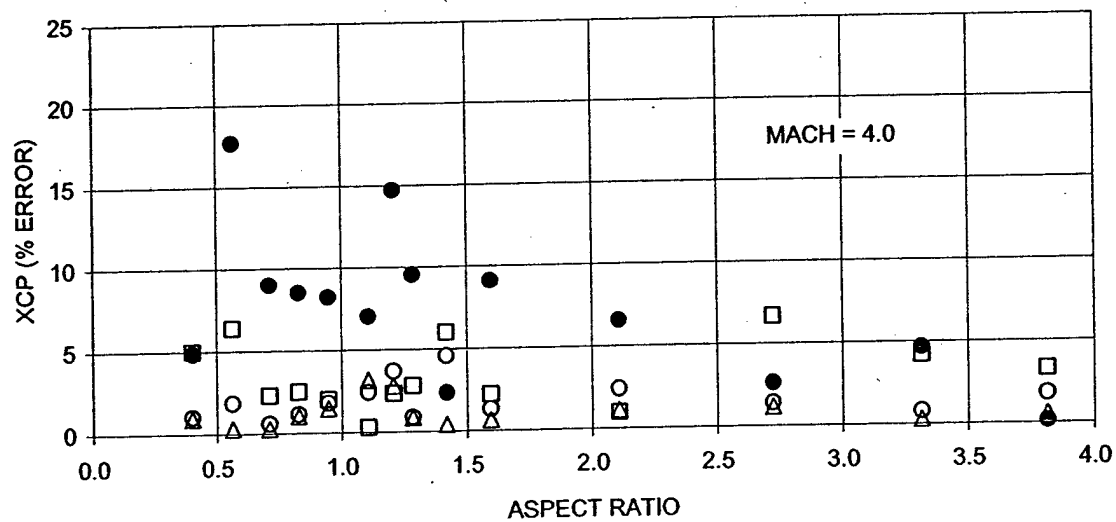
Figure 5. Analytical Error Versus Aspect Ratio.
