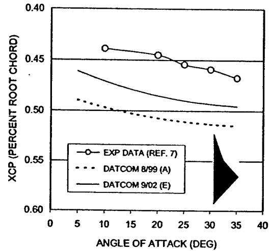
Figure 10. Wing x_{cp} Versus Angle of Attack, Configuration 17, Mach = 0.14.
