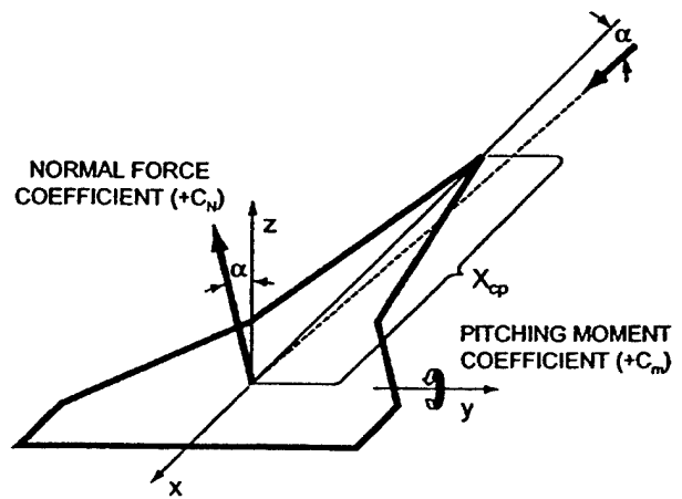
Figure 4. Sign Conventions.
