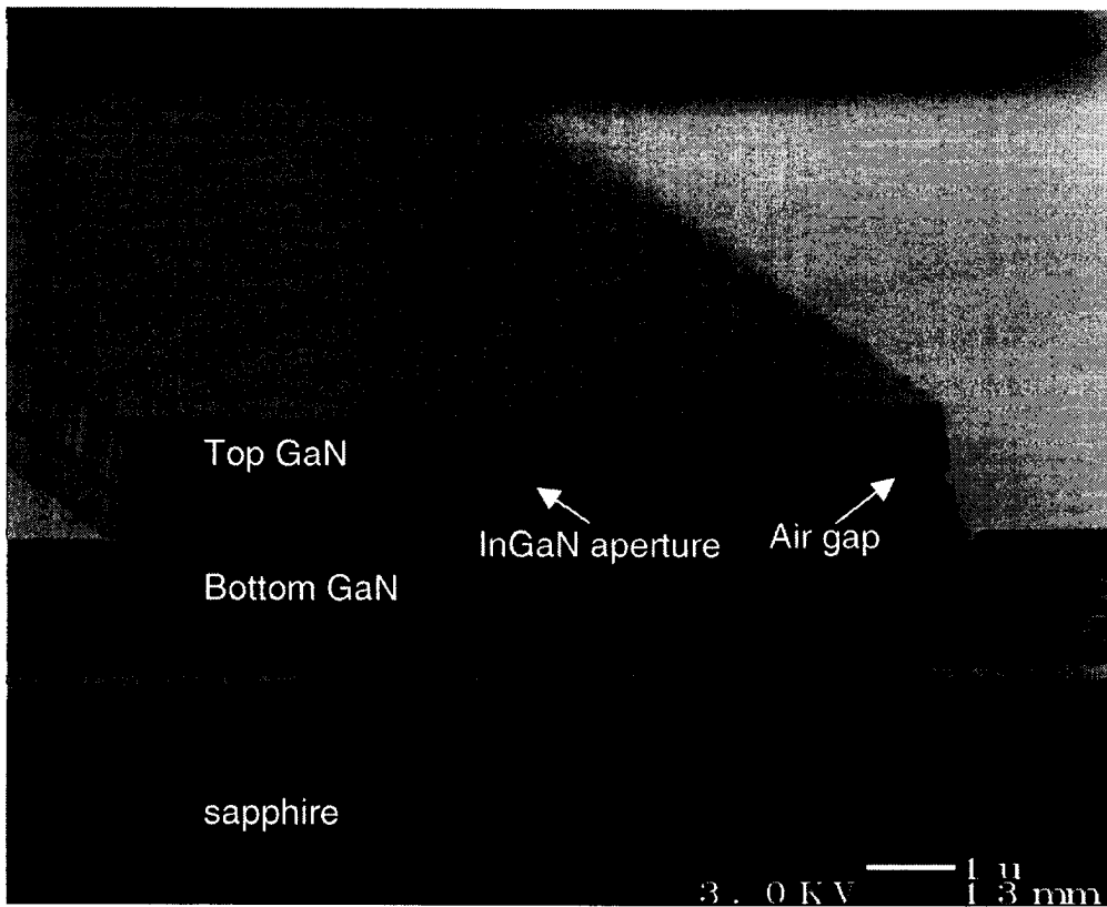
Fig 6. Highly controllable aperture formed by lateral etching \text{In}_x\text{Ga}_{1-x}\text{N} ( x \sim 8\% , 600 \text{ \AA} thick) sacrificial layer from each side.
