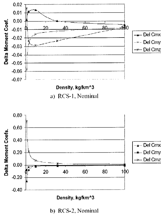
FIG 4. Increments in aerodynamic moments produced by various thruster firings. Spacecraft attitude at zero pitch and yaw.
