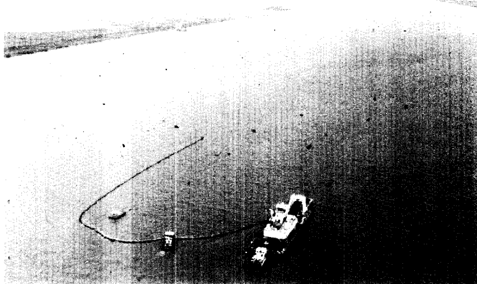
Figure 1. Dredge Beachbuilder with tug astern and its floating, flexible hose configuration restoring marshland at Head of Passes. The beginning of the shore pipeline is located in the upper left-hand side of the picture by the barge-mounted crane
