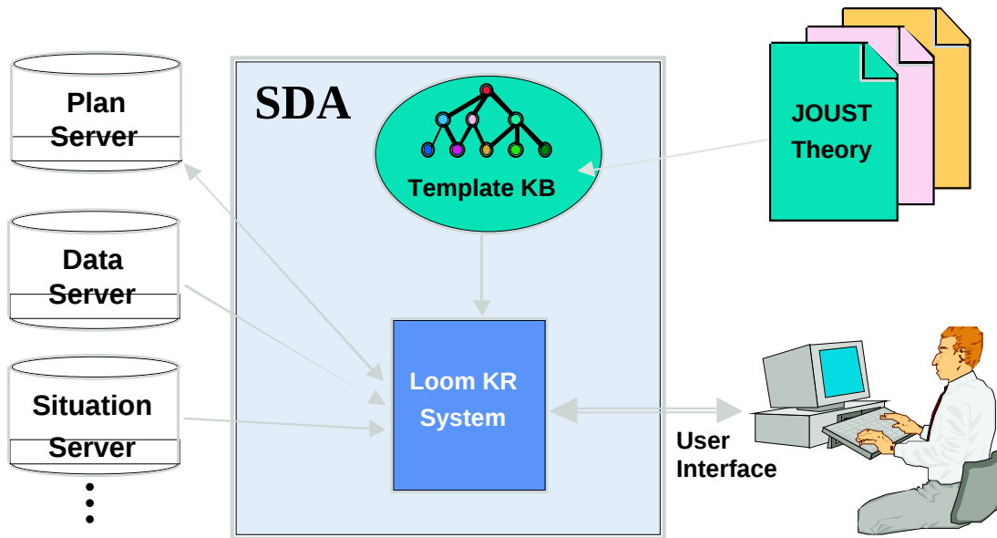
Figure 3.1: SDA Software Architecture
