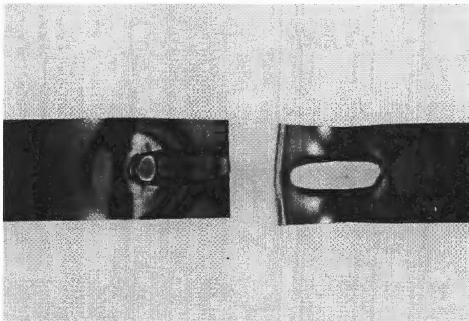
Figure 32. Typical failure of a plug weld peel specimen welded under improved conditions. Failure occurred by metal tearing initiated within the heat-affected zone; magnified 1 \times .
