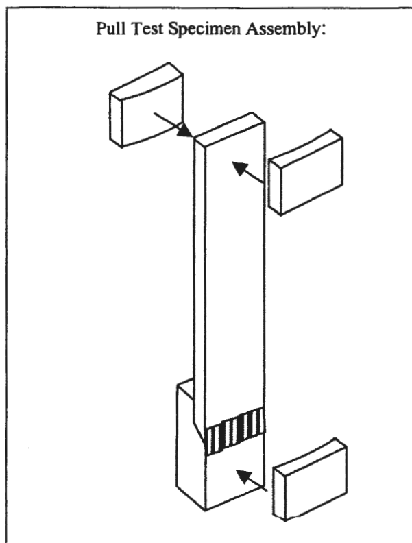
Figure H-8. Pull test assembly for fillet specimen.
