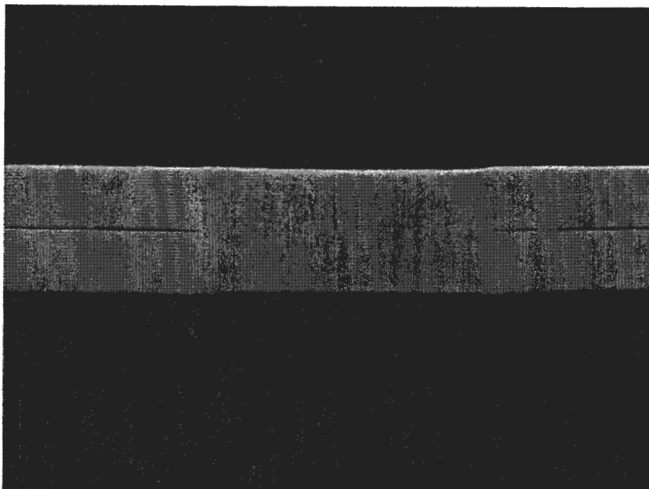
Figure 29. Macrograph of a typical improved spot weld tensile shear specimen; magnified 9 \times , etchant: 1% nital.
