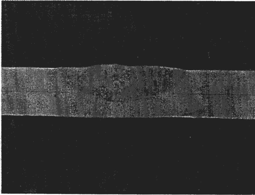
Figure 28. Macrograph of a plug weld peel specimen welded using improved conditions by Aerotek; magnified 9 \times , etchant: 1% nital.
