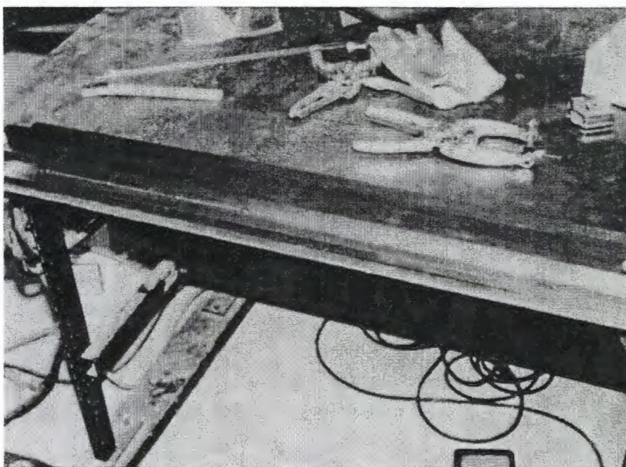
Figure 12. Photograph showing as-welded fillet weld assembly, from a different angle, at Aerotek.
