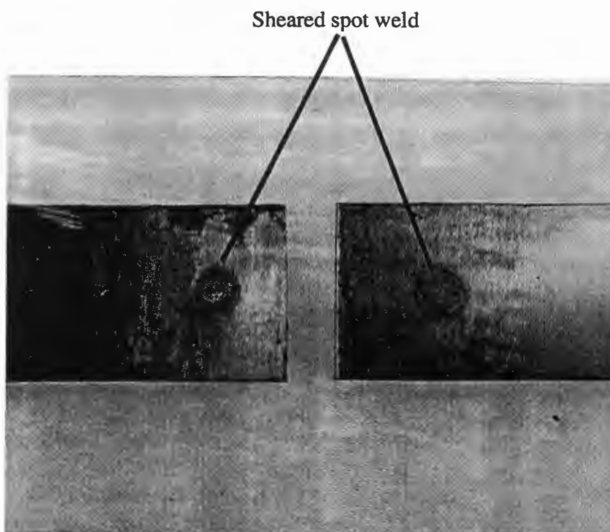
Figure 23. A typical spot weld shear failure; magnified 1×.
