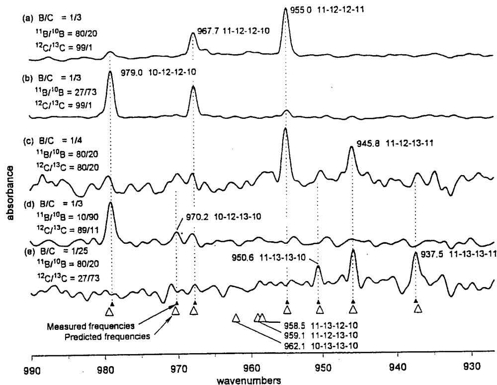
FIG. 3. FTIR spectra of the \nu_3(\nu_n) mode of isotomers of linear BCCB. The spectra were recorded after annealing the matrices with the indicated compositions at 27.5 K for 150 s. The large open triangles at the bottom show the predicted frequencies of linear BCCB isotomers (as explained in the text) and small filled triangles show measured isotomer frequencies.
