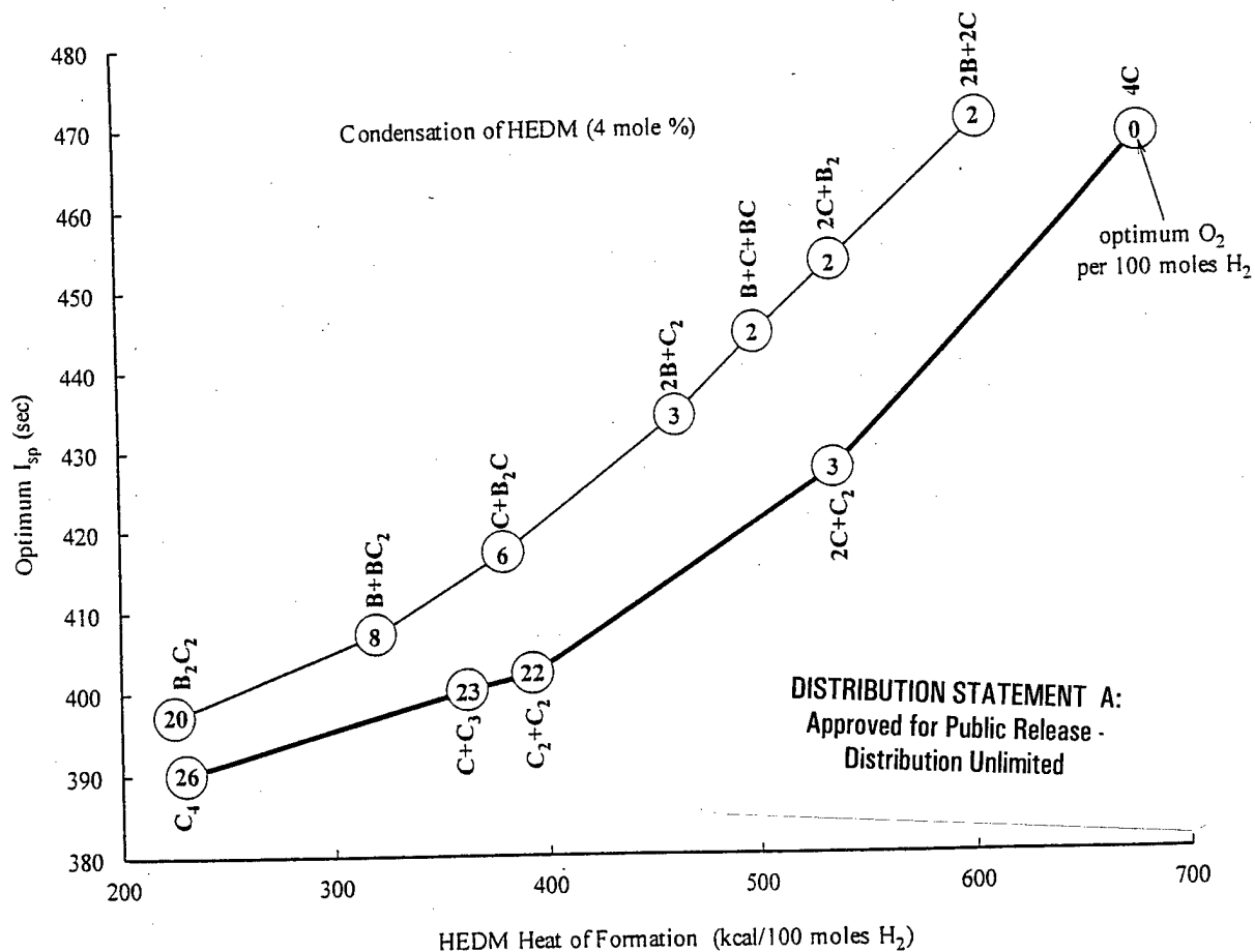
Figure 1. Specific impulse of HEDM containing 4 mole percent equivalent atom density in solid hydrogen with various stages of condensation. Numbers inside circles denote the optimum moles of O_2 per 100 moles of H_2 that produces the maximum I_{sp} for the indicated compositions. The calculations are based on the standard rocket operating conditions, 1000 psi combustion pressure and 1 atm nozzle exit pressure, which produce 389 sec with liquid oxygen/liquid hydrogen propellant. The propellant composed of 4 mole percent C-atoms produces maximum I_{sp} with no oxygen. If the atoms condense to 1 mole percent C_4 , the I_{sp} drops to the baseline 389 sec value.
