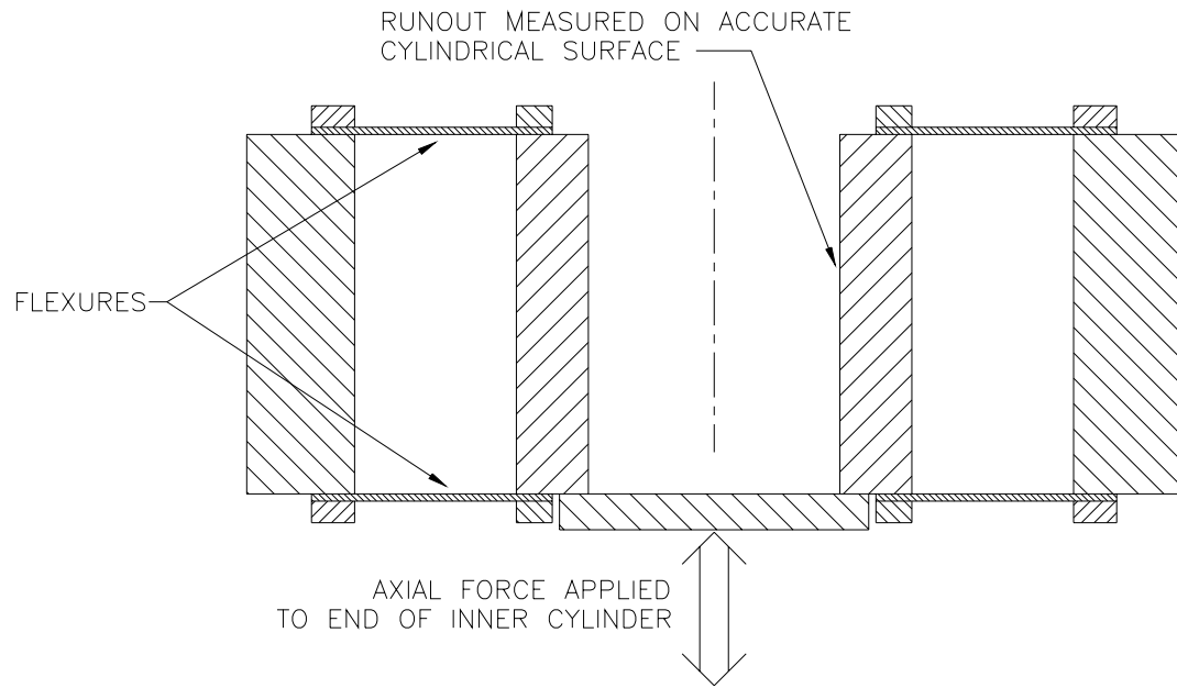
Figure 5. Test Assembly
