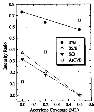
FIG. 3. Intensity ratios of the surface components ( S , SS , and S' ) to the bulk component ( B ) of the Si 2 p core-level spectra for different acetylene coverage. The S / B and SS / B data points predict an ideal homogeneous adsorption mode.
