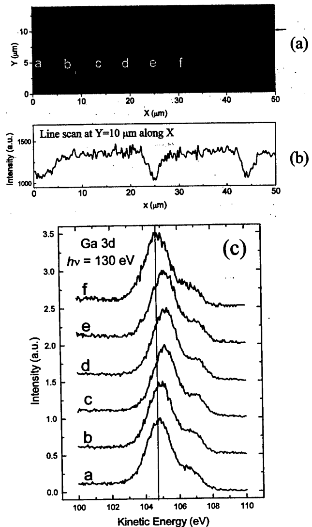
FIG. 7. (a) Photoemission spectromicroscopy image of a 50 \times 15\ \mu\text{m}^2 area of the ELO GaN surface (sample M287) with a 10\ \text{ML} equivalent Mg deposition. (b) Line profile obtained from the above image at the position marked by the arrow. (c) Microprobe Ga 3d EDCs collected at the positions from (a)–(f) noted in the image. All the curves have different energy positions that have no apparent relationship to the growth stripes on the film.
