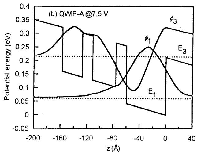
Figure 2. The calculated envelope wavefunctions of QWIP-A (a) under zero bias and (b) V_b = 7.5 V.
