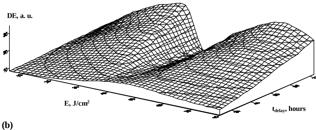
Fig. 14. The hologram diffraction efficiency for SD DG doped by KCl in the gelatination time dependence at temperature 24°C (a) and at temperature 0°C (b).
