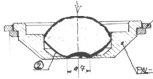
Fig. 8 Position of PAL forming the foveal aperture
