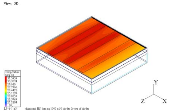
Figure 9. Heated Surface Temperature Profiles for Triple Diode Bar on Diamond, Ethylene Glycol/Water Coolant
