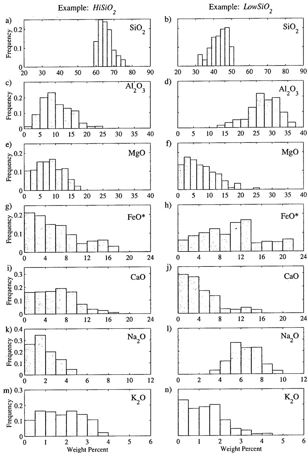
Figure 6-12: Frequency distributions of the major element oxides for examples, HiSiO 2 and LowSiO 2 . Distributions are calculated from the synthetic data by simultaneously constraining V_p and \text{SiO}_2 content. In both cases, V_p is constrained using the average crustal velocity between 20 and 40 km from Christensen and Mooney [1995], while \text{SiO}_2 content is limited to be > 60\% for HiSiO 2 and < 50\% for LowSiO 2 .
