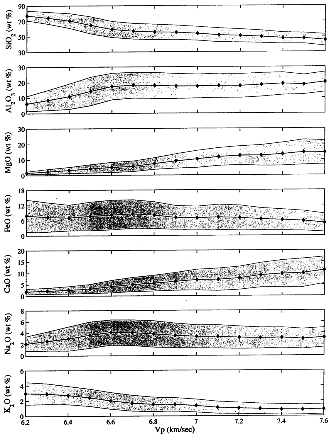
Figure 6-9: Composition bounds for major element oxides as a function of V_p for a depth of 35 km along a normal crustal geotherm. Mean oxide values are denoted by solid diamonds and grey fields represent 1\sigma variation around the mean. Values are taken from Table A.1.
