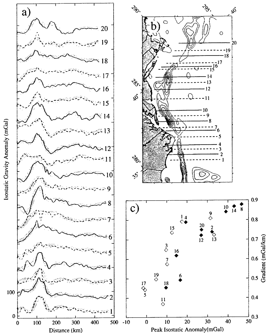
Figure 2-14: (a) Across-margin profiles showing variations in the isostatic gravity anomaly. Solid lines represent profiles taken through 100–150 km wavelength peaks in the isostatic gravity anomaly, while dashed lines show profiles taken through 100–150 km wavelength isostatic lows. Thick shaded lines represent the filtered isostatic anomaly calculated using a cosine cutoff taper to remove wavelengths < 50 –100 km. (b) Location of profiles shown in Figure 2-14a. Shaded contours illustrate filtered isostatic gravity anomalies greater than 0 mGal with a contour interval of 10 mGal. (c) Mean absolute gradient in across-margin anomaly versus the peak value of the isostatic gravity anomaly. The mean absolute gradient was calculated along an across-margin profile in a 200 km window around the peak value of the isostatic anomaly. Solid symbols represent across-margin profiles taken through 100–150 km wavelength isostatic highs, while open symbols represent across-margin profiles taken through isostatic lows. Note the positive relationship between the mean absolute across-margin gradient and the peak of the isostatic anomaly, indicating that as the peak of the isostatic anomaly decreases, the overall across-margin variation becomes smaller.
