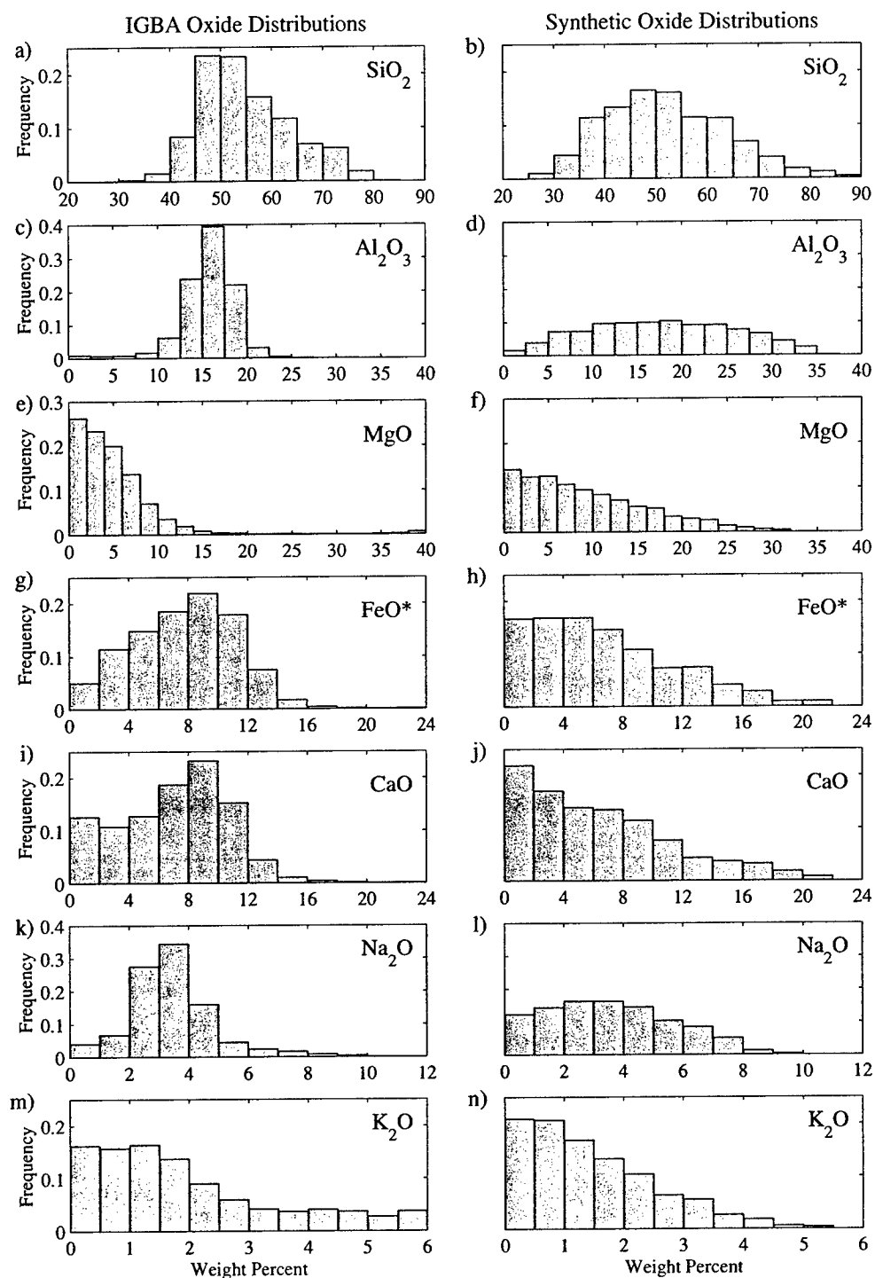
Figure 6-3: Observed frequency distributions for major oxides in IGBA database, a) SiO 2 , c) Al 2 O 3 , e) MgO, g) FeO*, i) CaO, k) Na 2 O, m) K 2 O, and calculated frequency distributions for synthetic compositions, b) SiO 2 , d) Al 2 O 3 , f) MgO, h) FeO*, j) CaO, l) Na 2 O, n) K 2 O. Note that synthetic oxide distributions are much broader than IGBA distributions.
