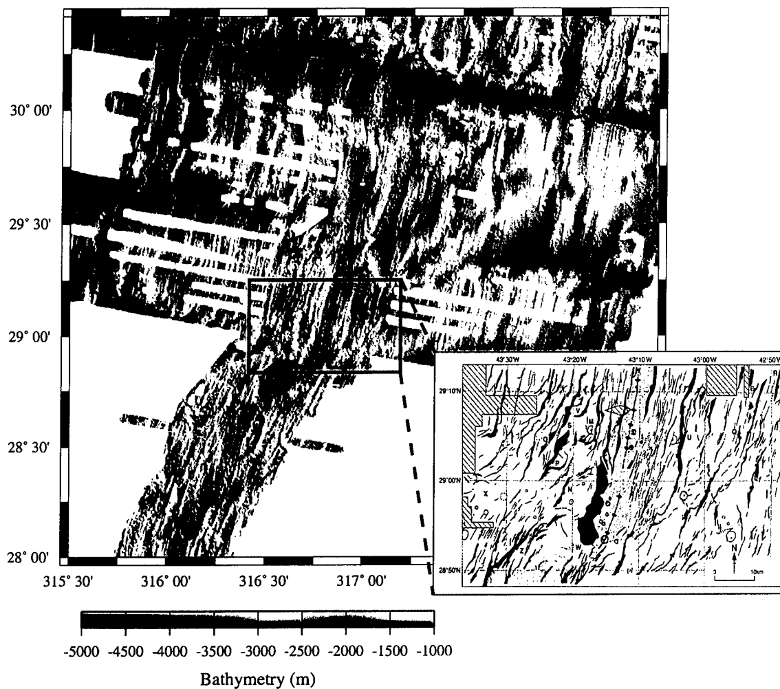
Figure 5-2: Sea Beam bathymetry map of the Mid-Atlantic Ridge south of the Atlantis Fracture Zone. Data from Purdy et al. [1990] and Sempéré et al. [1995]. Inset shows the geologic interpretation of the Broken Spur segment by Searle et al. [1998] based on bathymetry and TOBI sidescan images. Major fault scarps are shown in black. Inset from Searle et al. [1998].
