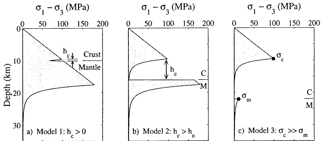
Figure 3-10: Three potential models to explain the transition from mantle-dominated to crust-dominated deformation in Figs. 3-6 and 3-9. (a) Model 1: Requires only the presence of a ductile lower crustal channel, with thickness h_c > 0 [Shaw and Lin, 1996]. (b) Model 2: Requires the thickness of the lower crustal channel to be greater than a critical value ( h_c > h_o ), which represents the length scale over which stresses can be transmitted through the channel. (c) Model 3: Requires stress accumulation in the crust ( \sigma_c ) to be much greater than the stress accumulation in the mantle ( \sigma_m ). The results of this study favor Model 3 for typical geologic conditions.
