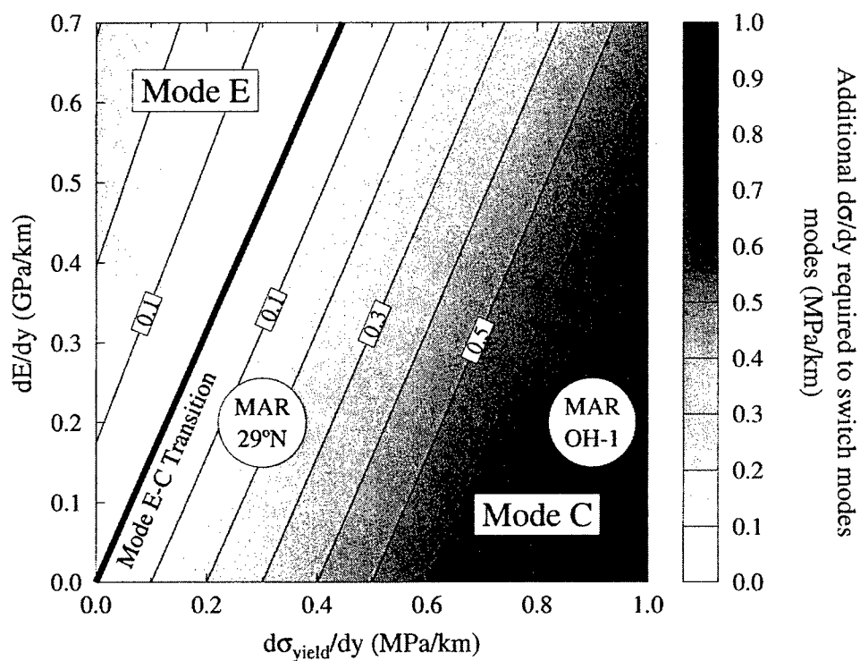
Figure 4-11: Contour plot of the additional gradient in \sigma_{\text{eff}} , after accounting for variations due to dE/dy , that is necessary to switch modes of faulting. Approximate parameter values of the OH-1 and MAR 29°N segments are shown based on the values of dE/dy and d\sigma_{\text{yield}}/dy calculated in Figure 4-4. We hypothesize that the additional gradient in \sigma_{\text{eff}} necessary to form the Model E faults observed at the OH-1 and MAR 29°N segments may be generated by a combination of shearing along transform faults and temporal variations in magma supply along the ridge axis.
