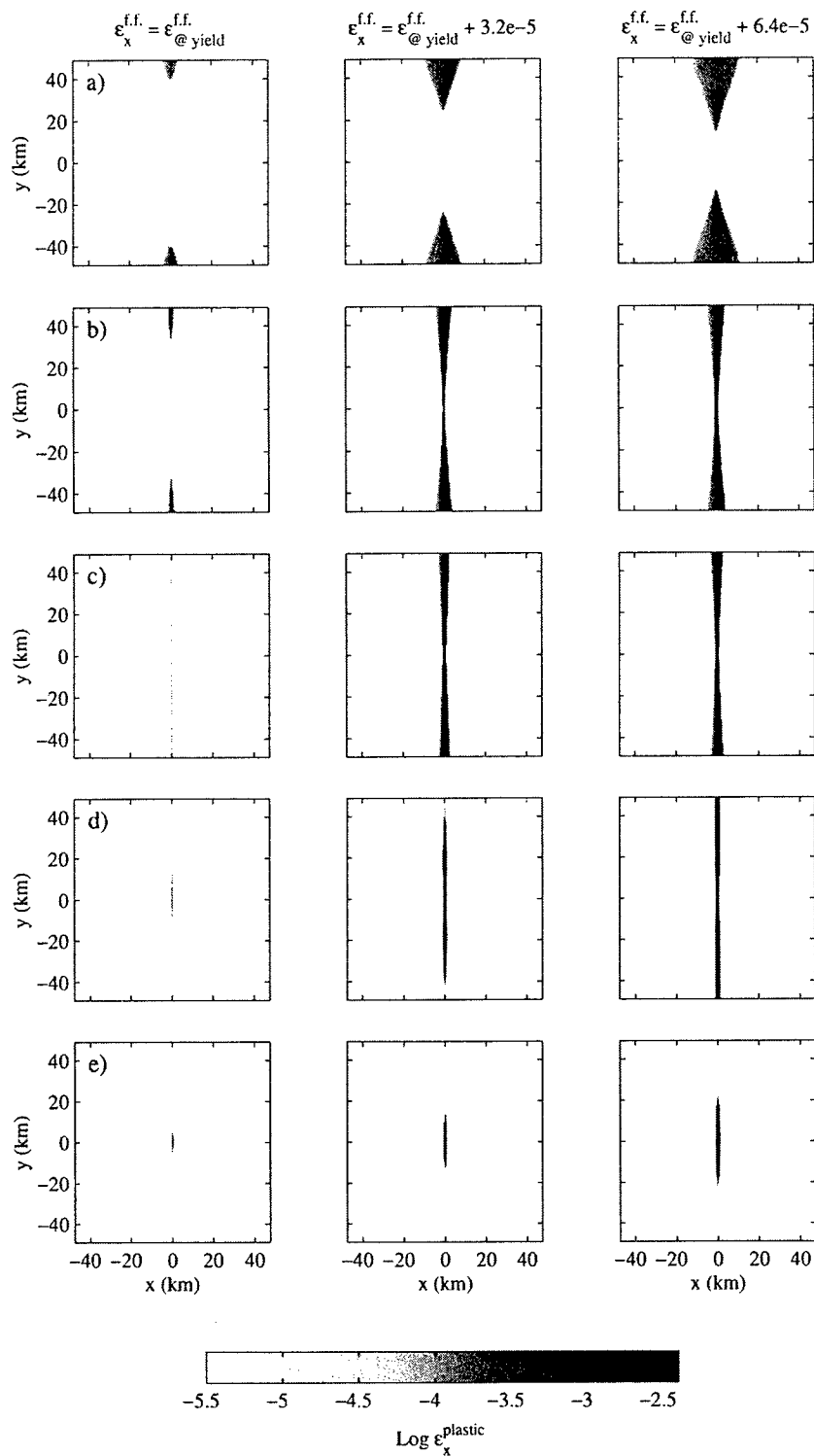
Figure 4-9: Plastic strain calculated using ADINA with increasing far-field strain for the 5 sets of parameters illustrated in Figure 4-8. (a,b) Mode E faults. (c) Uniform failure along the entire segment. (d,e) Mode C faults. For a given \epsilon_x^{f.f.} , the plastic deformation zone propagates a greater distance along-axis for the parameters in 4-9b and 4-9d than in 4-9a and 4-9e.
