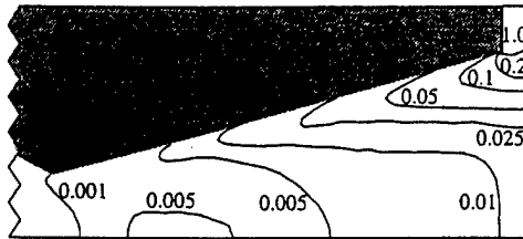
Fig. 8 Breakdown parameter (10 atm chamber pressure, SMILE)
