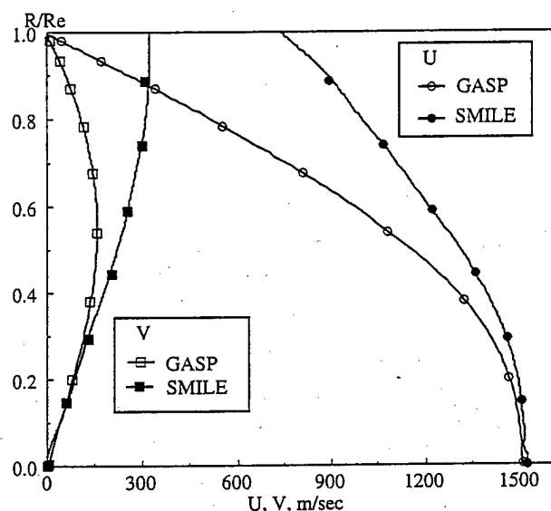
Fig. 14 Axial U and radial V velocity profiles at nozzle exit plane (1 atm chamber pressure)
